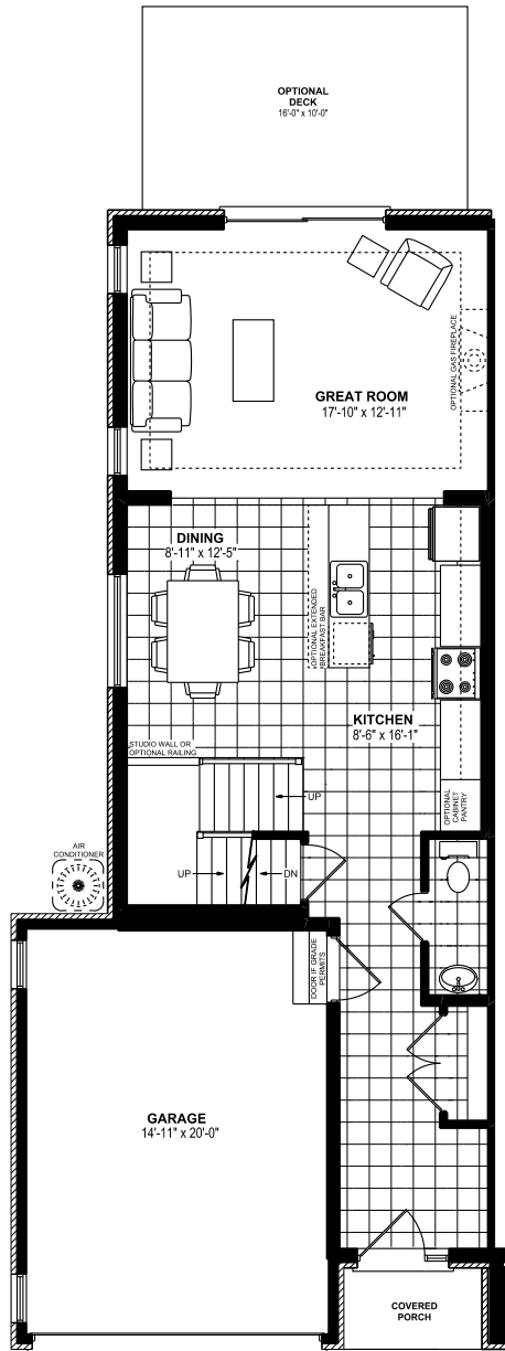
MAIN FLOOR - 811 SQ. FT.
