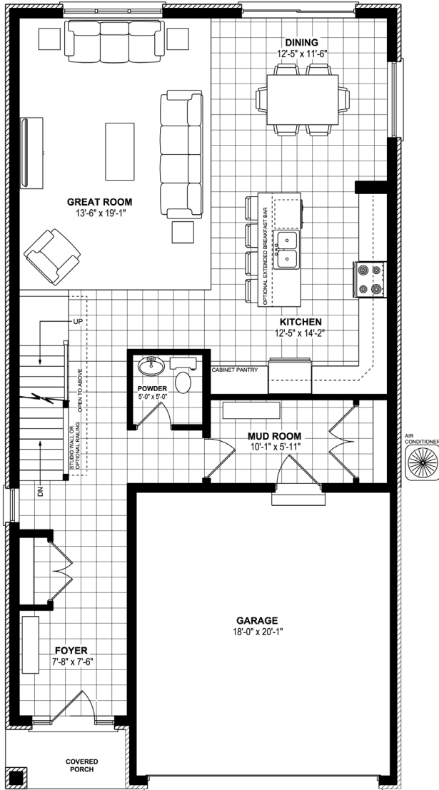
MAIN FLOOR - 1100 SQ. FT.
