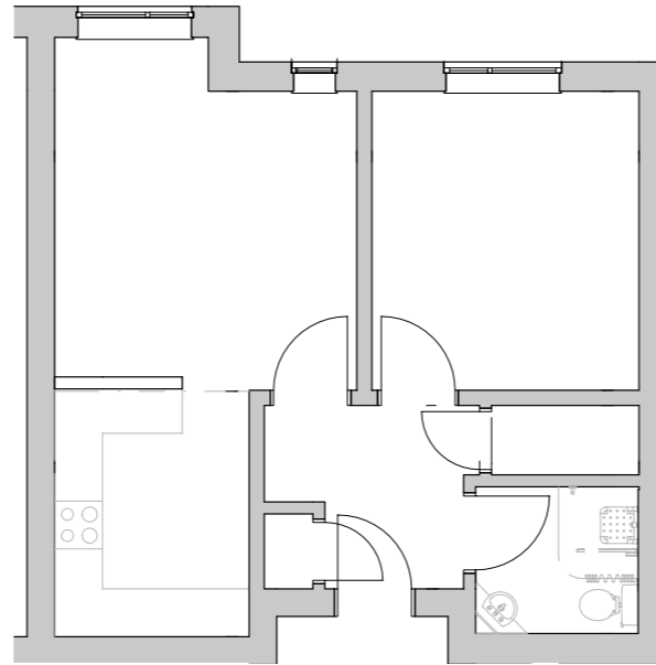
Apartment type A4
