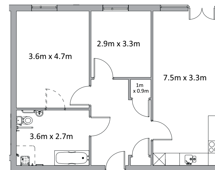
Apartment type H
