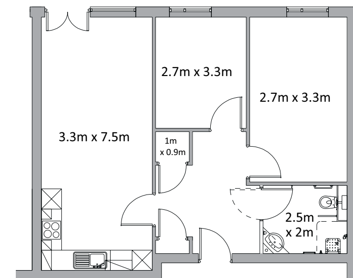
Apartment type D
