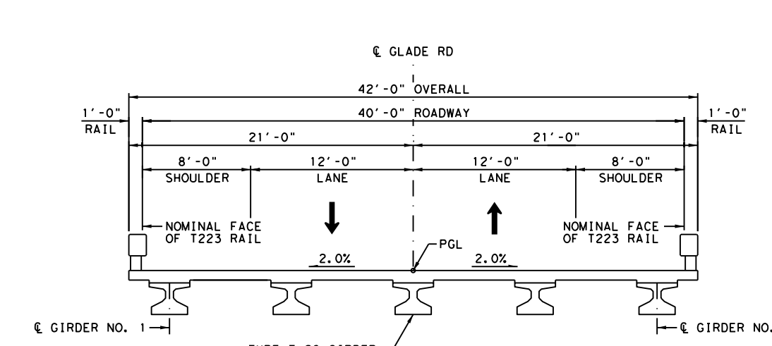
BRIDGE TYPICAL SECTION
