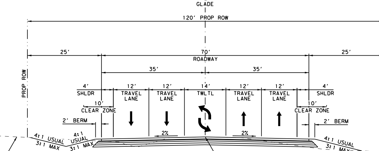
PROPOSED GLADE ROAD TYPICAL SECTION
