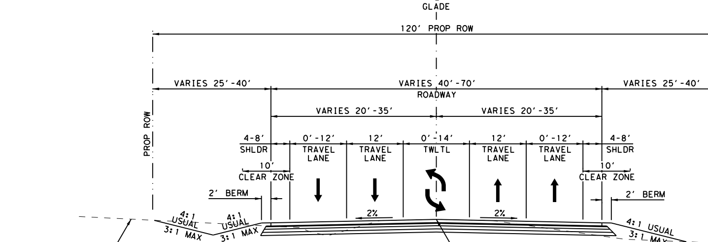
PROPOSED GLADE ROAD TYPICAL SECTION
