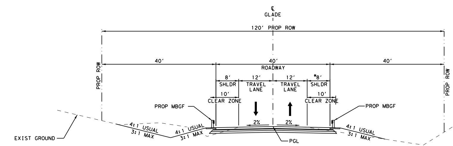
PROPOSED GLADE ROAD TYPICAL SECTION
