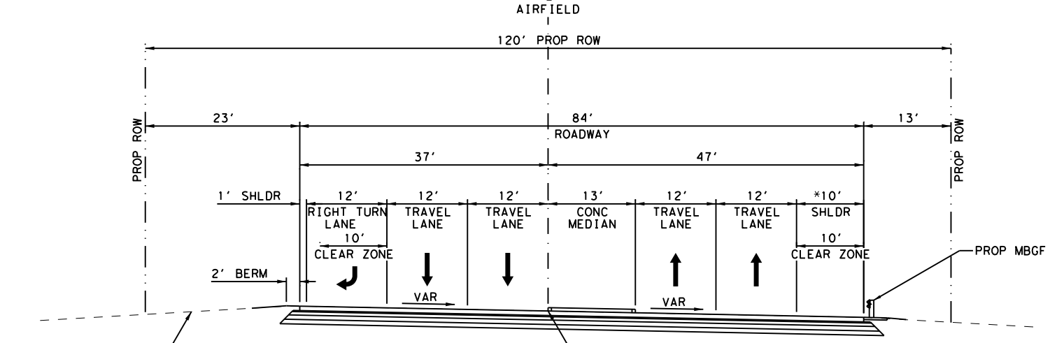
PROPOSED AIRFIELD DRIVE TYPICAL SECTION
