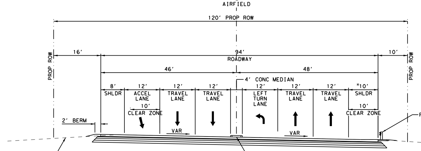
PROPOSED AIRFIELD DRIVE TYPICAL SECTION
