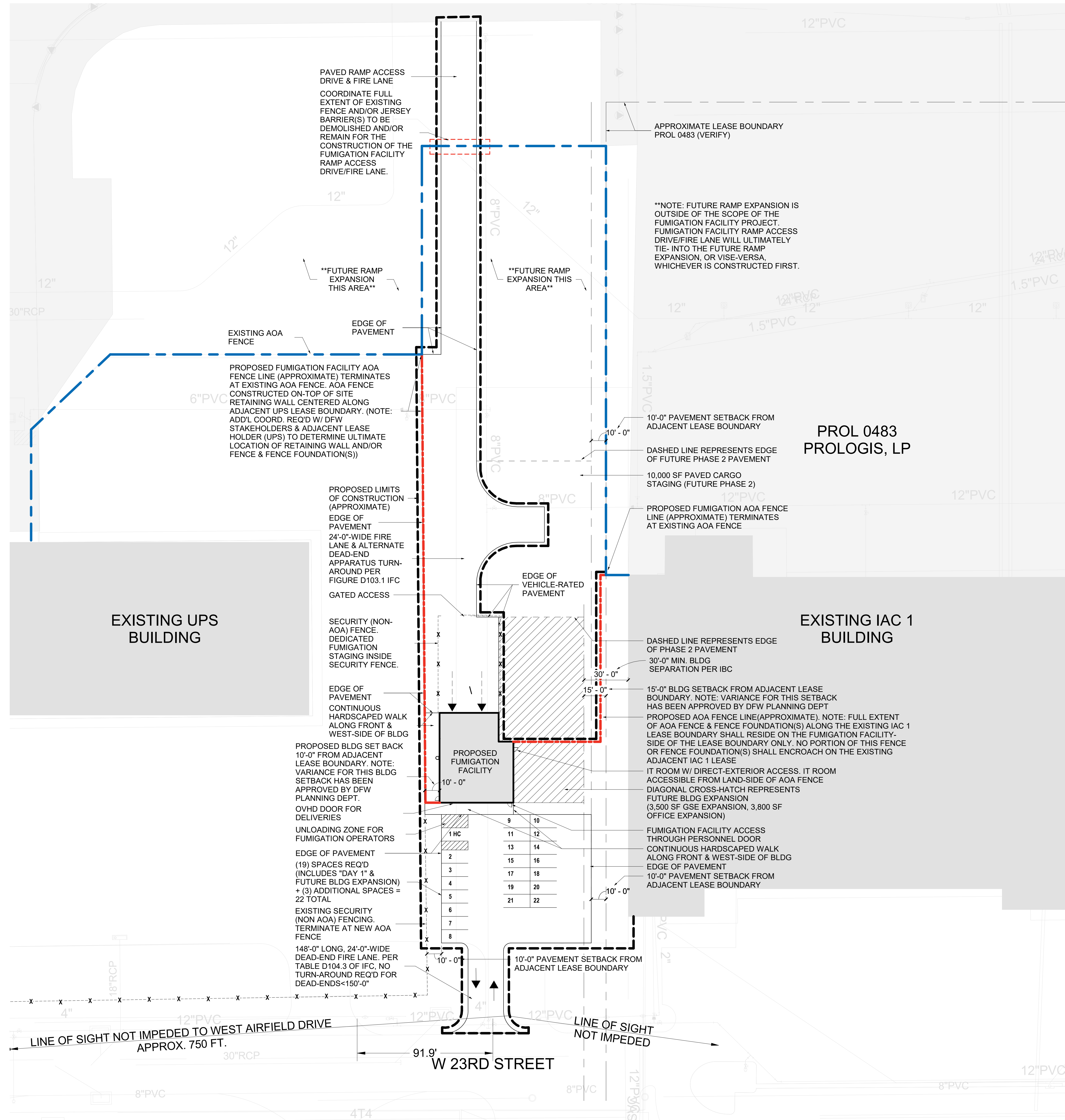
1 CONSTRUCTION PLAN - FUMIGATION FACILITY ENLARGED SCALE: 1" = 30'-0"
