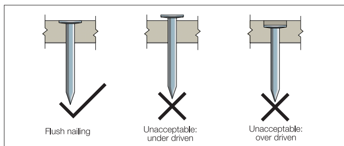
FIGURE 2: NAIL FASTENER DEPTH
