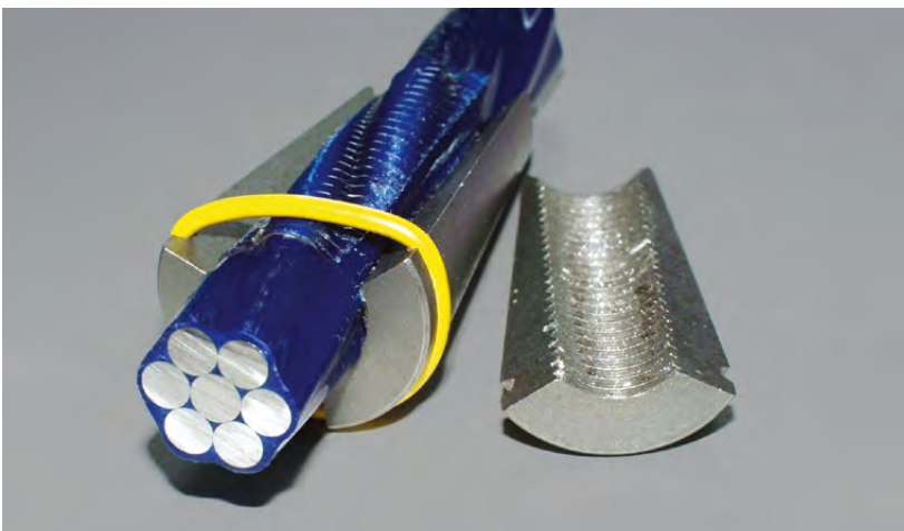
Wedge for Epoxy Strands
