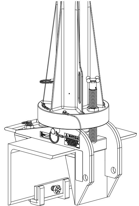
TOP MOUNT
