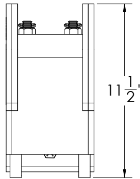
FRONT VIEW MAXIMUM ANGLE BEAM
