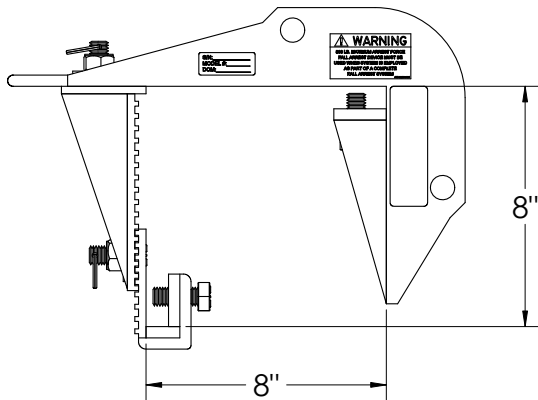
SIDE VIEW MAXIMUM ANGLE BEAM
