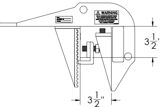
SIDE VIEW MINIMUM ANGLE BEAM
