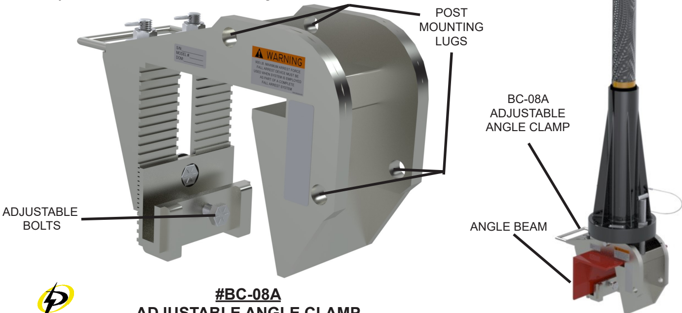
ADJUSTABLE ANGLE CLAMP SHOWN ON A TYPICAL STRUCTURAL ANGLE SECTION WITH A MODEL #FT-C70 FALL ARREST POST INSTALLED
