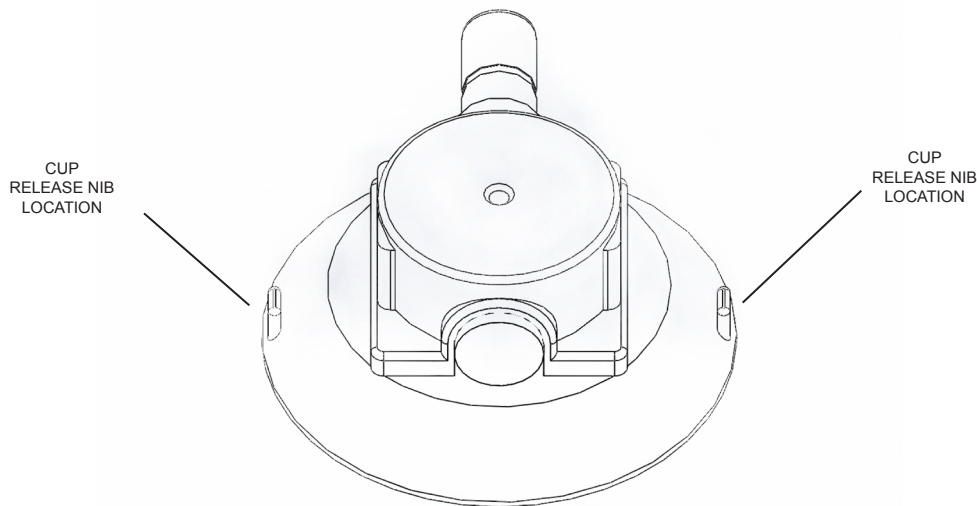
Figure #5.2b: Location of cup nibs for release of vacuum mount.
