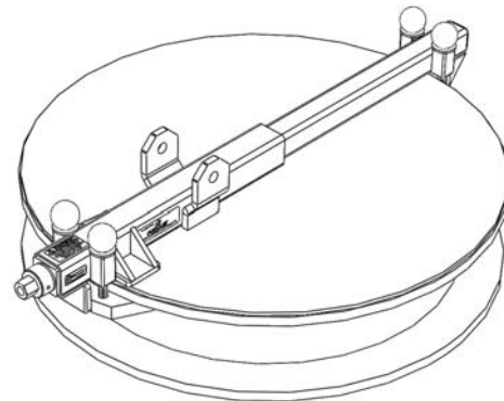
Figure #5b: AC-R Series Installed on a Manway (Maximum Diameter)
