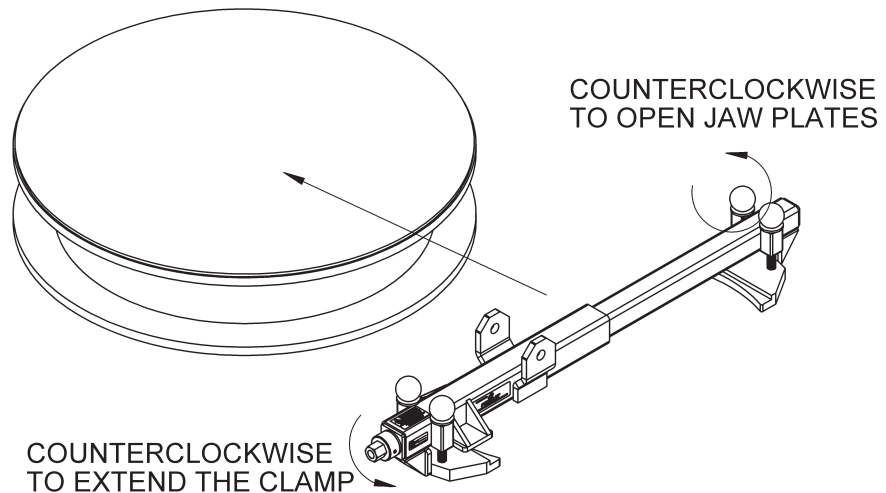
Figure #5f: Installation Step “b”
