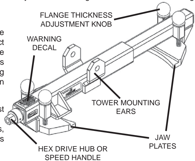
Figure #5d: AC-R Series Pre-Operation Inspection Points
