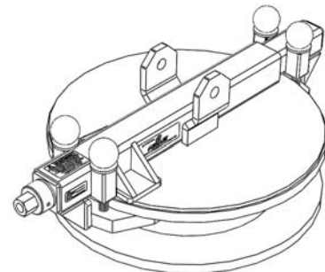
Figure #5a: AC-R Series Installed on a Manway (Minimum Diameter)
