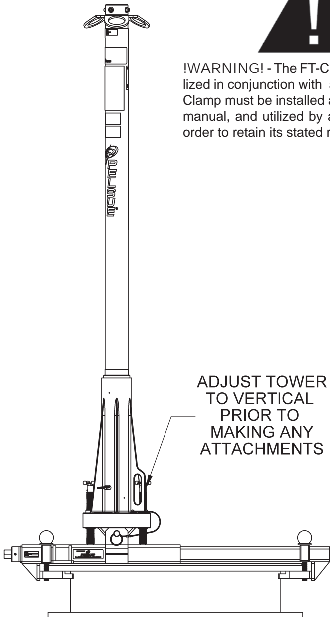
Figure #5n: Tower #FT-C70 Installation Step "e"
