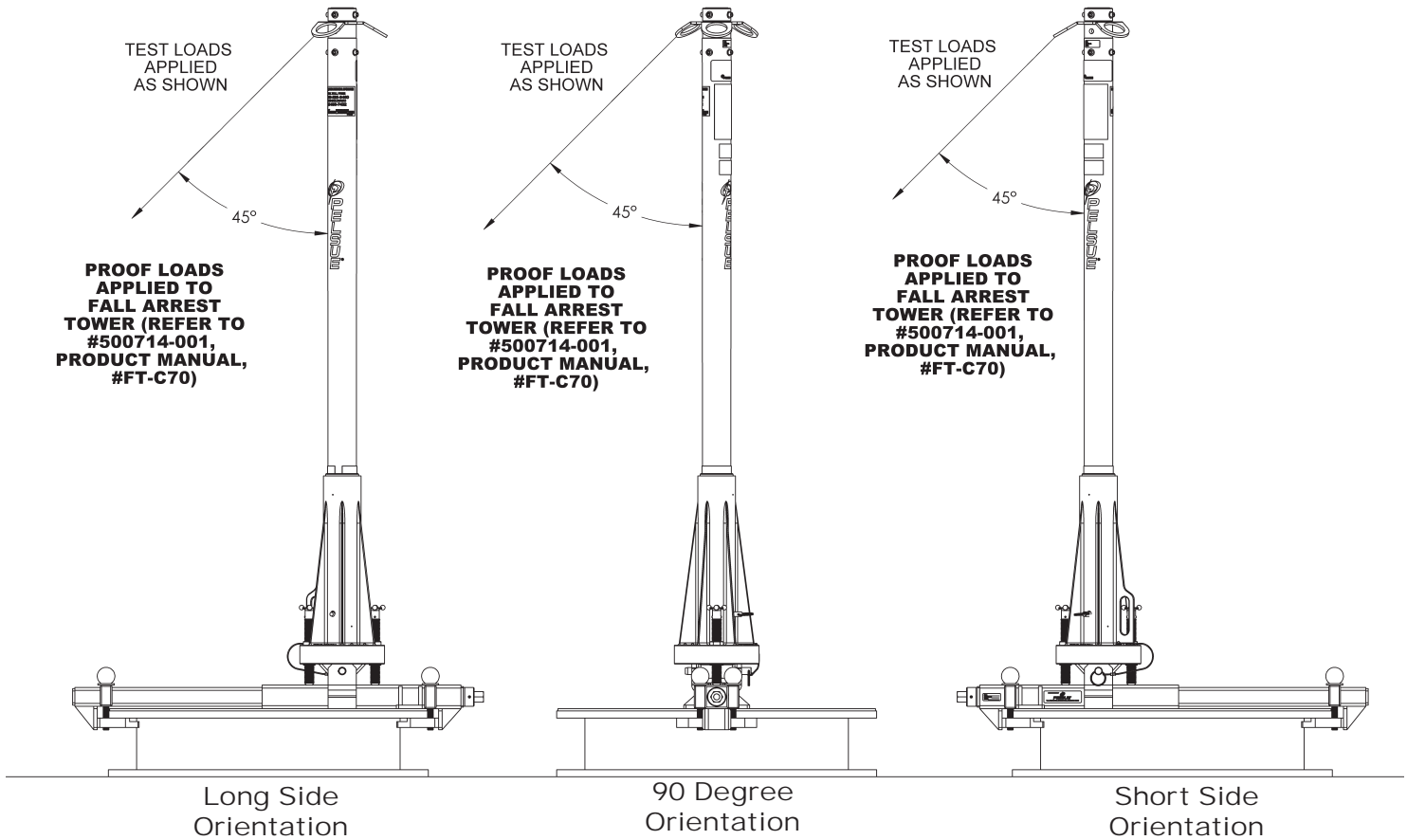
Figure #5c: AC-R Series Anchor Clamp, Testing & Loading Diagram
