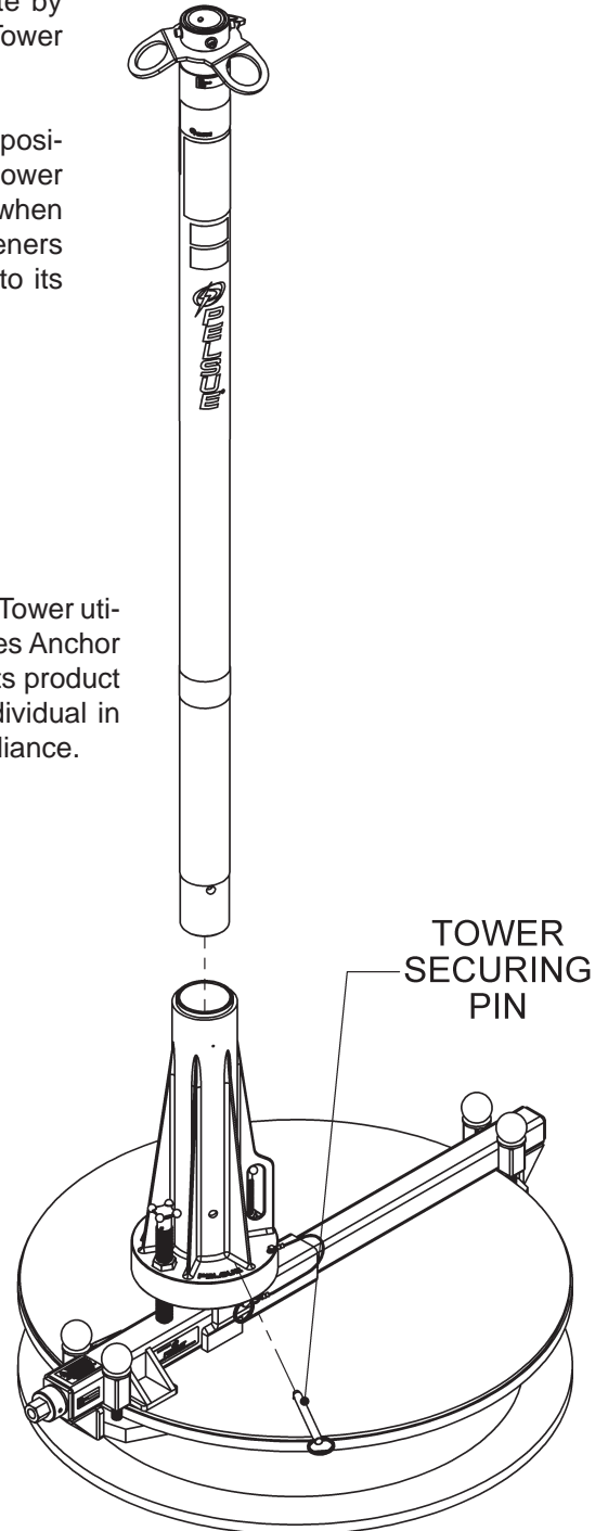
Figure #5m: Tower #FT-C70 Installation Step "d"
