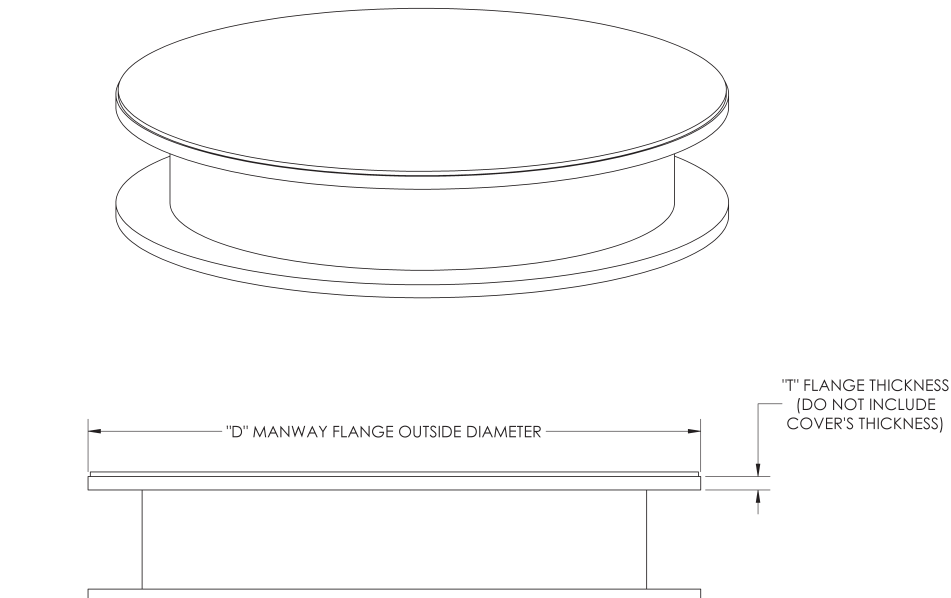
Figure #5e: Manway Diagram with Dimensional Definitions (typical, Round Construction)
