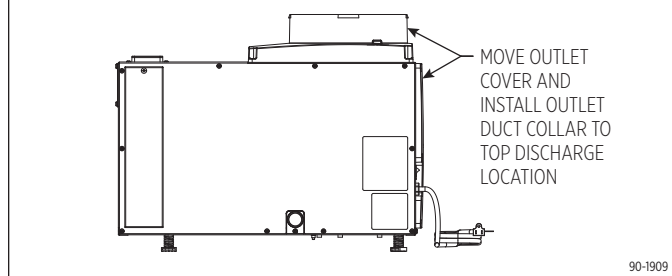
FIGURE 4 – FLOOR MOUNT INSTALL
