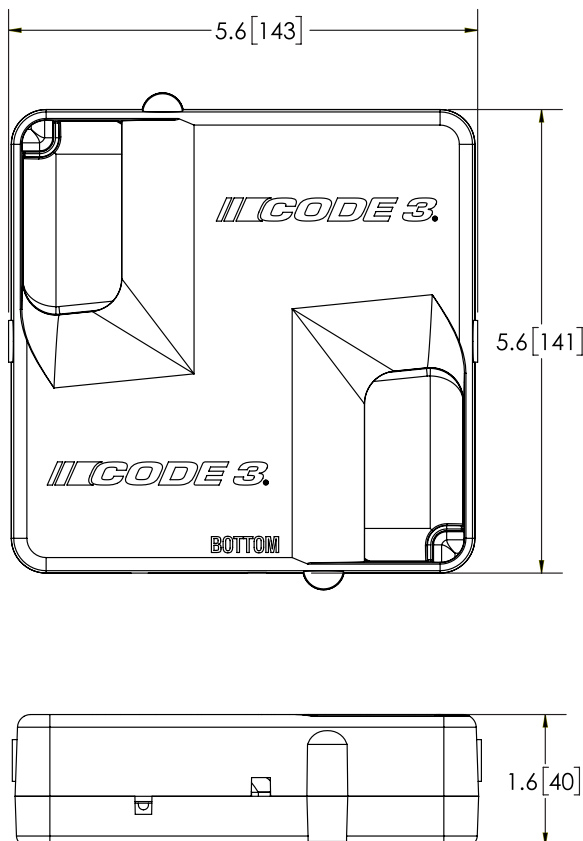
CZ0142 Siren Bracket 2015+ F150, 2018+ EXPEDITION SINGLE/DUAL
