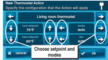
New Thermostat Action Screen
