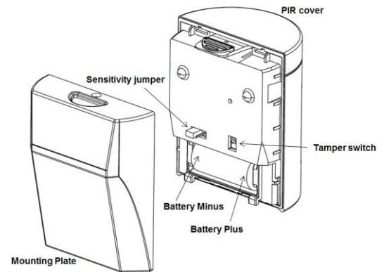
Figure 8: PIR Components, Battery Locations & Tamper Switch
