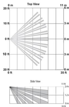
Figure 7: High Sensitivity Setting
