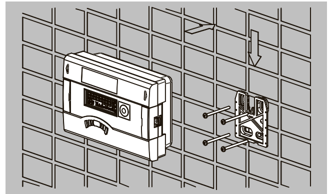
Wall mounting
