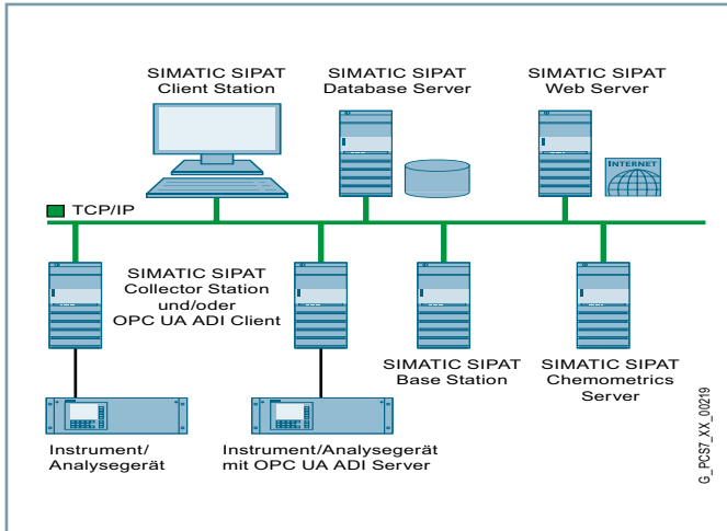
SIMATIC SIPAT distributed architecture diagram
