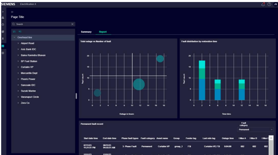
Electrification X – Network Fault Management (Overhead Line Fault Management): Fault Analysis Report view
