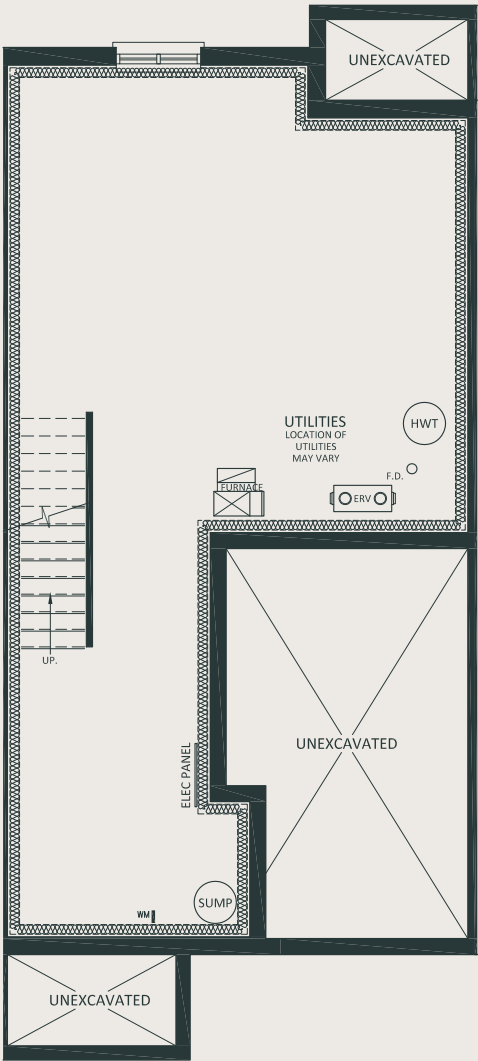
BASEMENT
