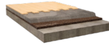
Slab and Floors Support for nailed flooring
