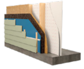
Interior solutions for exterior walls Support for wooden wainscot
