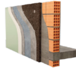
External walls Exterior cladding - cork at sight
