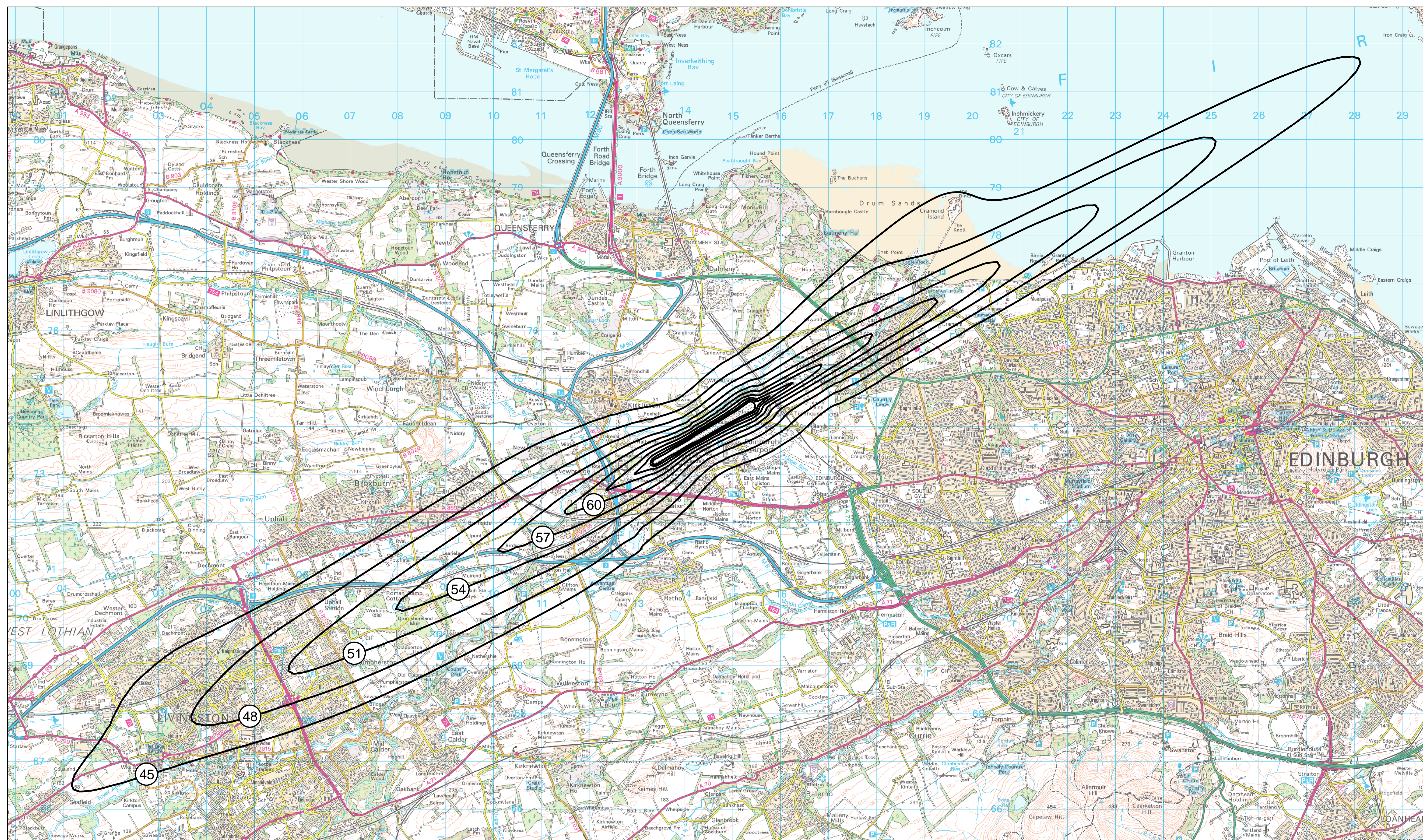
EDINBURGH AIRPORT 2023 Average Summer Night 45-72 dB L_{Aeq,8h} Contours Actual Runway Modal Split 79%W / 21%E
