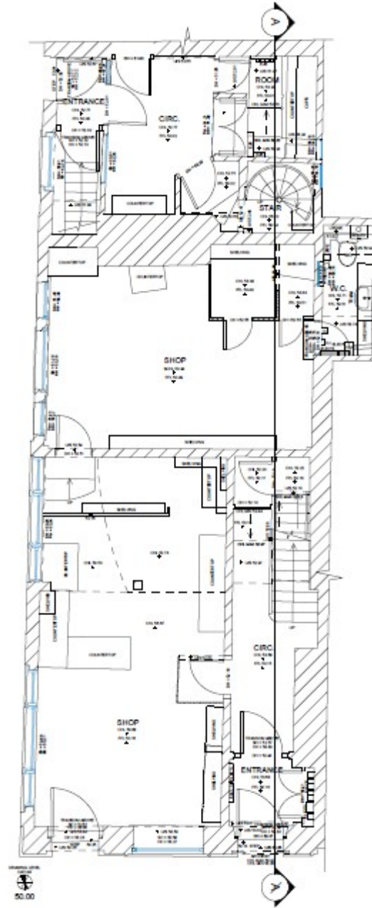
Ground Floor
