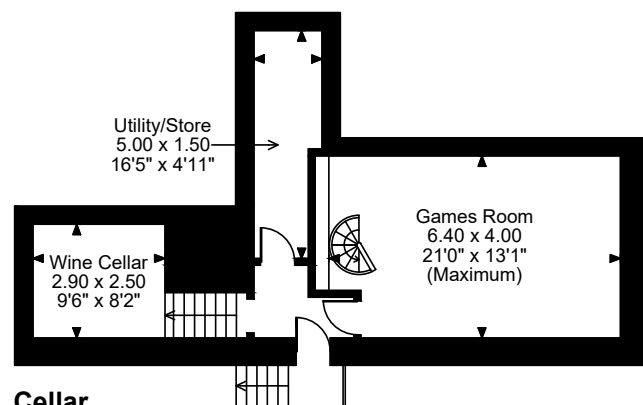
Cellar
