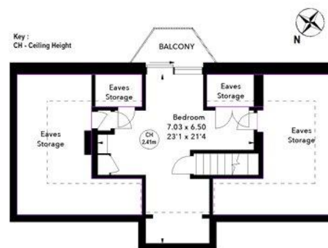
Second Floor Approx. 81.01 sq m / 872 sq ft
