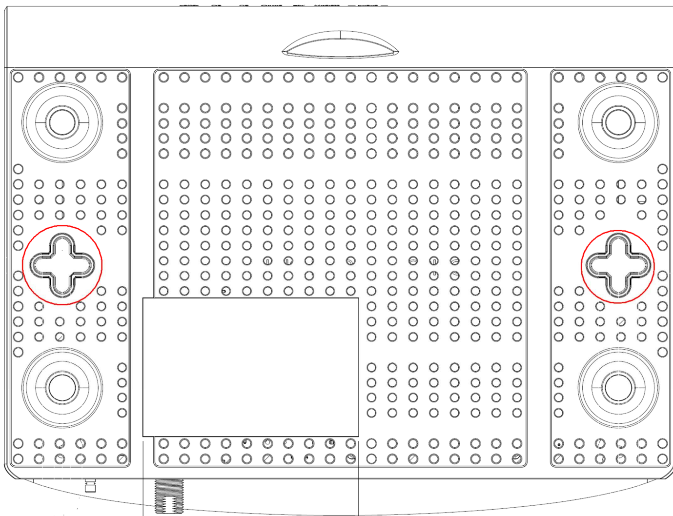
Abb. 1-4 Wandmontage
