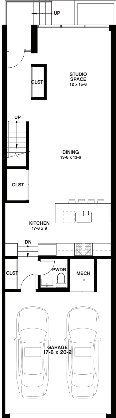
First Floor
