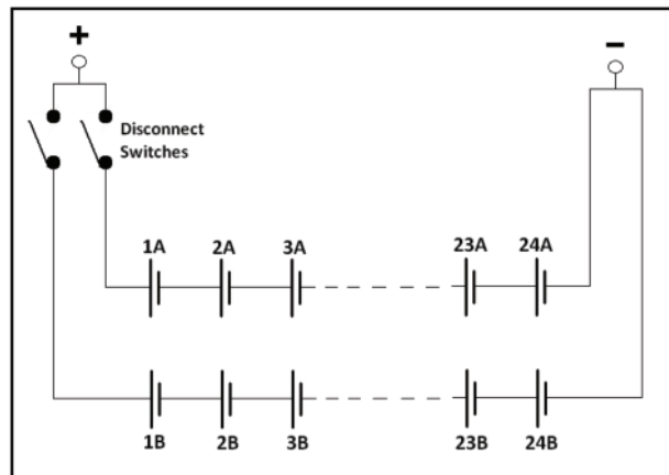
Figure 2 – Parallel Connected Strings
