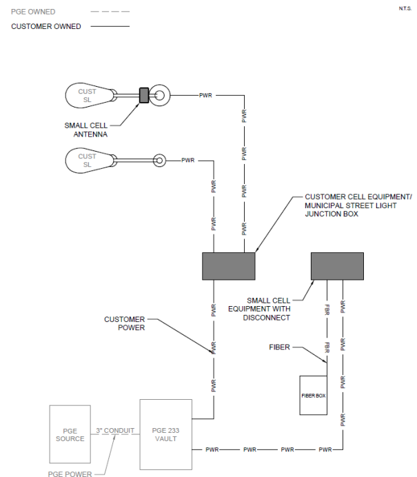
Figure 2. Electrical Service for Option C (Customer-Owned Poles)
