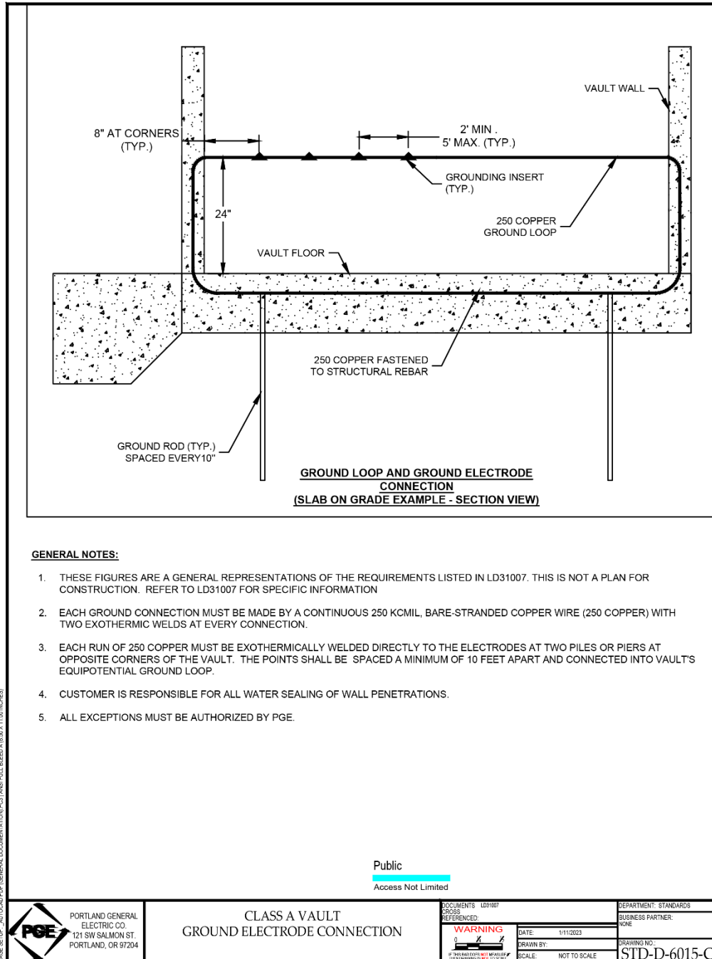
Figure 13. Slab on Grade Vault
