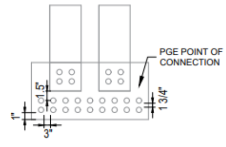
DIMENSIONS FOR TWO BUS CUT FLANGE CONNECTIONS
