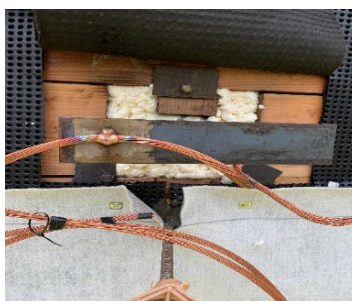
Figure 12. Components Joined by a Continuous Weld
