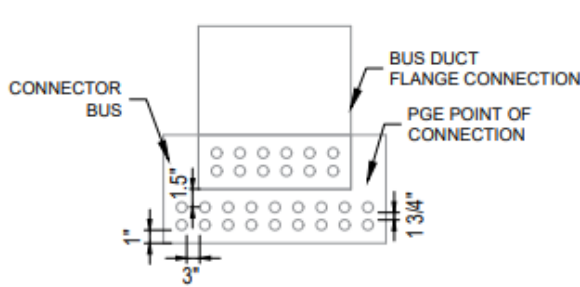
DIMENSIONS OF SINGLE BUS DUCT FLANGE CONNECTIONS
