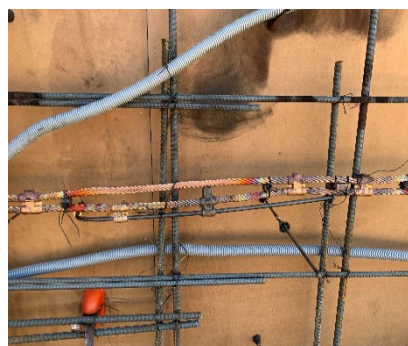
Figure 15. Cadweld Connection Options
