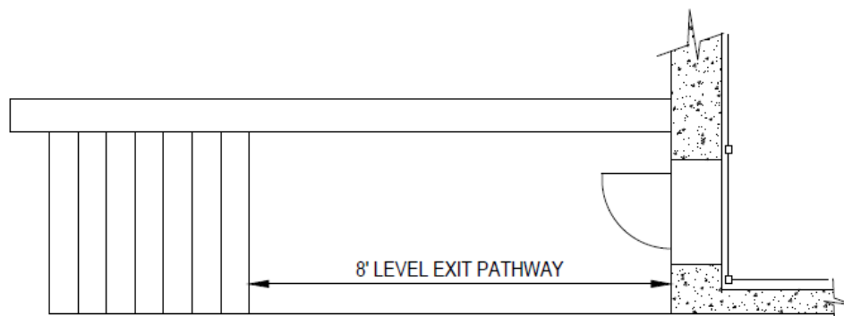
Figure 4. 8-Foot Level Egress Corridor (STD-D-6300)
