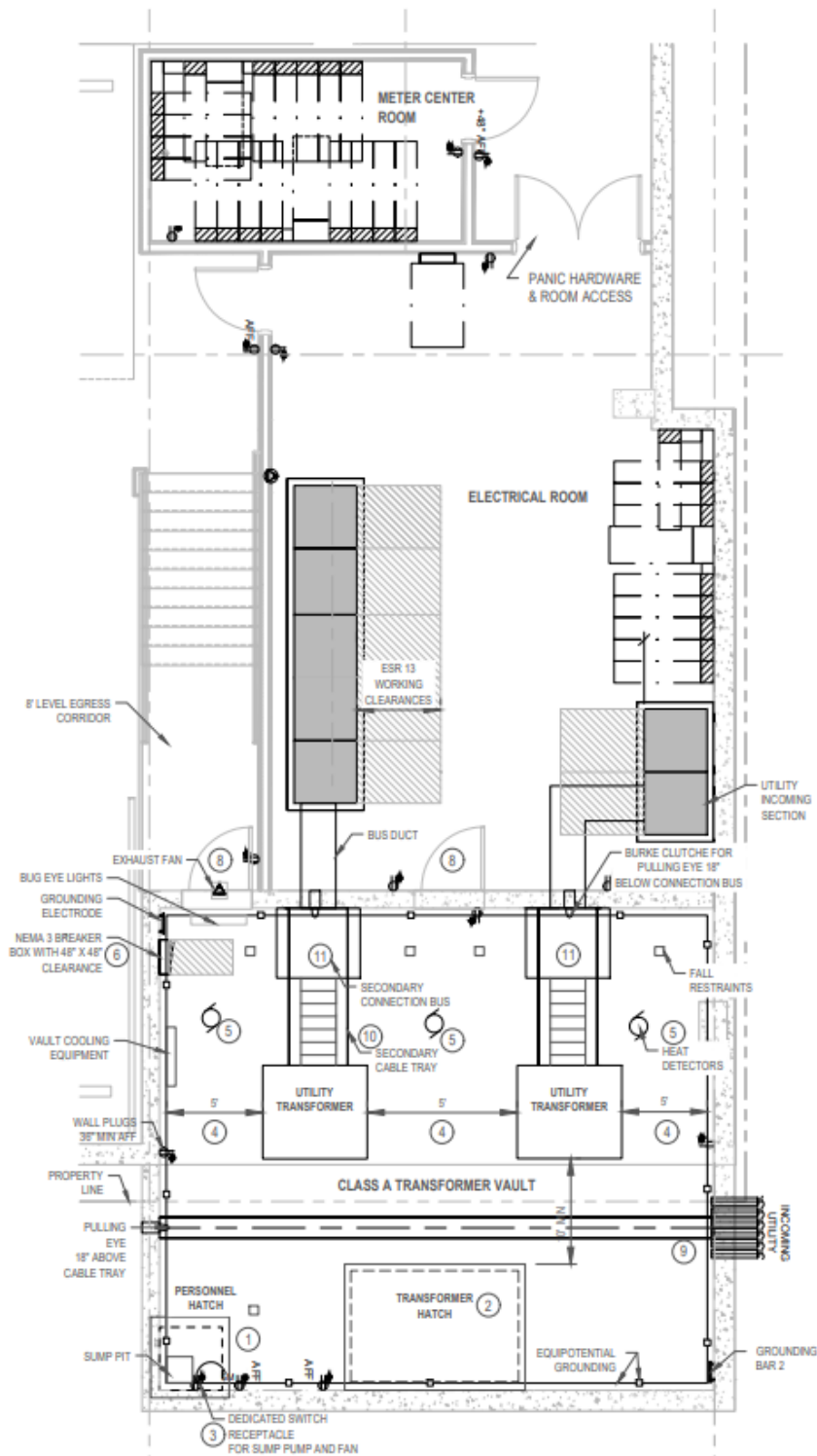
Figure 2. Overhead View of a Sub-Grade Class A Vault and Electrical Room (STD-D-6308-1)
