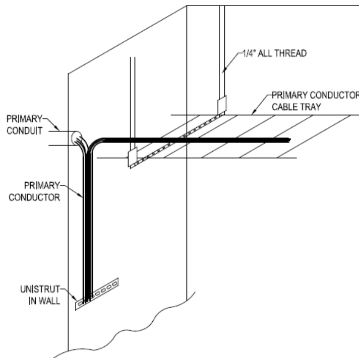
Figure 20. Primary Laterals with Point of Isolation in a Sub-Grade Vault(STD-D-3223)
