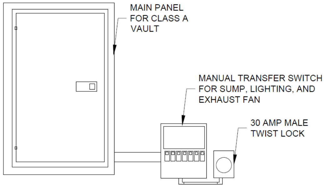
Figure 35. Class A Vault Electrical Panels Where No Generator Exists On-site (STD-D-6314)
