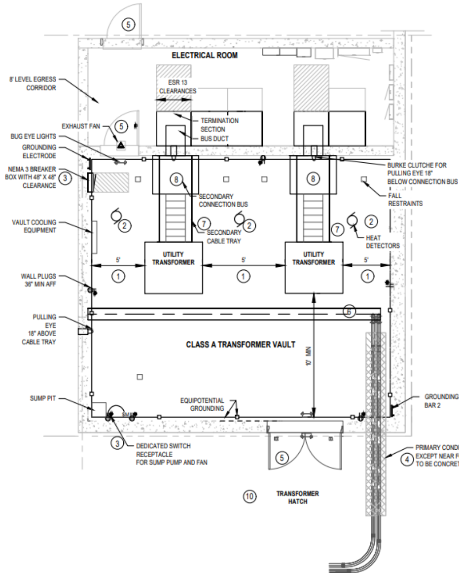
Figure 1. Overhead View of an At-Grade Class A Vault and Electrical Room (STD-D-6308-2)
