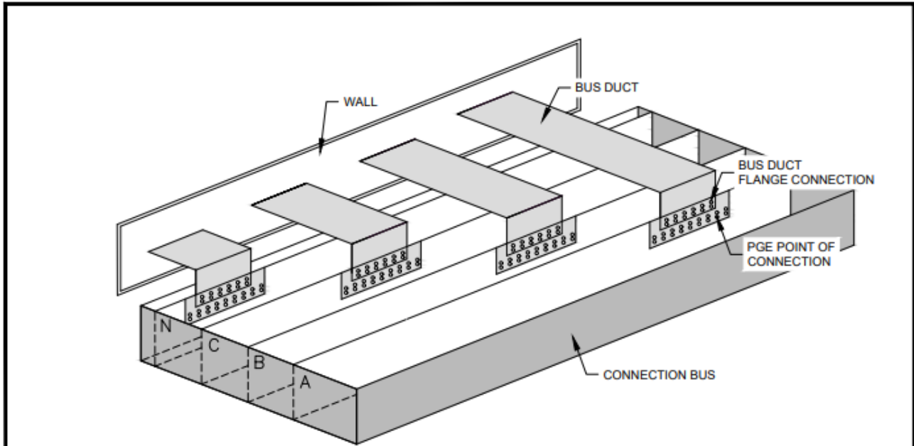
BUS COUPLER EXAMPLE - ISOMETRIC VIEW NON-ALIGNED FOR ILLUSTRATIVE PURPOSES
