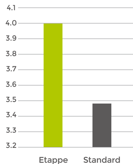
Average bunch per meter
