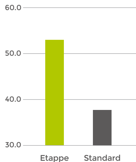
Average germination per meter
