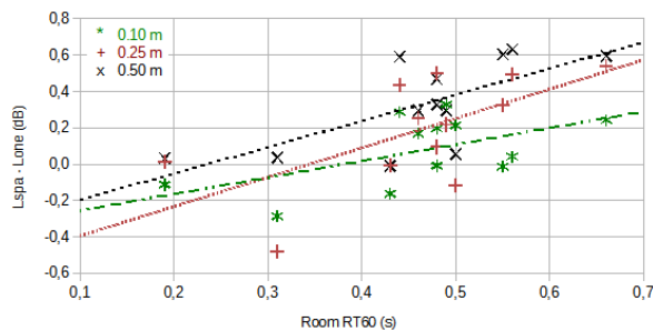
Figure 7. Mean level difference in octave bands, averaged across the audio band for the spatial offset cases 0.1, 0.25 and 0.5 m. The reverberation time RT60 is the maximum within the frequencies 0.4-4 kHz.
