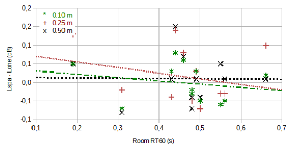
Figure 8. Mean level difference in octave bands 500 Hz and above, averaged across the audio band for the spatial offset cases 0.1, 0.25 and 0.5 m. The reverberation time RT60 is the maximum within the frequencies 0.4-4 kHz.
