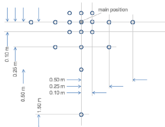
Figure 1. The definitions of the spatial averaging measurement positions; 'main position' is the nominal listener/microphone position.
