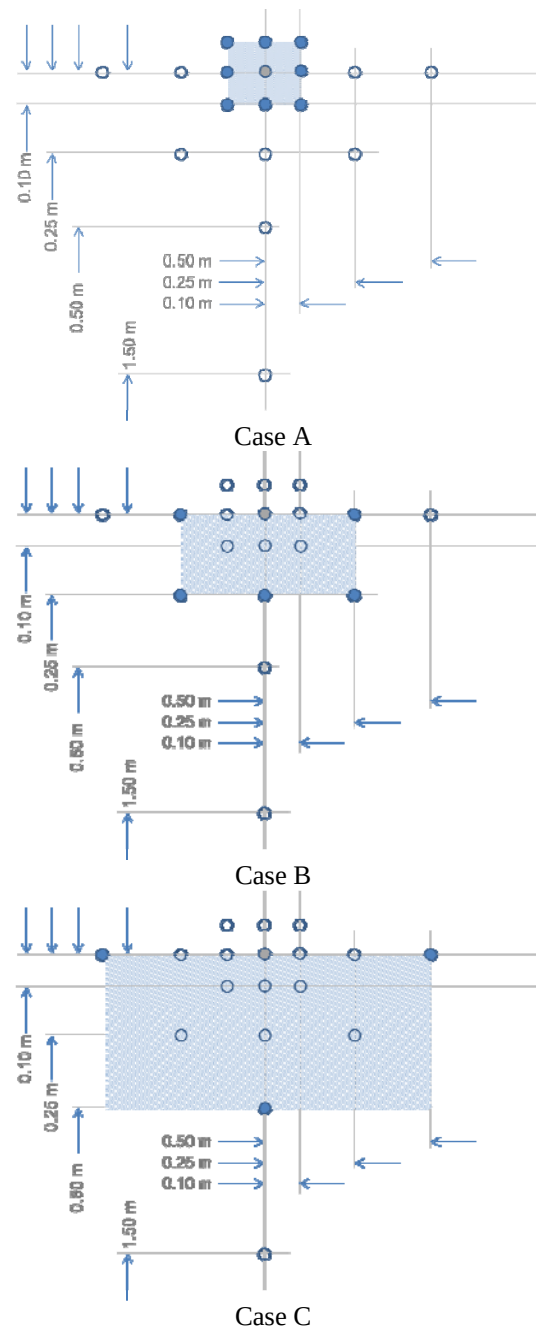
Figure 3. Definitions of the spatial average cases A to C showing the spatial averaging areas (shaded) and the numbers of measurement positions used (dark colour).
