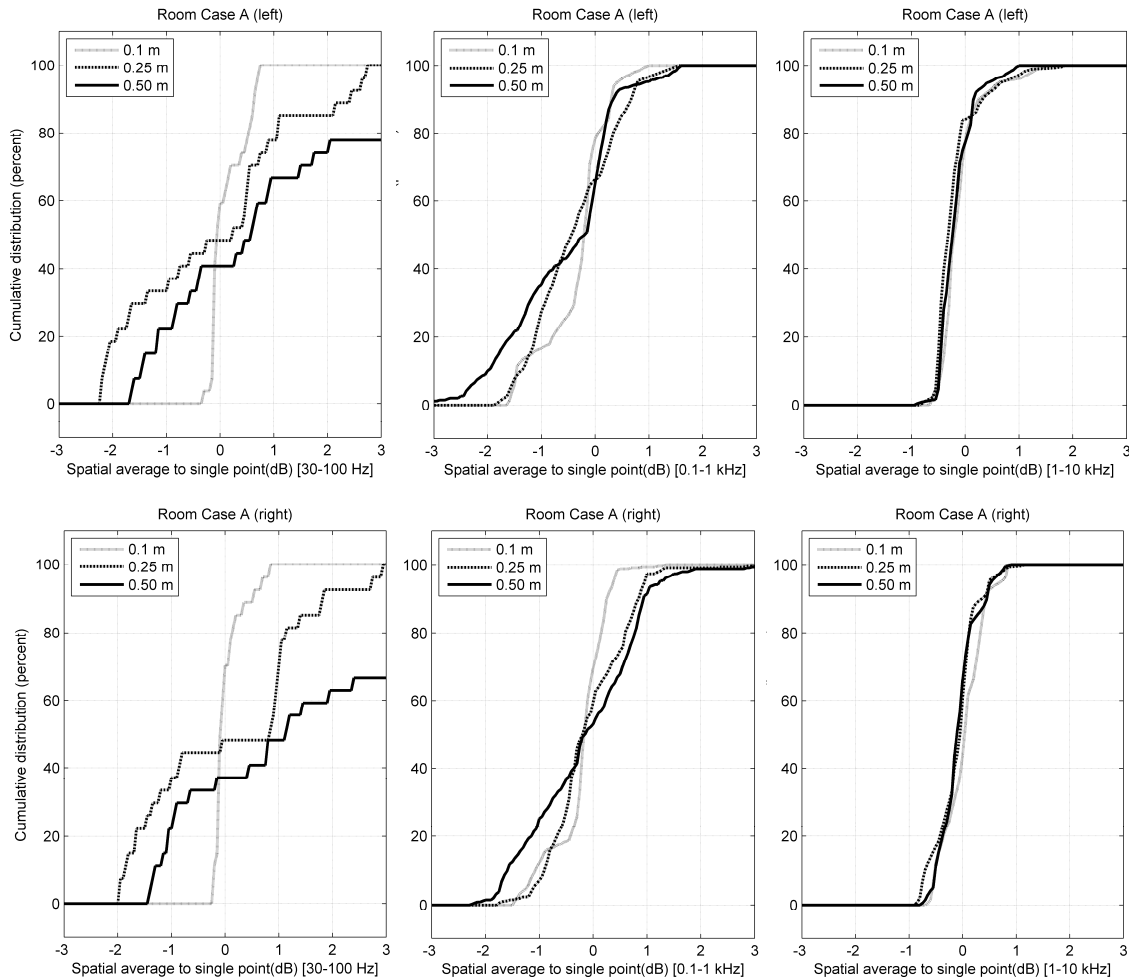
Figure 5. Example of results is Room A, cumulative distribution of the difference of the spatial average SPL from the single position SPL, left monitor (top) and right monitor (bottom); the cumulative distributions are presented in three different frequency bands (30-100 Hz, 100-1000 Hz and 1-10 kHz).
