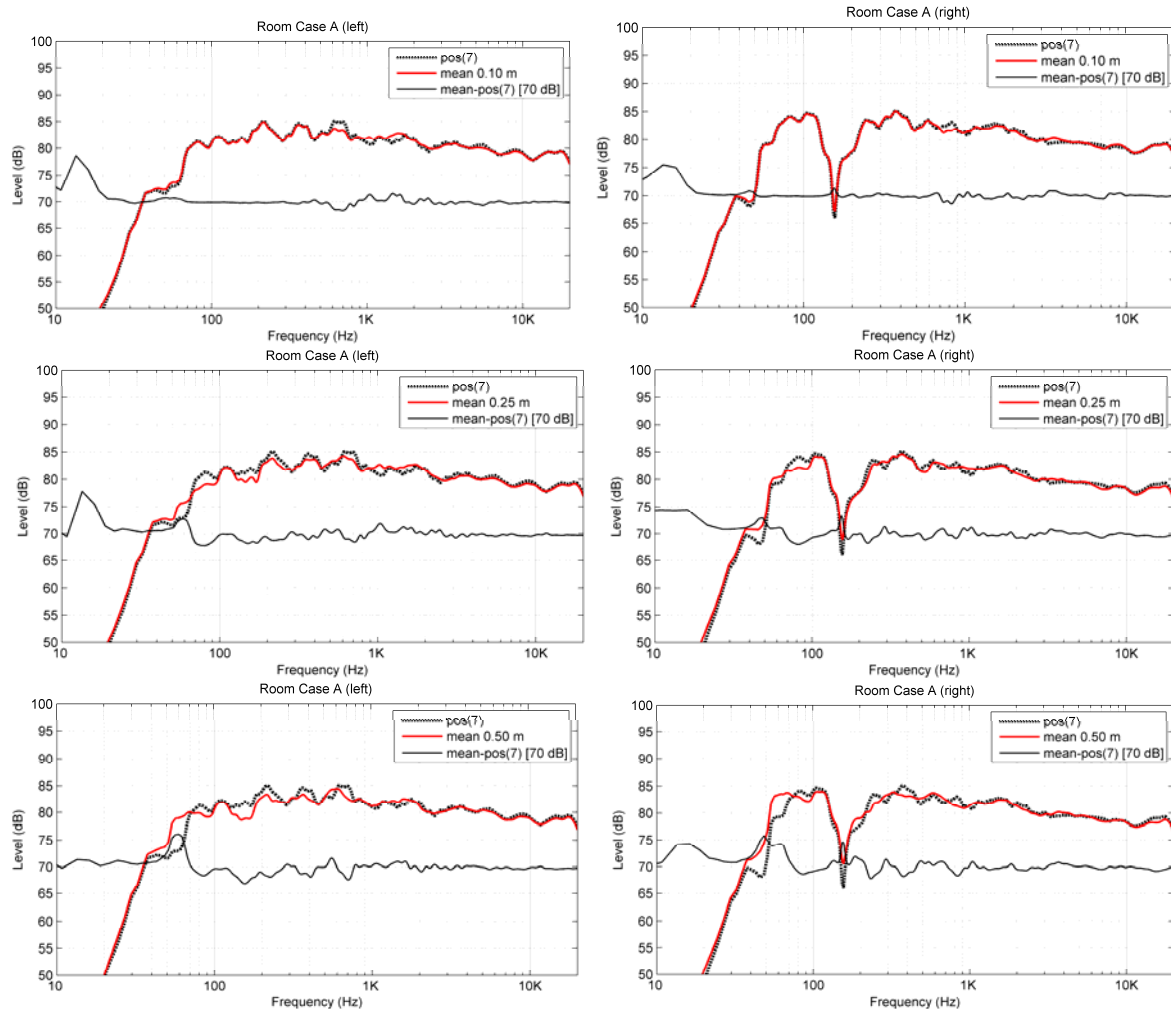
Figure 4. Example of a results is Room A, left and right monitors, spatial means at 0.1, 0.25, and 0.5 m distances from the nominal listening position, compared to the single response at the nominal listening position; difference between the spatial mean and the single mic position is shown with zero shifted to the level 70 dB.
