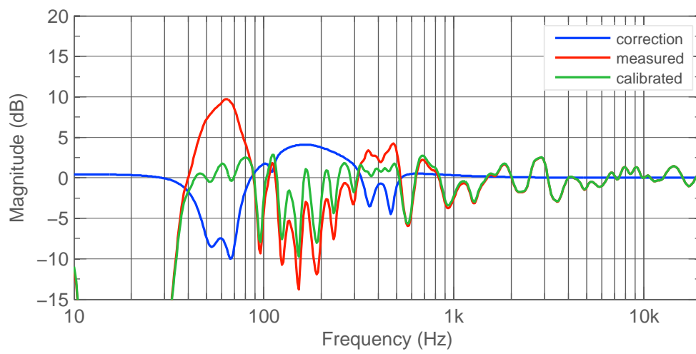
Figure 3.15: Left Side 8341A frequency response.
