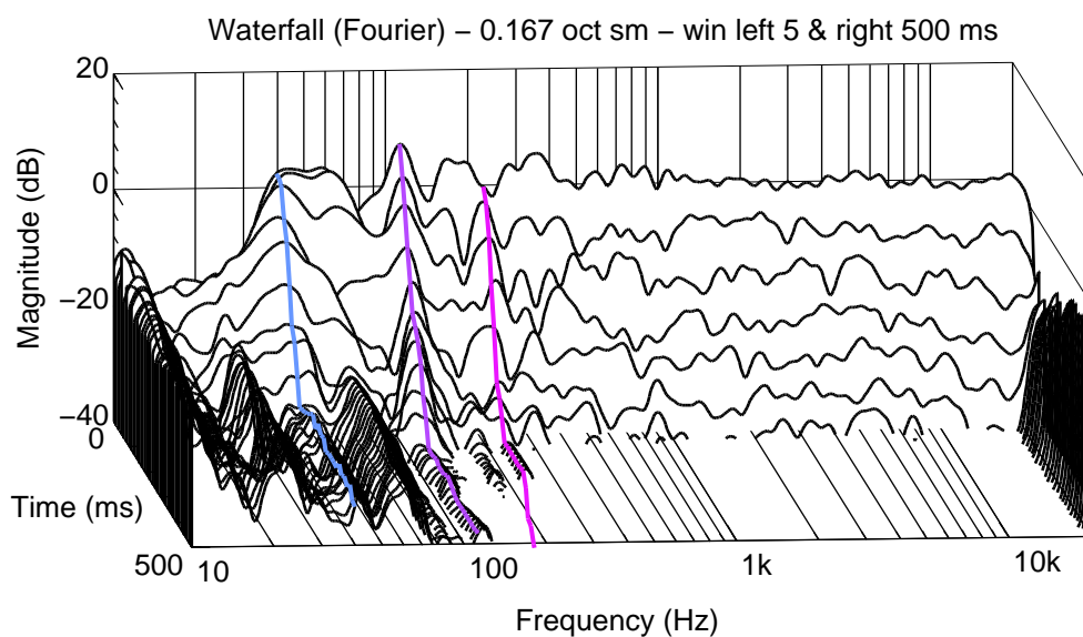
Figure 5.12: T R Rear. Waterfall.
