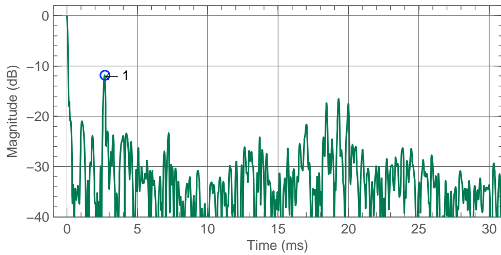
Figure 4.26: Right Side 8341A early reflections.
