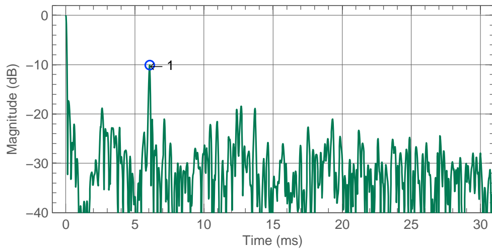
Figure 4.8: T R Mid early reflections.
