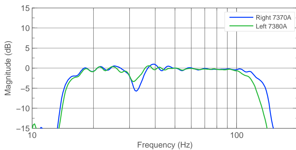
Figure 3.26: Filtered frequency responses for subwoofers. 1/12 octave smoothing.
