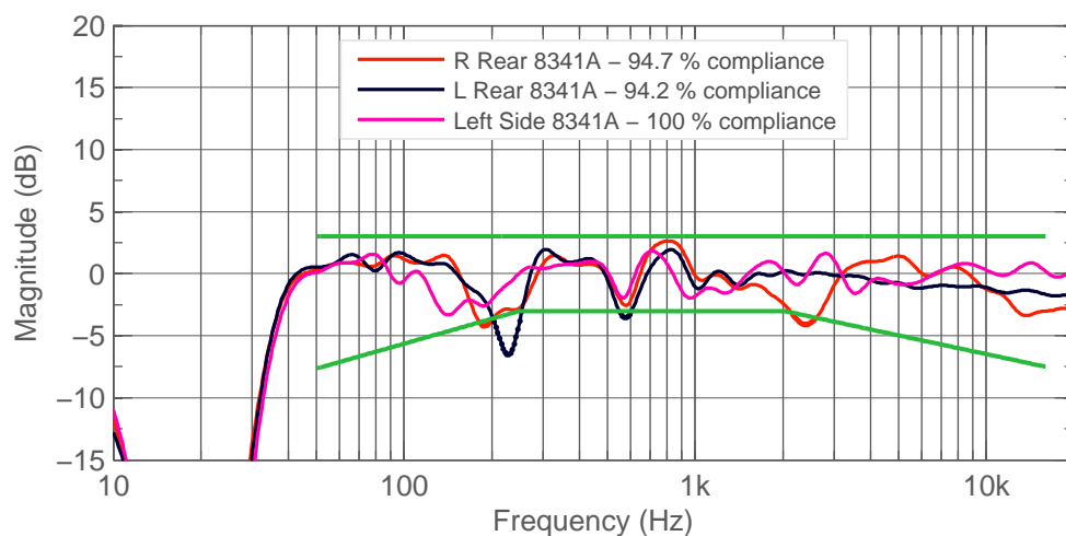
Figure 6.4: Operational room response curve.
