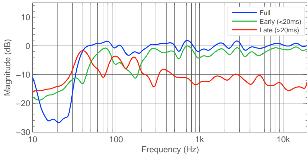
Figure 4.48: Left Side 8341A. Full, early and late frequency response.
