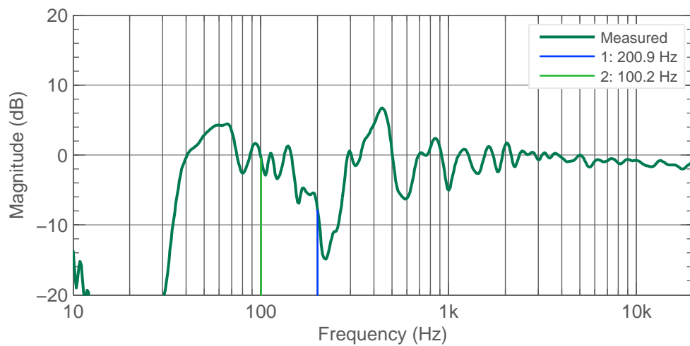
Figure 4.31: L Rear 8341A. Response and lowest cancellation frequency resulting from early reflection.
