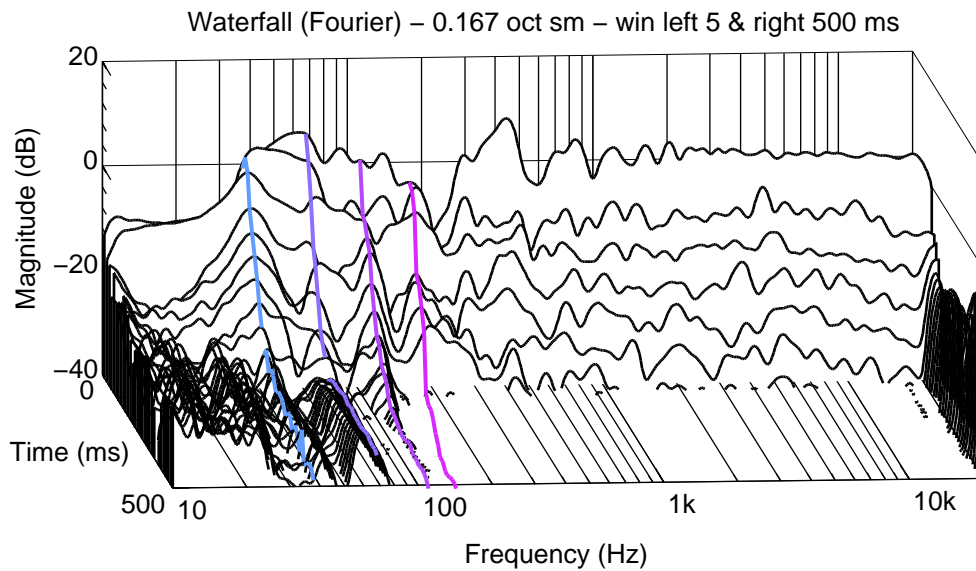
Figure 5.32: L Rear 8341A. Waterfall.
