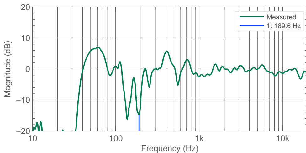
Figure 4.25: Right 8341A w. Response and lowest cancellation frequency resulting from early reflection.
