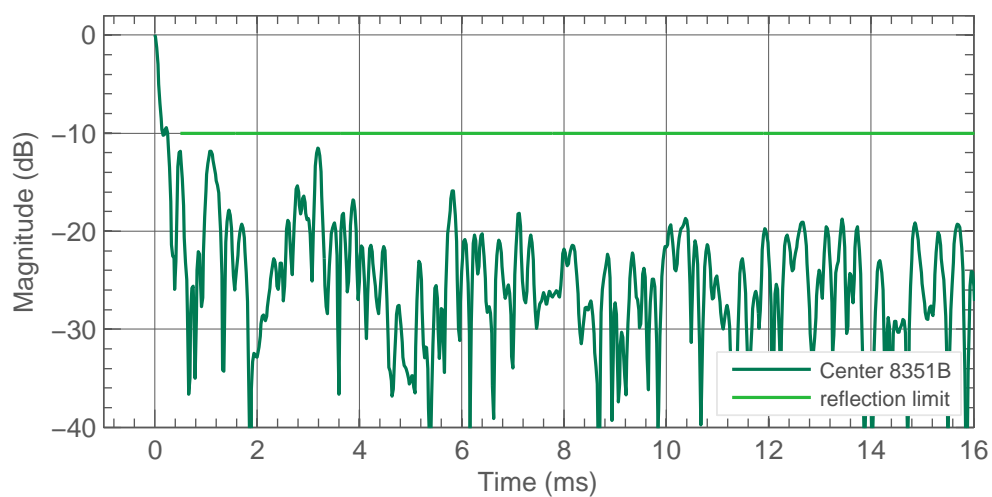
Figure 6.11: Early reflections. 1-8 kHz band. Level is relative to direct sound level.
