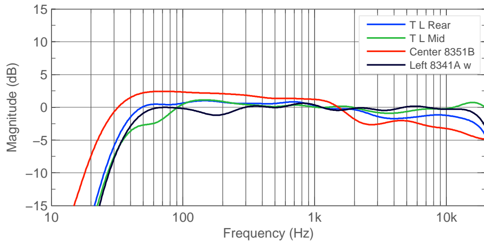
Figure 3.23: Frequency responses for monitors. One octave smoothing.
