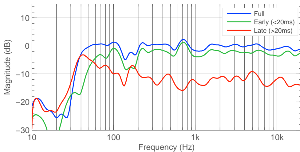
Figure 4.44: Right 8341A w. Full, early and late frequency response.
