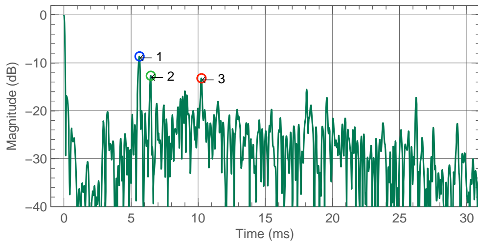
Figure 4.12: T L Rear early reflections.
