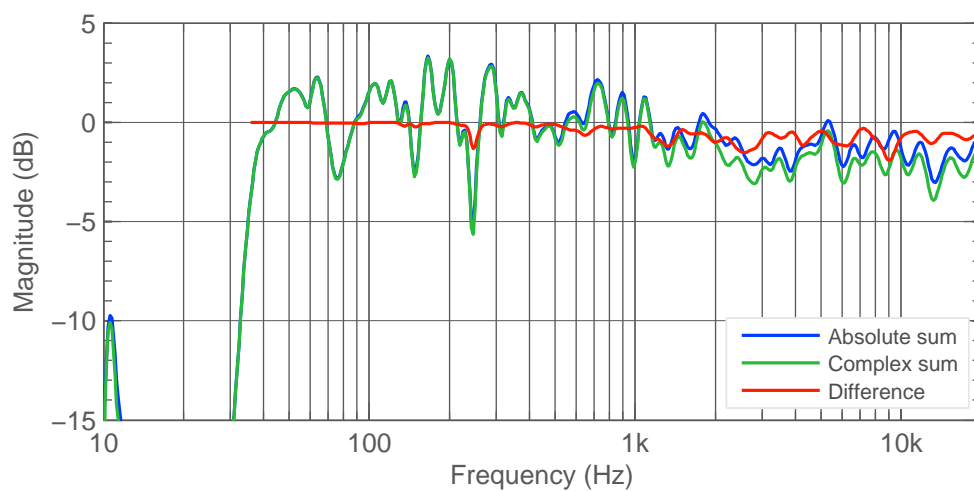
Figure 3.29: Difference between the sum of complex pressure and sum of absolute pressure. Calibration group ID 6.
