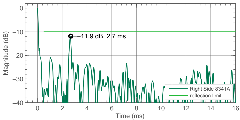
Figure 6.16: Early reflections. 1-8 kHz band. Level is relative to direct sound level.
