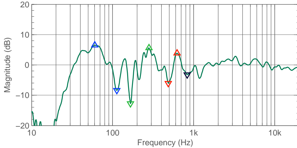
Figure 3.42: Left 8351B peaks and notches (before calibration).
