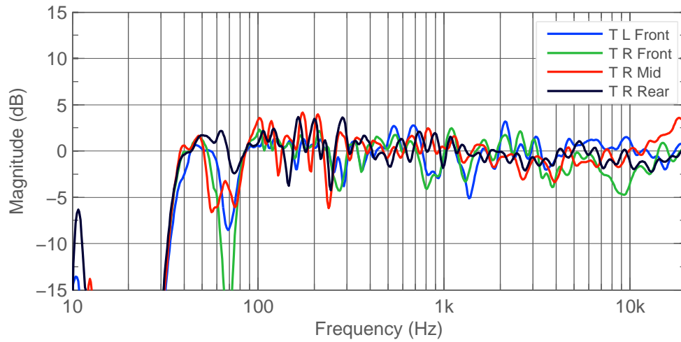
Figure 3.18: Frequency responses for monitors. AccuSmoothed.
