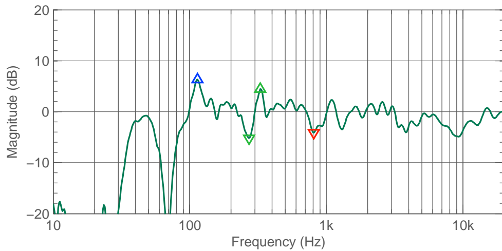
Figure 3.35: T R Front peaks and notches (before calibration).
