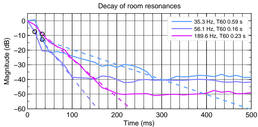
Figure 5.23: Left 8351B. Decay of detected resonances.
