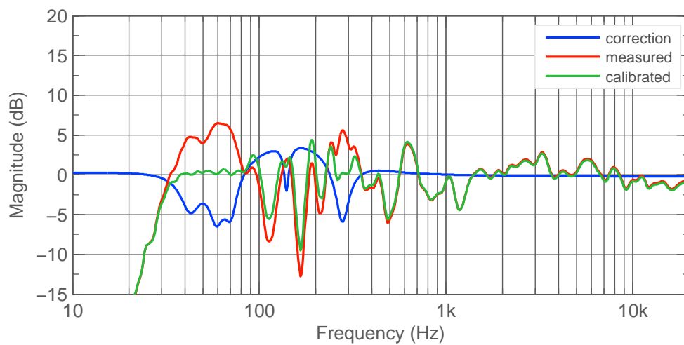
Figure 3.9: Left 8351B frequency response.
