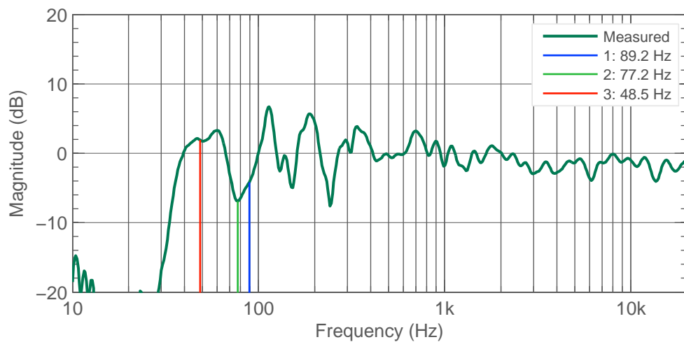
Figure 4.13: T L Rear. Response and lowest cancellation frequency resulting from early reflection.
