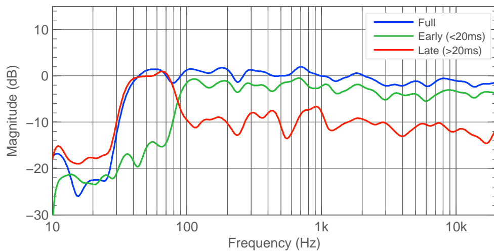
Figure 4.38: T L Rear. Full, early and late frequency response.
