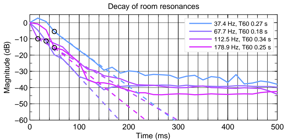
Figure 5.33: L Rear 8341A. Decay of detected resonances.
