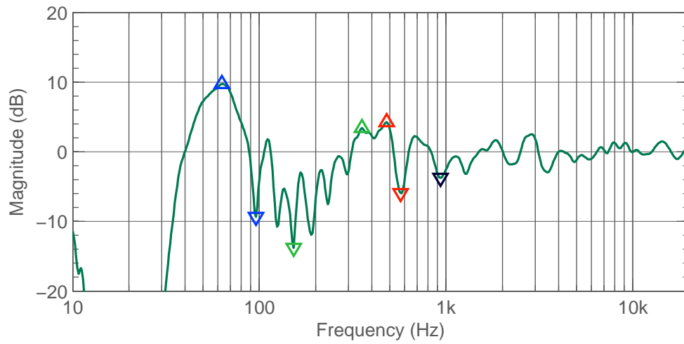
Figure 3.48: Left Side 8341A peaks and notches (before calibration).
