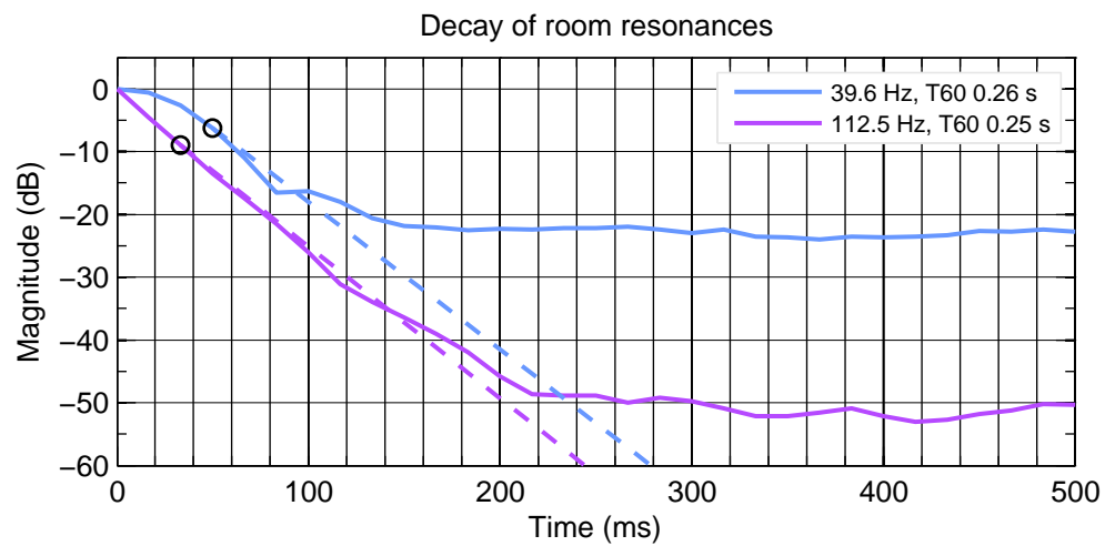
Figure 5.17: T L Mid. Decay of detected resonances.
