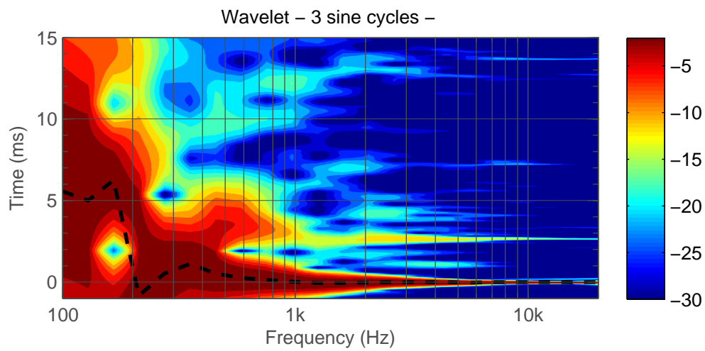
Figure 5.52: Right Side 8341A. Wavelet.
