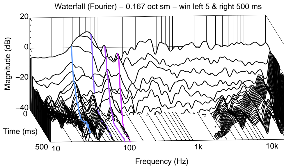
Figure 5.34: Left Side 8341A. Waterfall.
