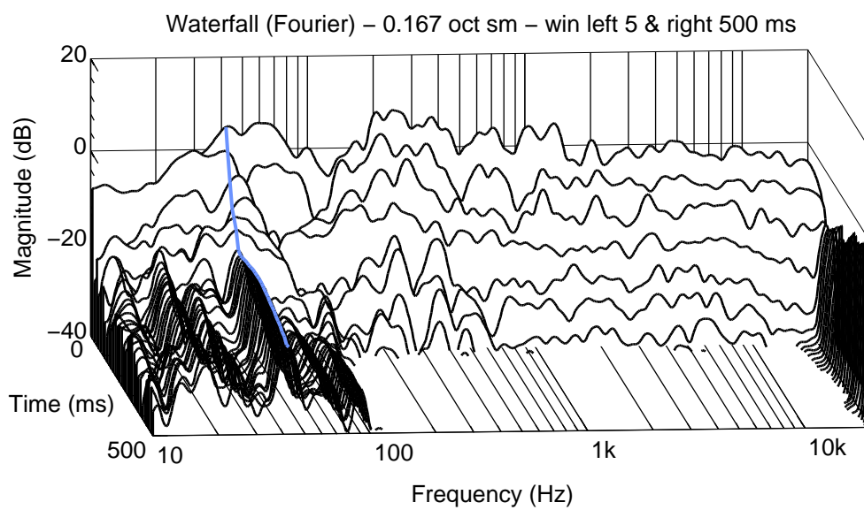
Figure 5.18: Center 8351B. Waterfall.
