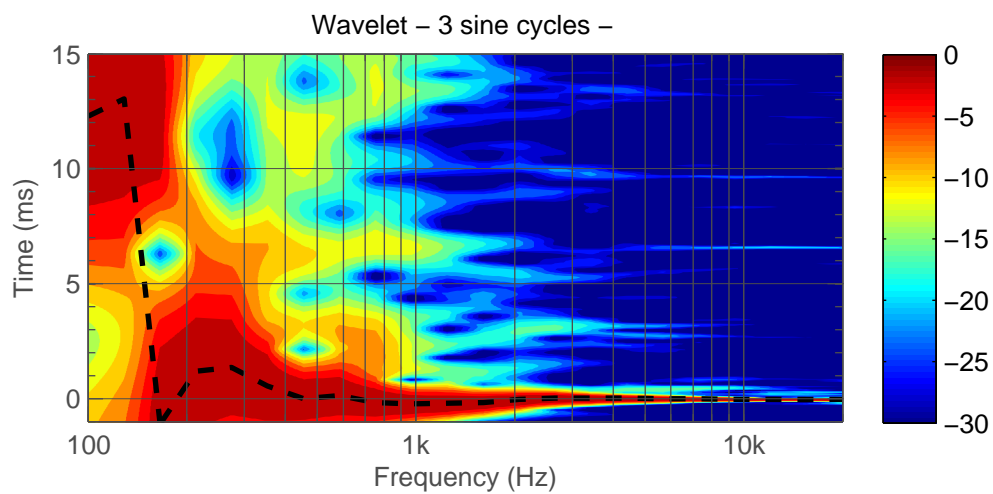
Figure 5.50: Right 8351B. Wavelet.
