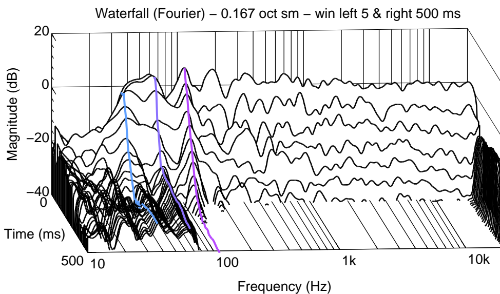
Figure 5.14: T L Rear. Waterfall.
