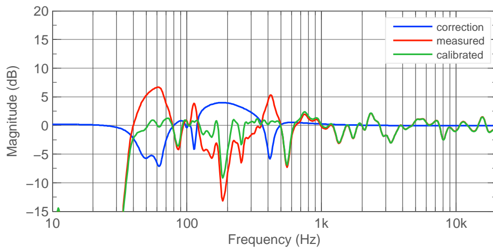
Figure 3.8: Left 8341A w frequency response.
