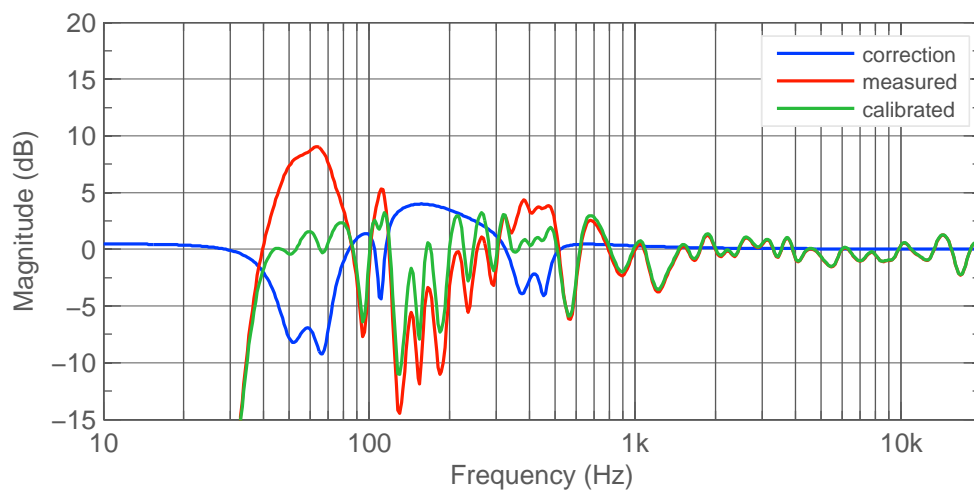
Figure 3.12: Right Side 8341A frequency response.
