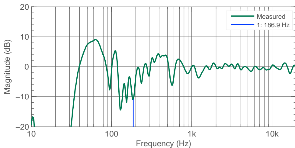
Figure 4.27: Right Side 8341A. Response and lowest cancellation frequency resulting from early reflection.
