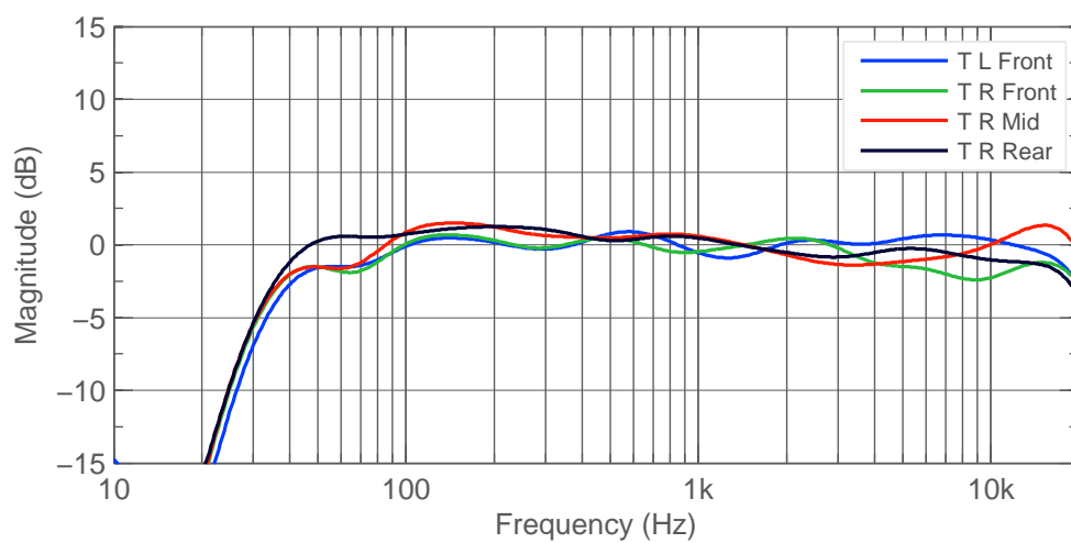
Figure 3.22: Frequency responses for monitors. One octave smoothing.
