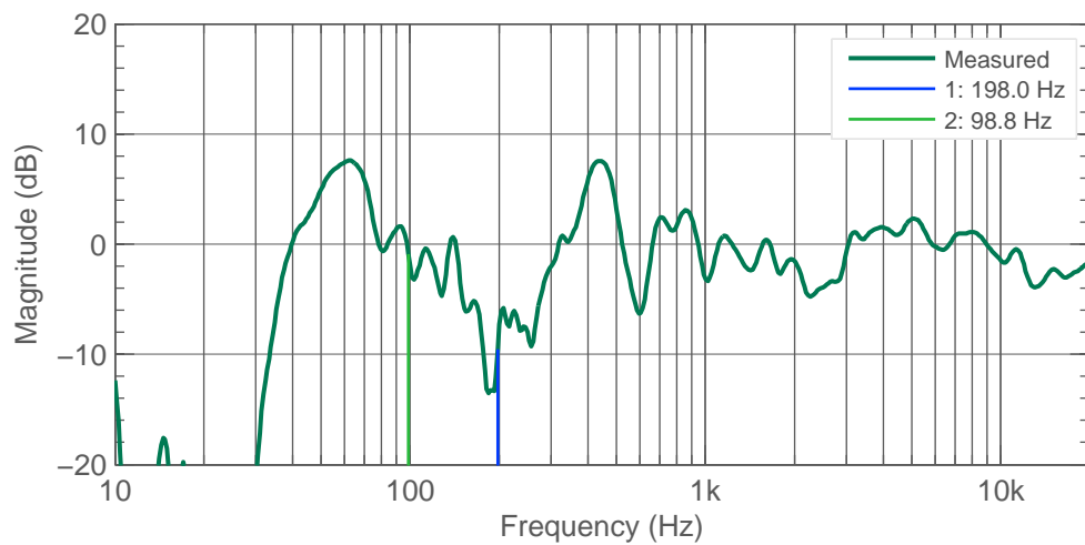
Figure 4.29: R Rear 8341A. Response and lowest cancellation frequency resulting from early reflection.
