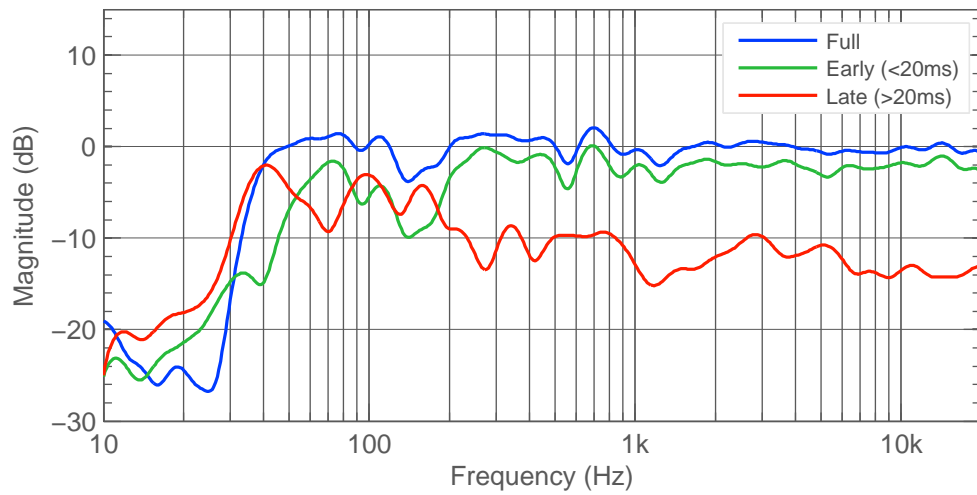
Figure 4.45: Right Side 8341A. Full, early and late frequency response.
