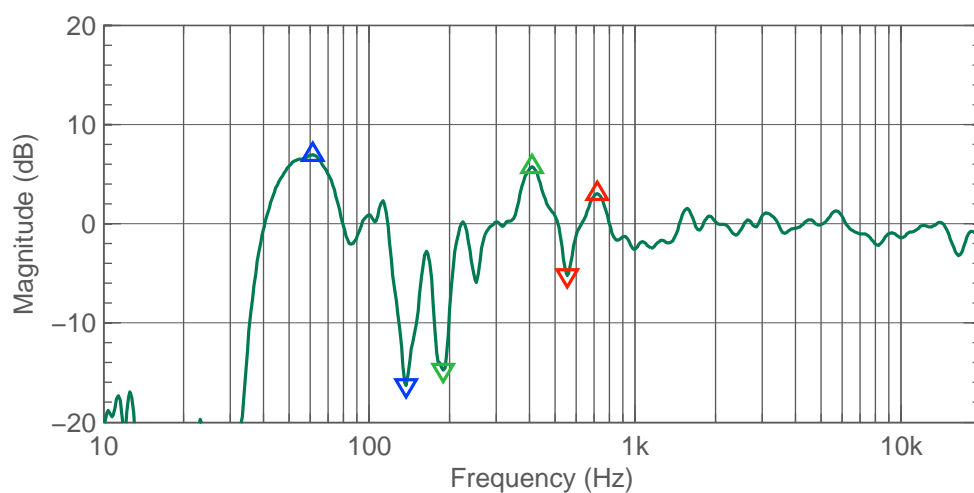
Figure 3.44: Right 8341A w peaks and notches (before calibration).
