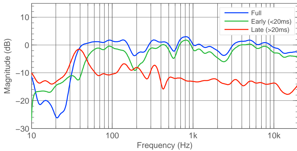
Figure 4.46: R Rear 8341A. Full, early and late frequency response.
