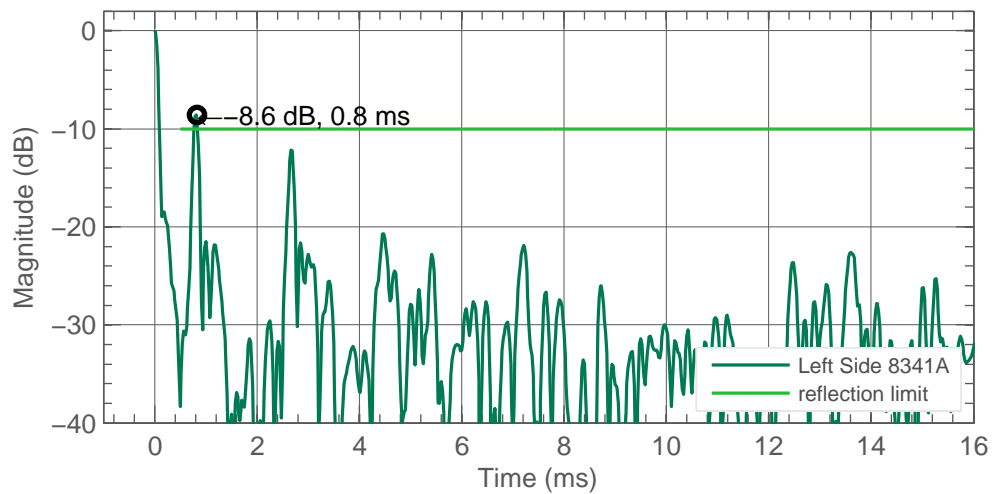
Figure 6.19: Early reflections. 1-8 kHz band. Level is relative to direct sound level.
