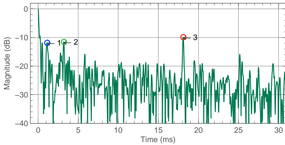
Figure 4.16: Center 8351B early reflections.
