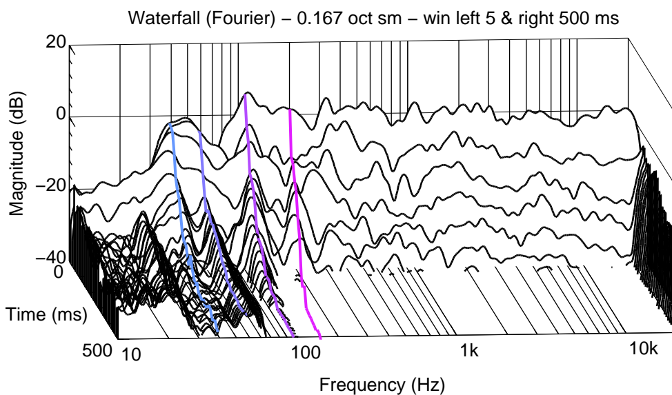
Figure 5.8: T R Front. Waterfall.
