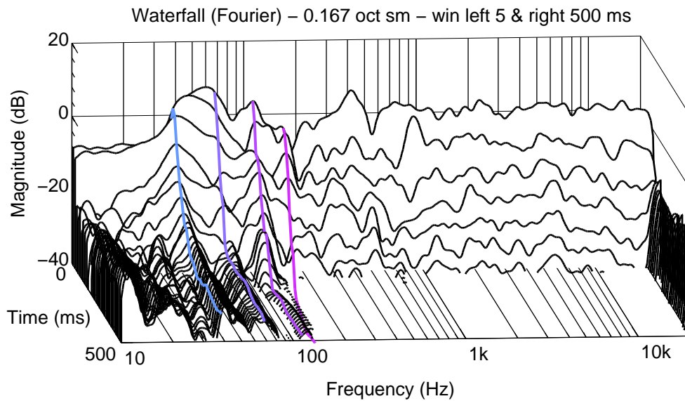
Figure 5.20: Left 8341A w. Waterfall.
