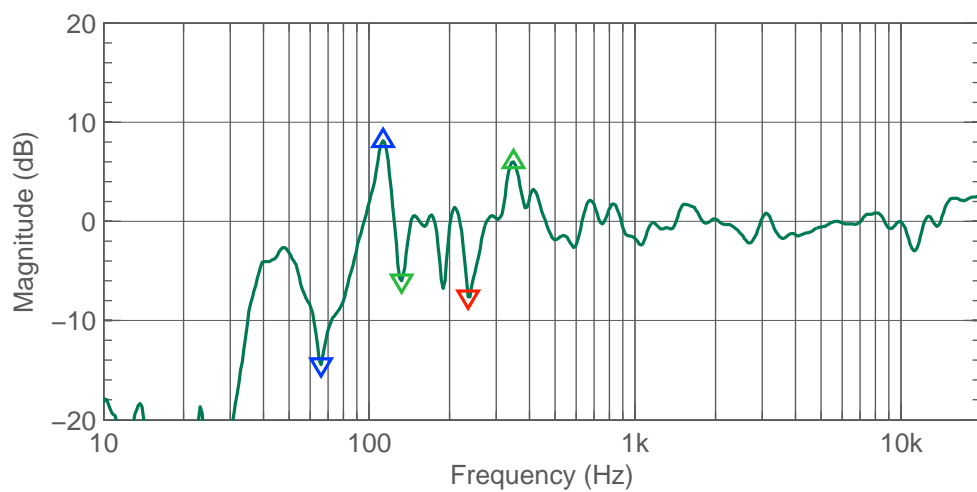
Figure 3.39: T L Mid peaks and notches (before calibration).
