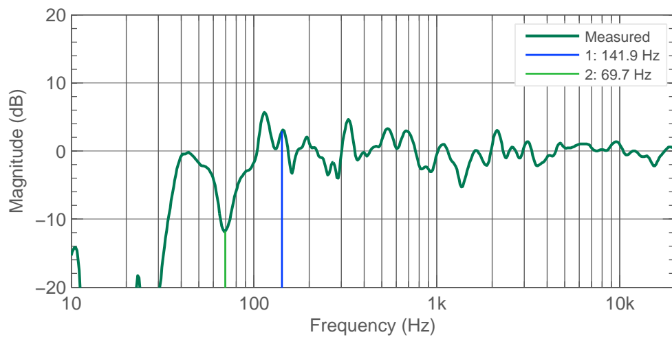
Figure 4.5: T L Front. Response and lowest cancellation frequency resulting from early reflection.
