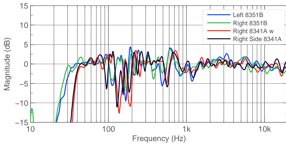
Figure 3.20: Frequency responses for monitors. AccuSmoothed.
