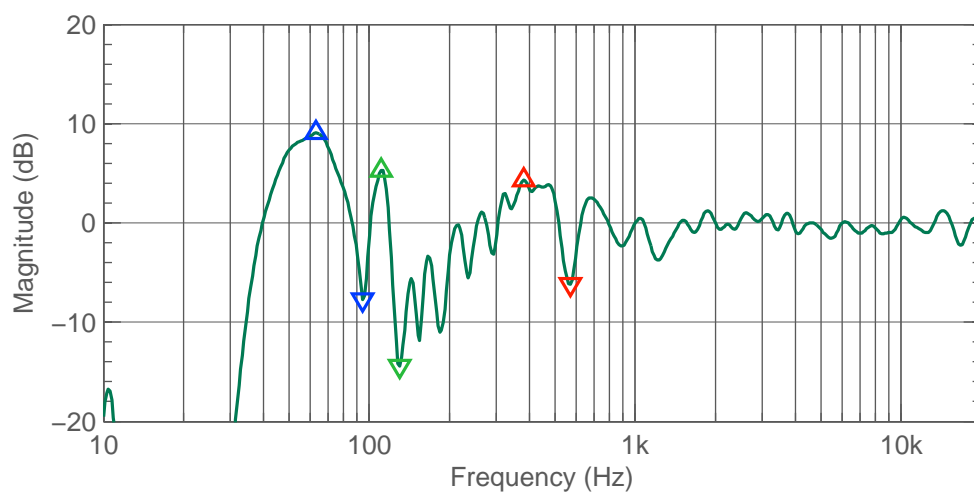
Figure 3.45: Right Side 8341A peaks and notches (before calibration).
