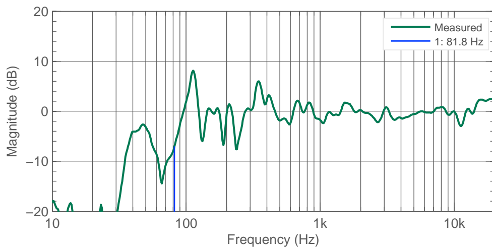
Figure 4.15: T L Mid. Response and lowest cancellation frequency resulting from early reflection.
