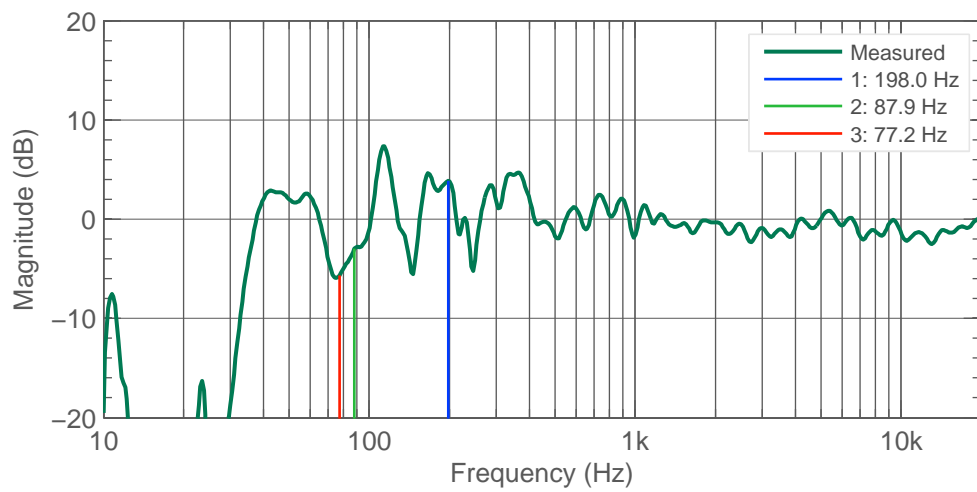
Figure 4.11: T R Rear. Response and lowest cancellation frequency resulting from early reflection.
