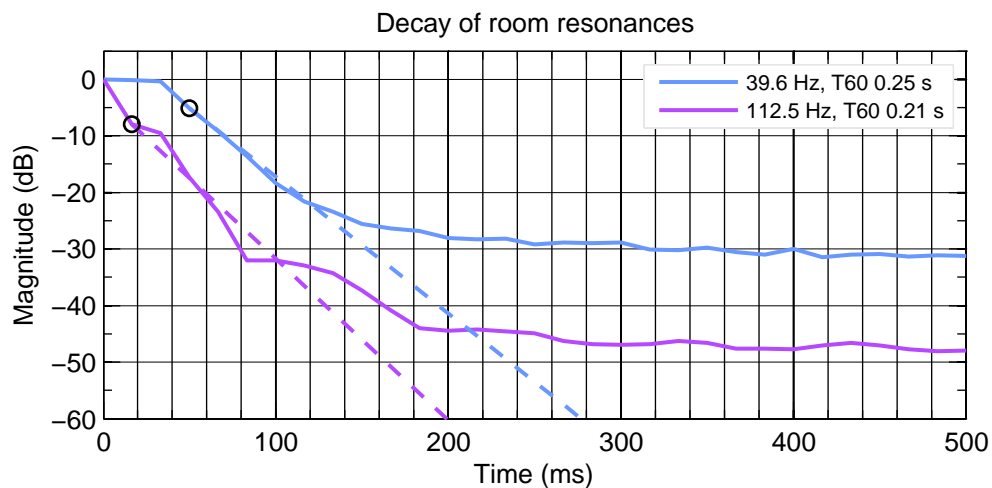
Figure 5.7: T L Front. Decay of detected resonances.
