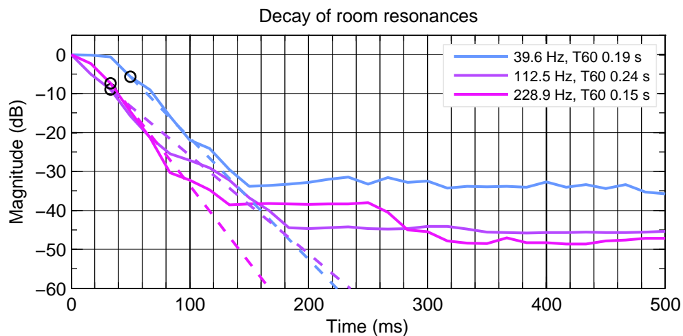
Figure 5.13: T R Rear. Decay of detected resonances.
