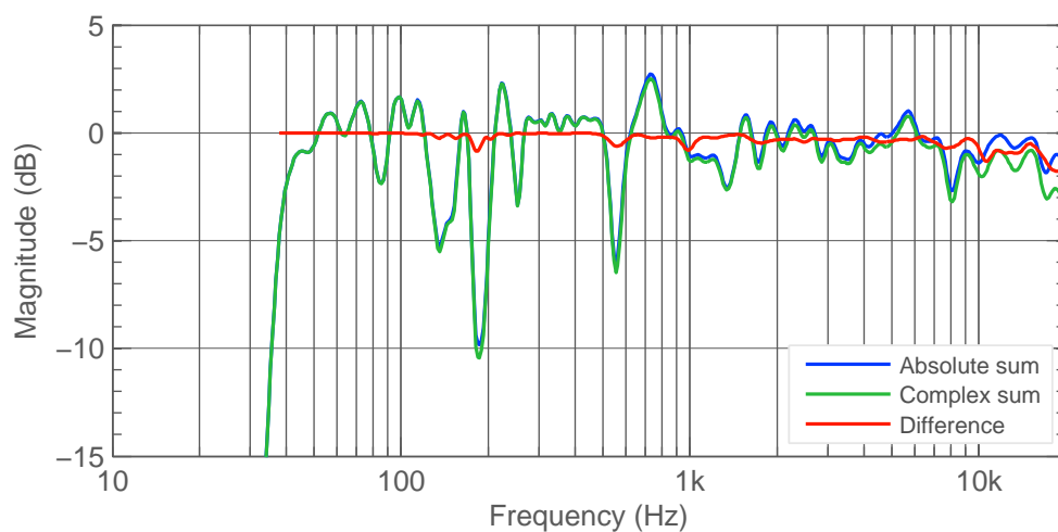
Figure 3.31: Difference between the sum of complex pressure and sum of absolute pressure. Calibration group ID 19.
