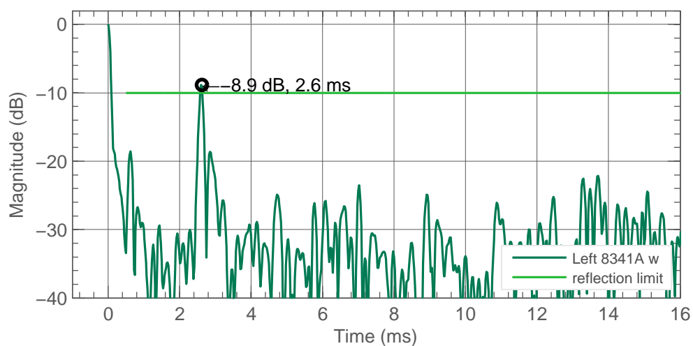
Figure 6.12: Early reflections. 1-8 kHz band. Level is relative to direct sound level.
