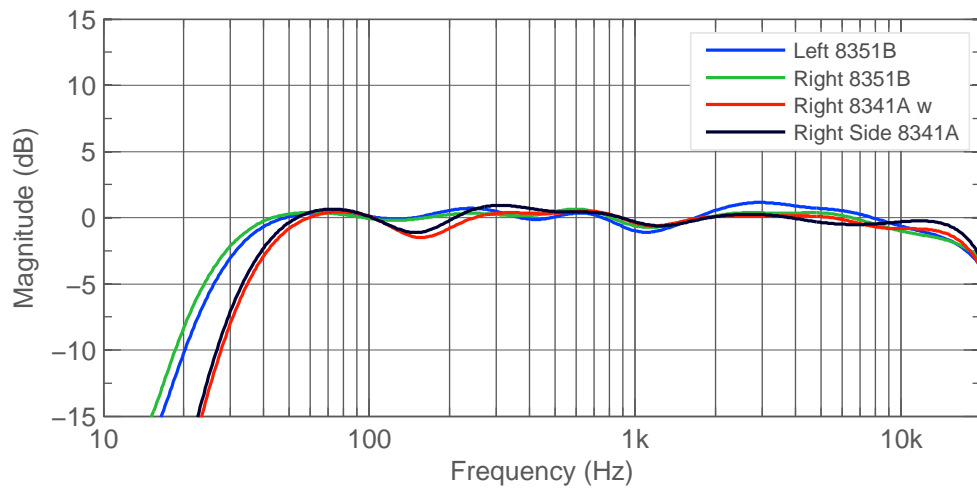
Figure 3.24: Frequency responses for monitors. One octave smoothing.
