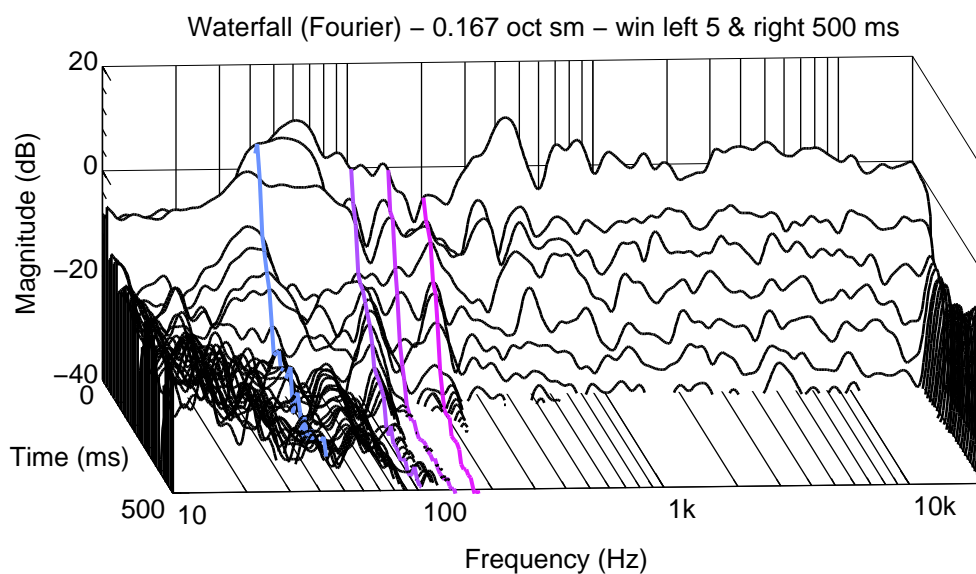
Figure 5.30: R Rear 8341A. Waterfall.
