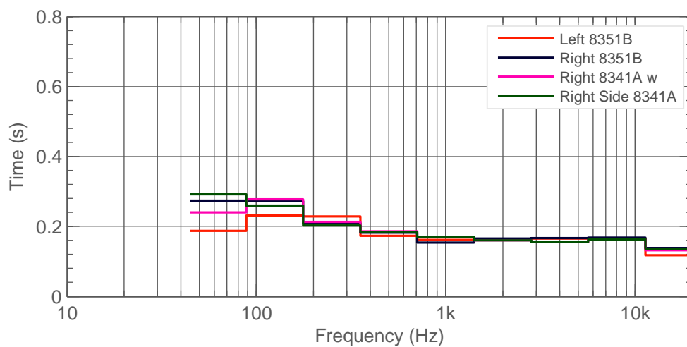
Figure 5.4: Decay time T_{60} , after calibration.
