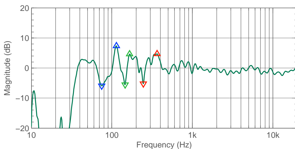
Figure 3.37: T R Rear peaks and notches (before calibration).
