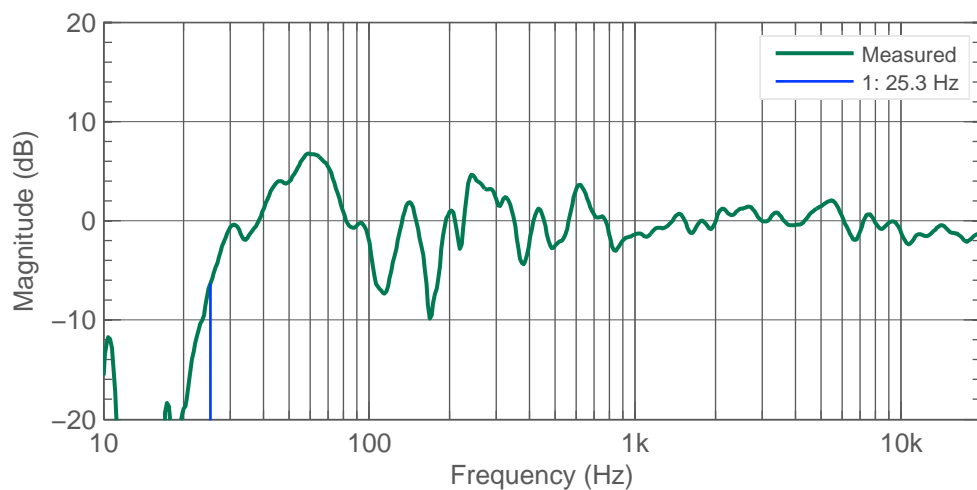
Figure 4.23: Right 8351B. Response and lowest cancellation frequency resulting from early reflection.
