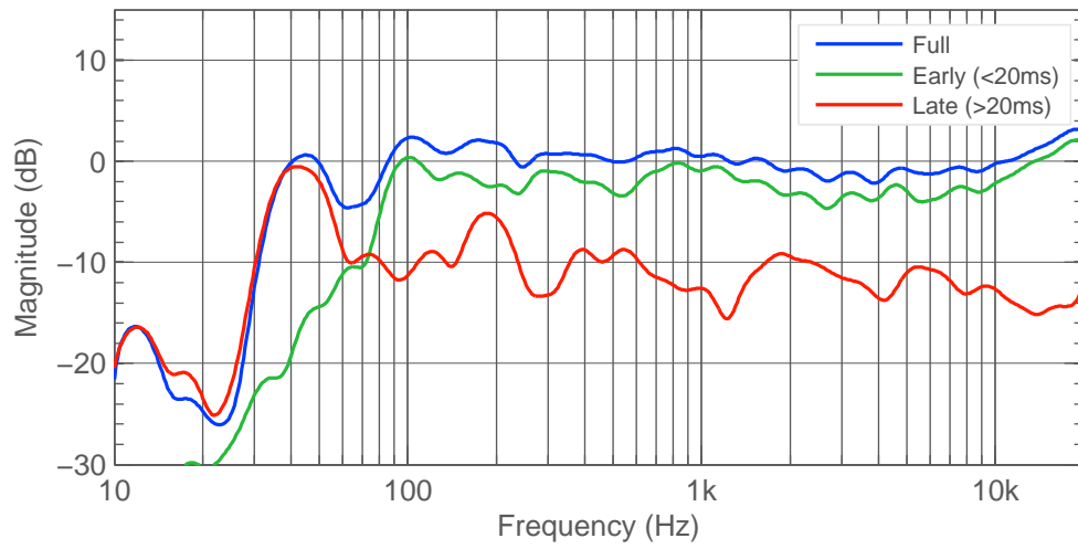
Figure 4.36: T R Mid. Full, early and late frequency response.
