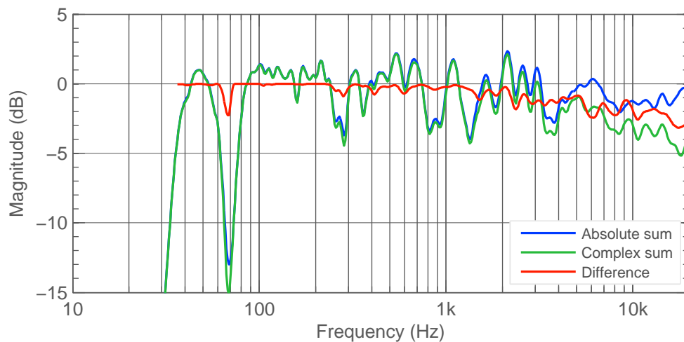
Figure 3.27: Difference between the sum of complex pressure and sum of absolute pressure. Calibration group ID 4.
