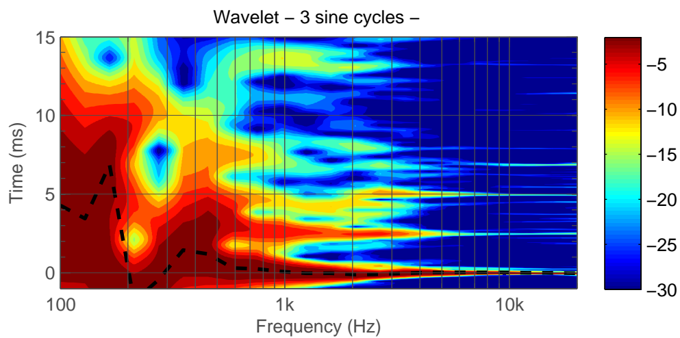
Figure 5.53: R Rear 8341A. Wavelet.
