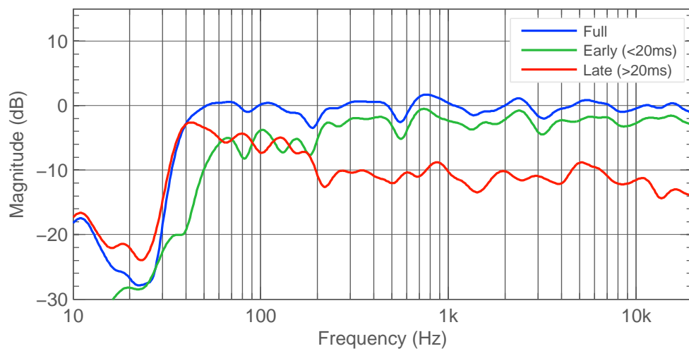
Figure 4.41: Left 8341A w. Full, early and late frequency response.
