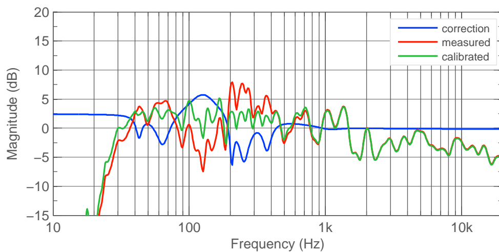
Figure 3.7: Center 8351B frequency response.
