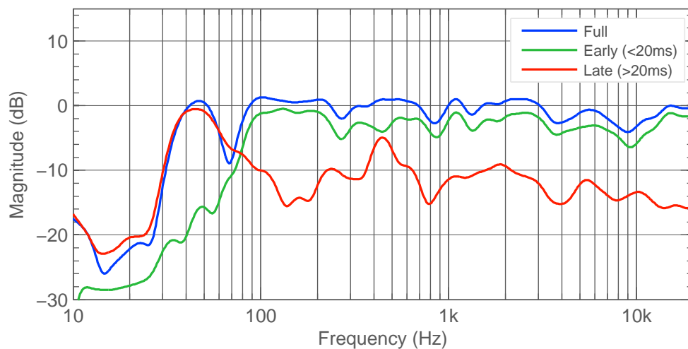
Figure 4.35: T R Front. Full, early and late frequency response.
