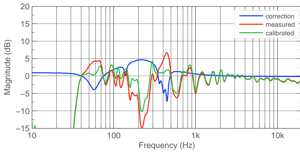
Figure 3.14: L Rear 8341A frequency response.
