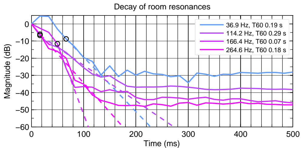
Figure 5.27: Right 8341A w. Decay of detected resonances.
