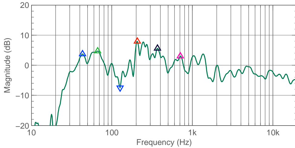
Figure 3.40: Center 8351B peaks and notches (before calibration).
