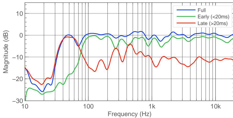
Figure 4.34: T L Front. Full, early and late frequency response.
