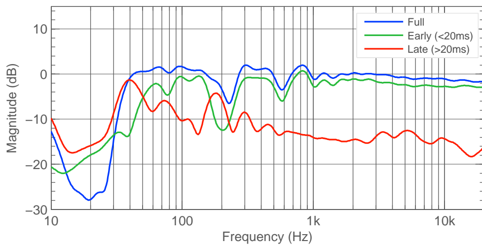
Figure 4.47: L Rear 8341A. Full, early and late frequency response.
