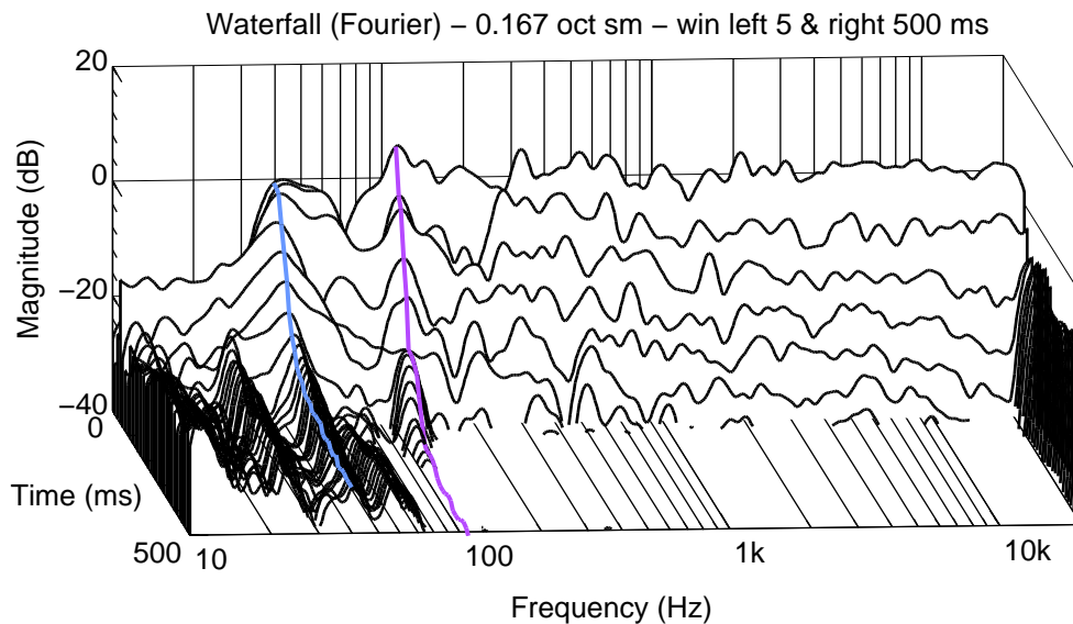
Figure 5.6: T L Front. Waterfall.
