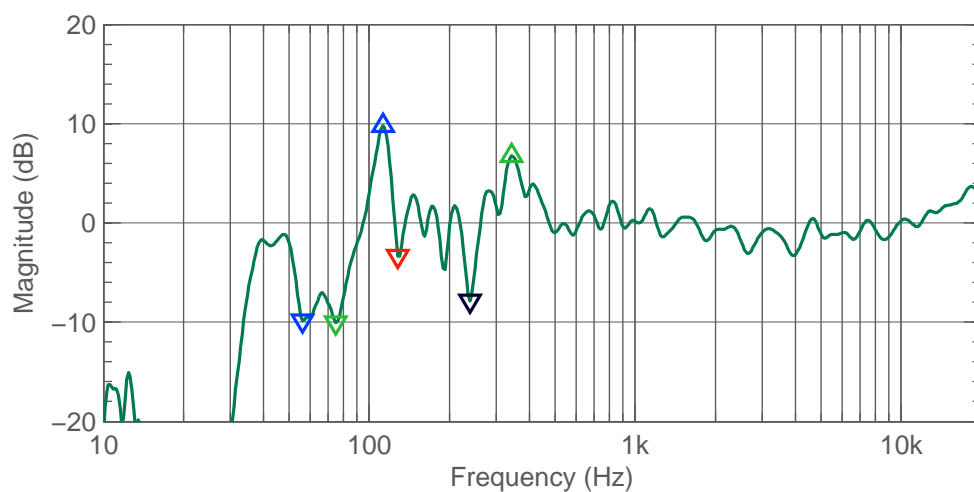
Figure 3.36: T R Mid peaks and notches (before calibration).
