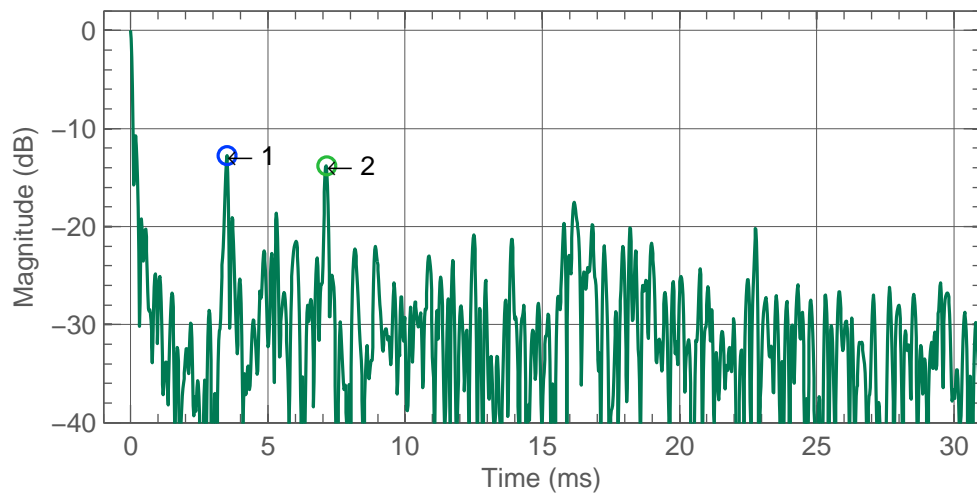
Figure 4.4: T L Front early reflections.
