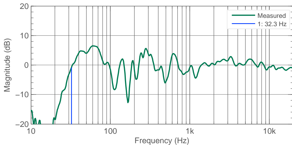
Figure 4.21: Left 8351B. Response and lowest cancellation frequency resulting from early reflection.
