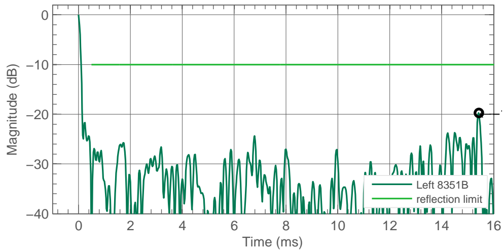
Figure 6.13: Early reflections. 1-8 kHz band. Level is relative to direct sound level.
