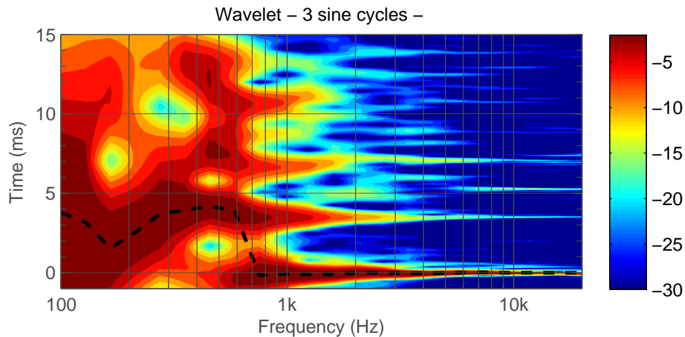
Figure 5.41: T L Front. Wavelet.
