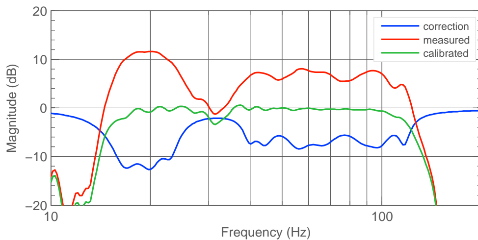
Figure 3.17: Left 7380A frequency response.
