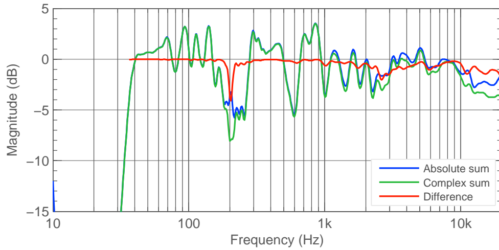
Figure 3.33: Difference between the sum of complex pressure and sum of absolute pressure. Calibration group ID 24.
