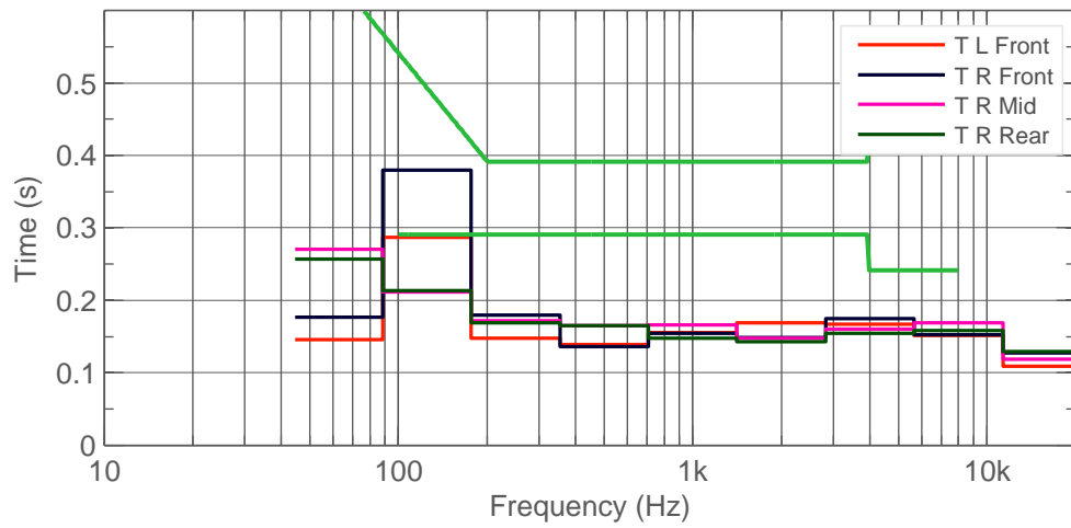
Figure 6.20: Decay time T60, after calibration. Target decay time T_m = 0.34 s (based on calculated room volume).
