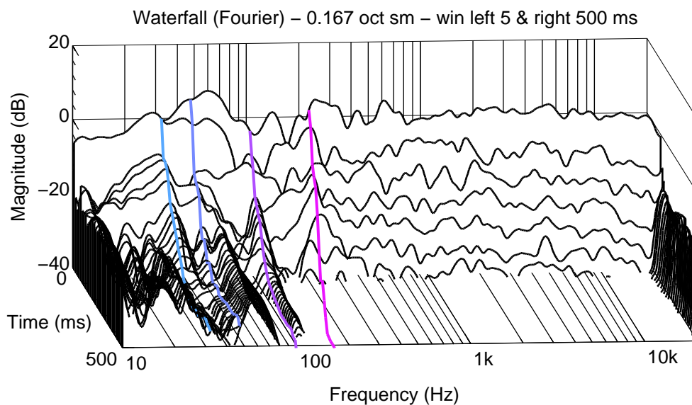
Figure 5.24: Right 8351B. Waterfall.
