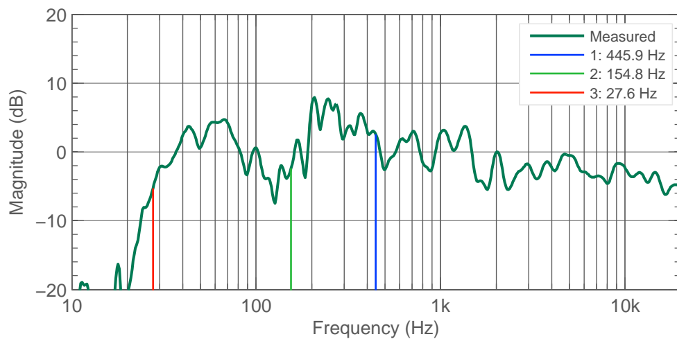
Figure 4.17: Center 8351B. Response and lowest cancellation frequency resulting from early reflection.
