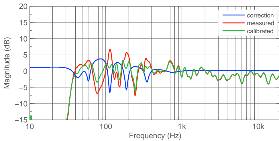
Figure 3.5: T L Rear frequency response.
