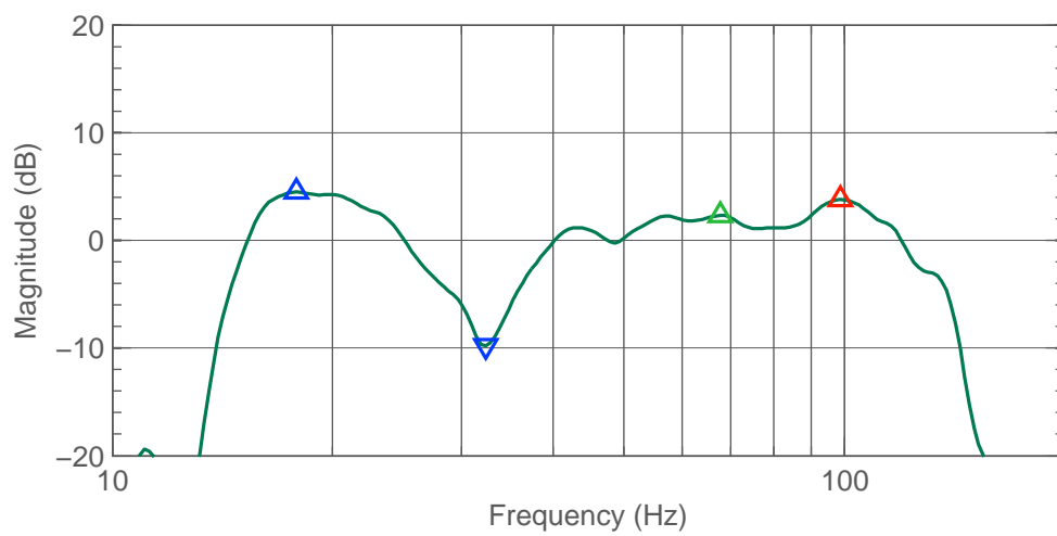
Figure 3.49: Right 7370A peaks and notches (before calibration).
