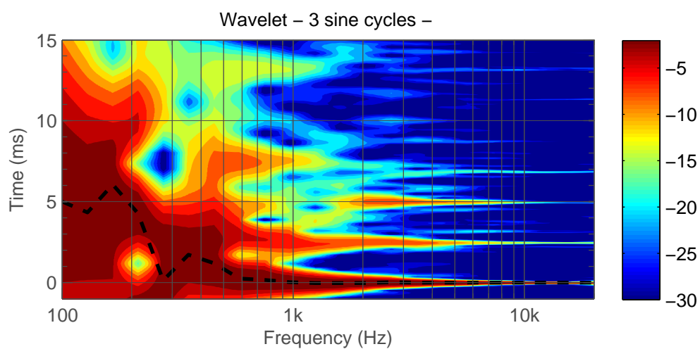
Figure 5.54: L Rear 8341A. Wavelet.
