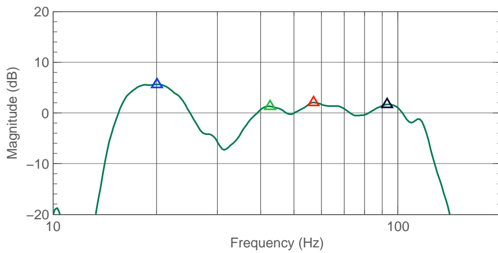
Figure 3.50: Left 7380A peaks and notches (before calibration).
