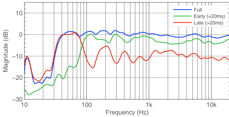
Figure 4.37: T R Rear. Full, early and late frequency response.
