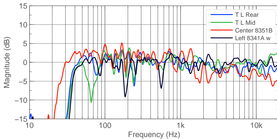
Figure 3.19: Frequency responses for monitors. AccuSmoothed.
