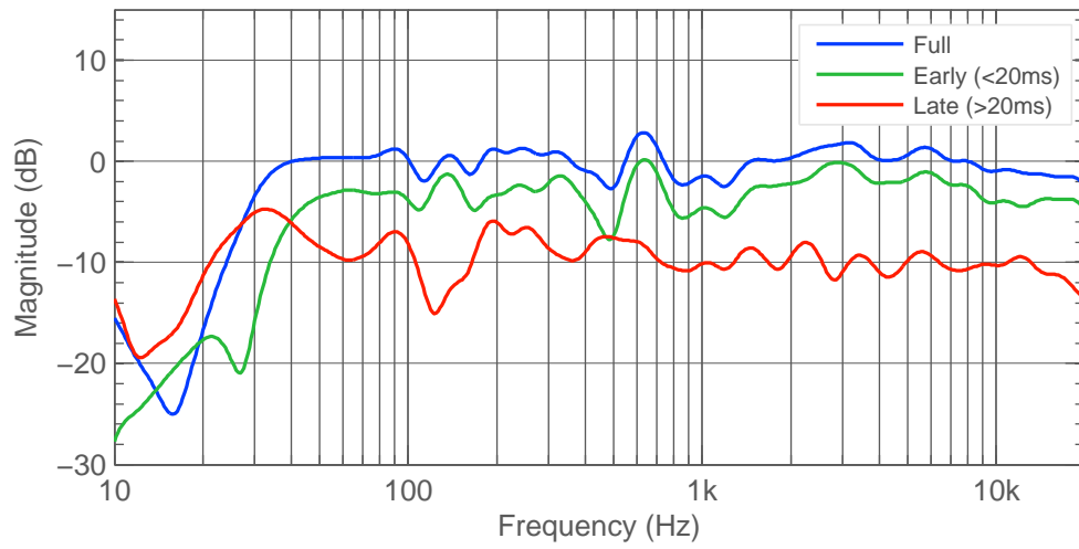
Figure 4.42: Left 8351B. Full, early and late frequency response.
