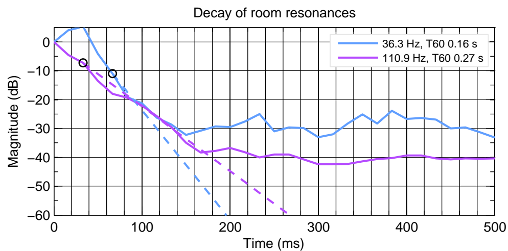
Figure 5.29: Right Side 8341A. Decay of detected resonances.
