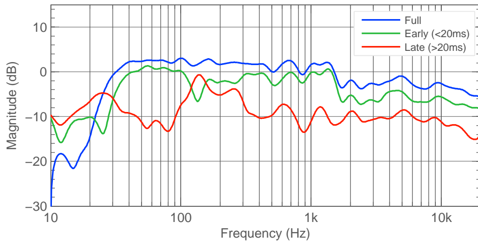
Figure 4.40: Center 8351B. Full, early and late frequency response.
