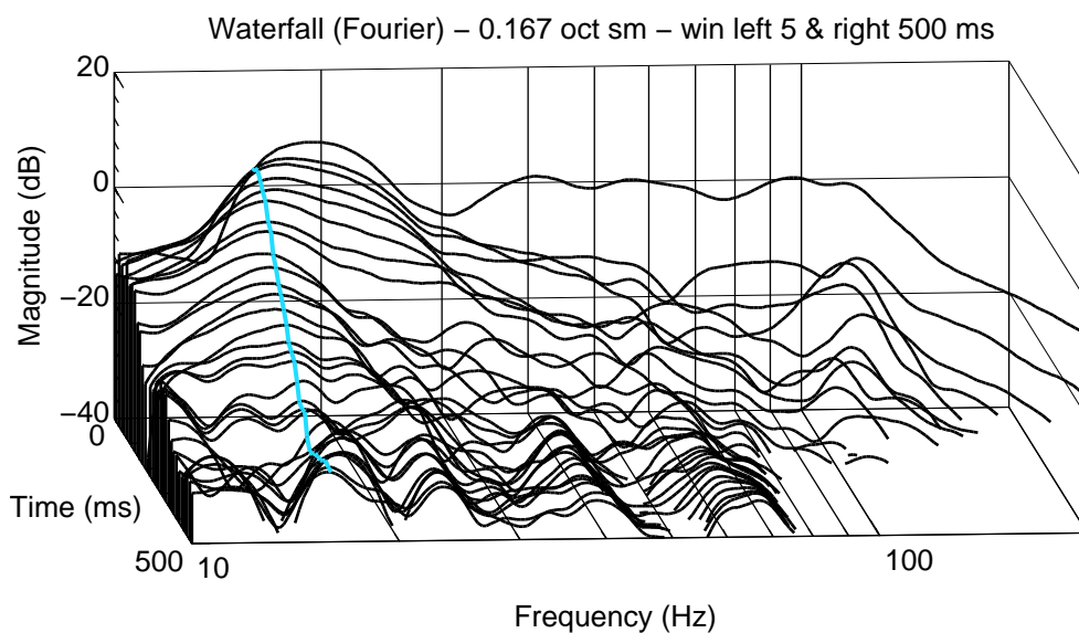
Figure 5.38: Left 7380A. Waterfall.
