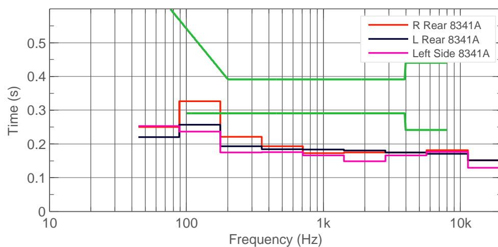
Figure 6.23: Decay time T60, after calibration. Target decay time T_m = 0.34 s (based on calculated room volume).
