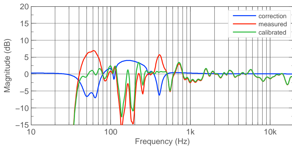
Figure 3.11: Right 8341A w frequency response.
