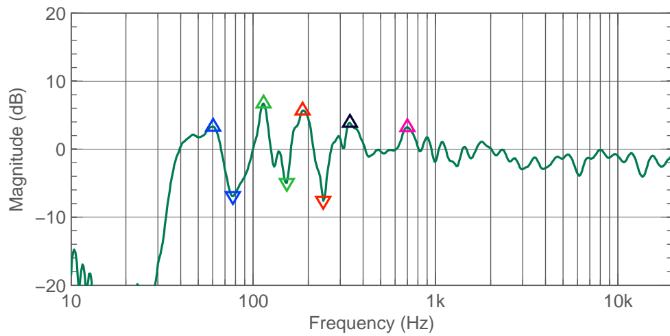
Figure 3.38: T L Rear peaks and notches (before calibration).
