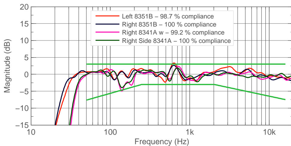
Figure 6.3: Operational room response curve.
