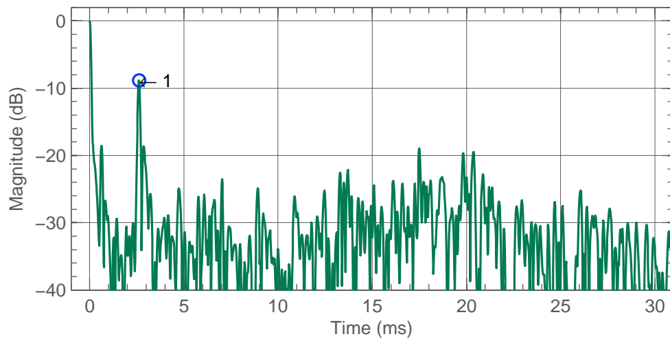
Figure 4.18: Left 8341A w early reflections.
