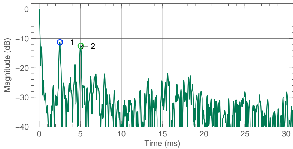
Figure 4.28: R Rear 8341A early reflections.
