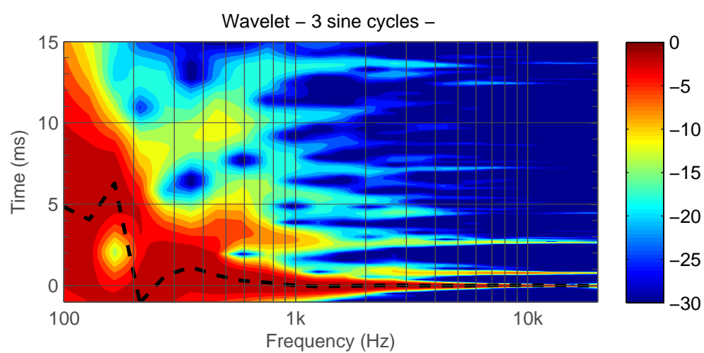
Figure 5.55: Left Side 8341A. Wavelet.
