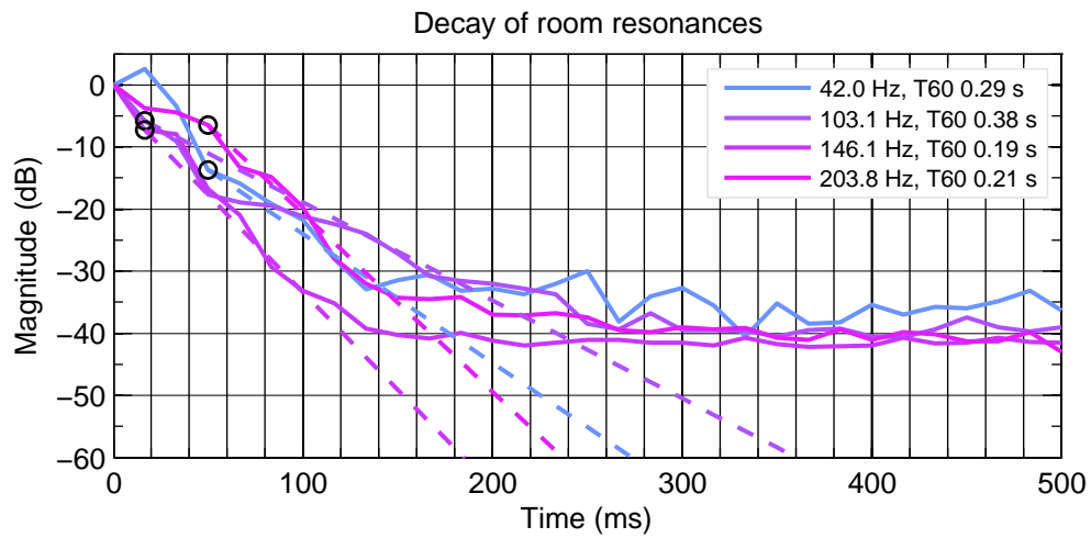
Figure 5.31: R Rear 8341A. Decay of detected resonances.
