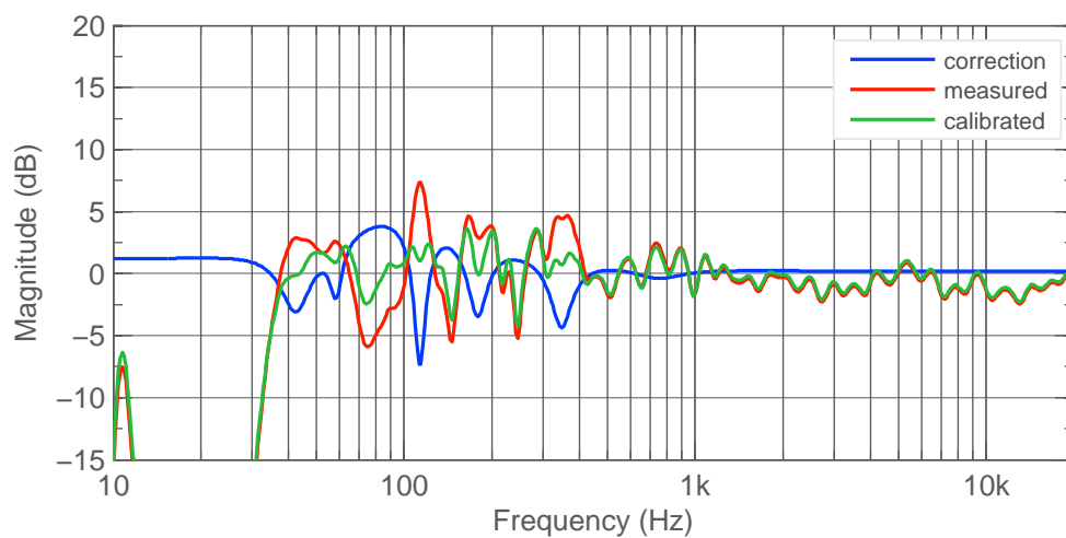
Figure 3.4: T R Rear frequency response.
