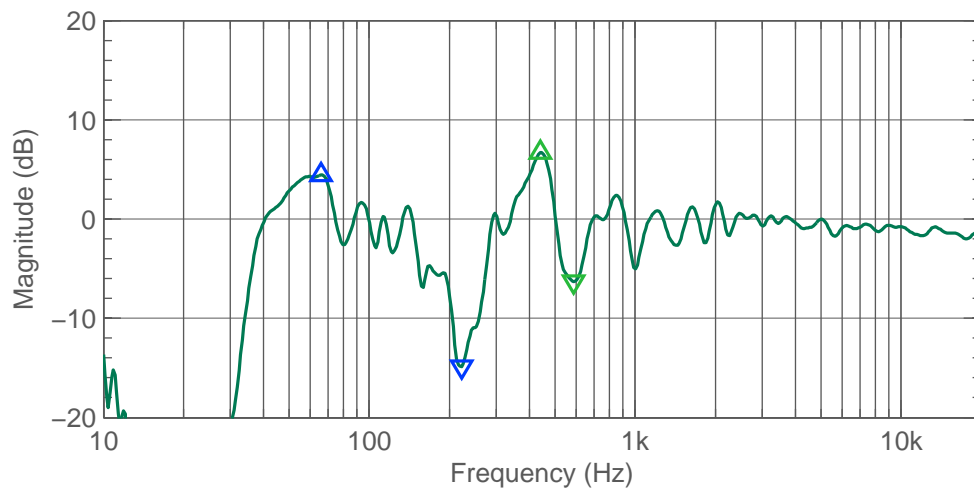
Figure 3.47: L Rear 8341A peaks and notches (before calibration).
