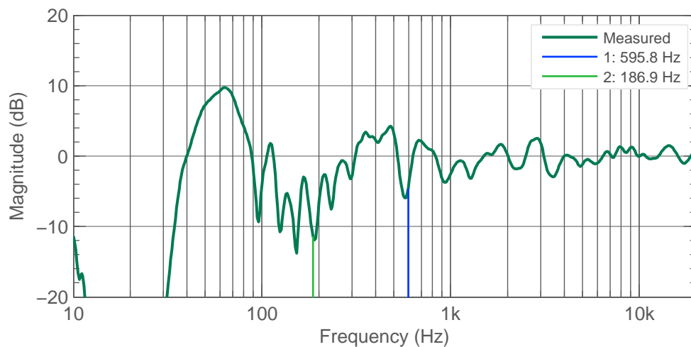
Figure 4.33: Left Side 8341A. Response and lowest cancellation frequency resulting from early reflection.
