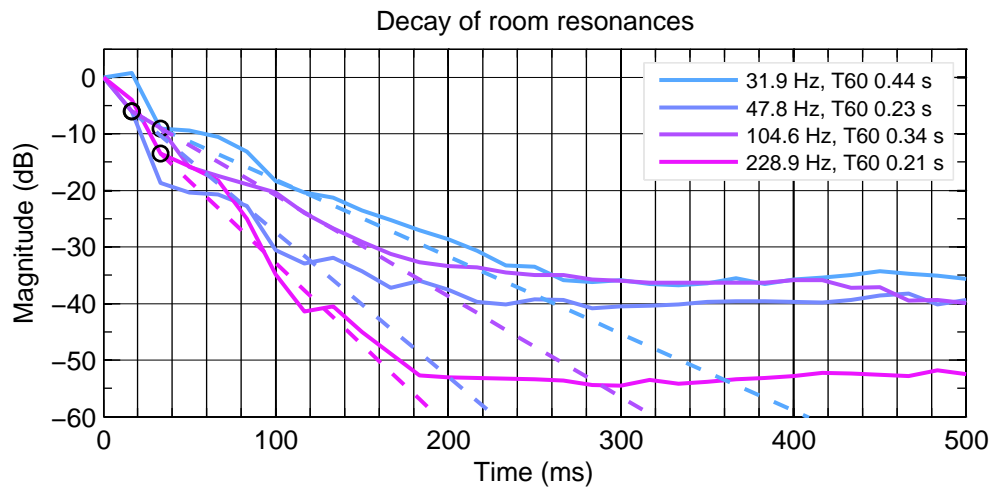
Figure 5.25: Right 8351B. Decay of detected resonances.
