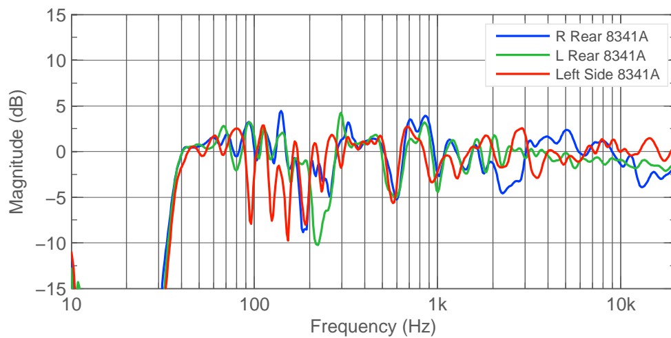
Figure 3.21: Frequency responses for monitors. AccuSmoothed.
