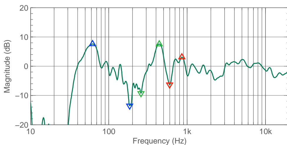
Figure 3.46: R Rear 8341A peaks and notches (before calibration).
