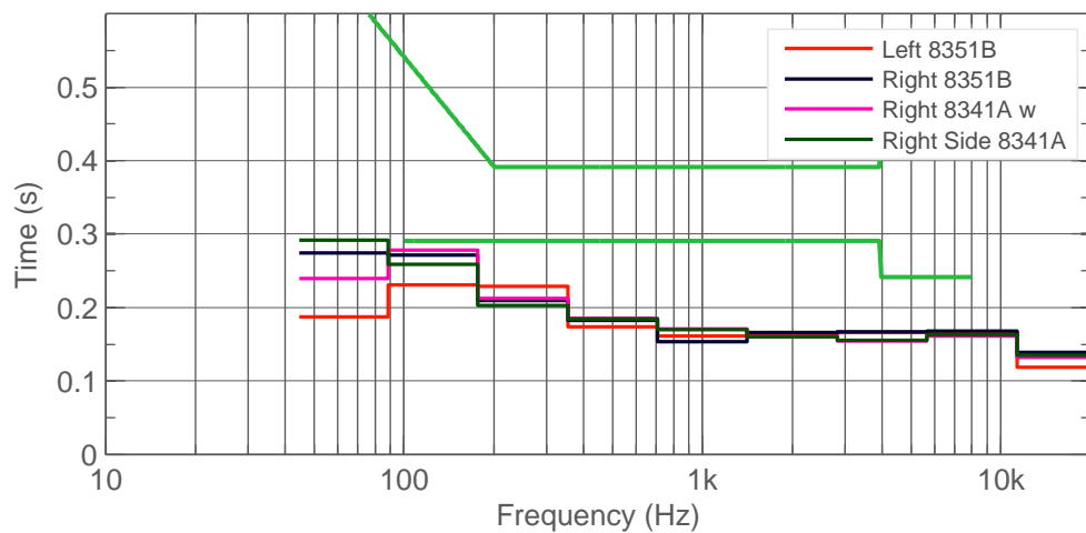
Figure 6.22: Decay time T60, after calibration. Target decay time T_m = 0.34 s (based on calculated room volume).
