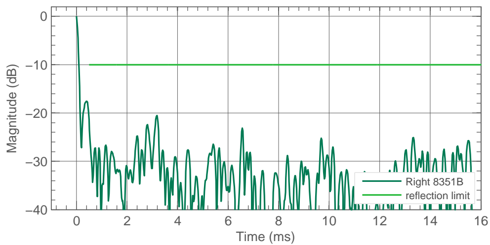
Figure 6.14: Early reflections. 1-8 kHz band. Level is relative to direct sound level.
