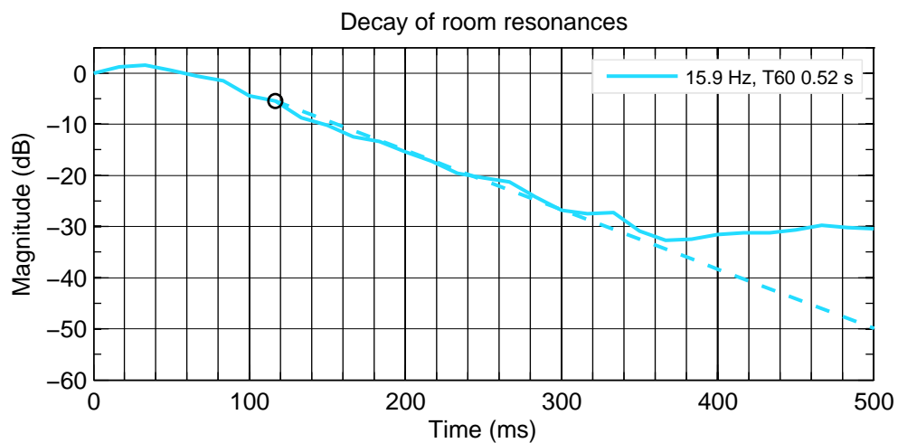
Figure 5.39: Left 7380A. Decay of detected resonances.
