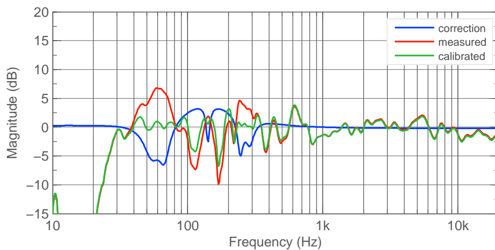
Figure 3.10: Right 8351B frequency response.
