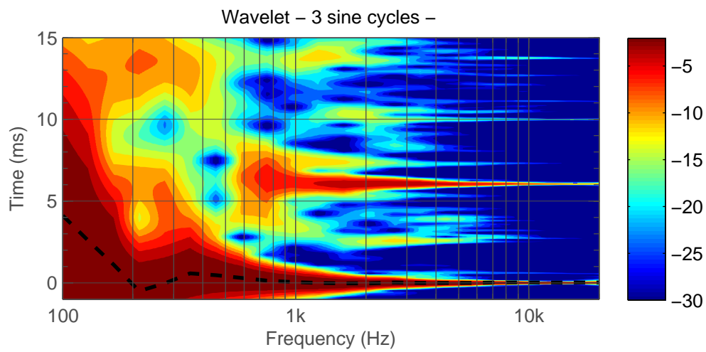
Figure 5.46: T L Mid. Wavelet.
