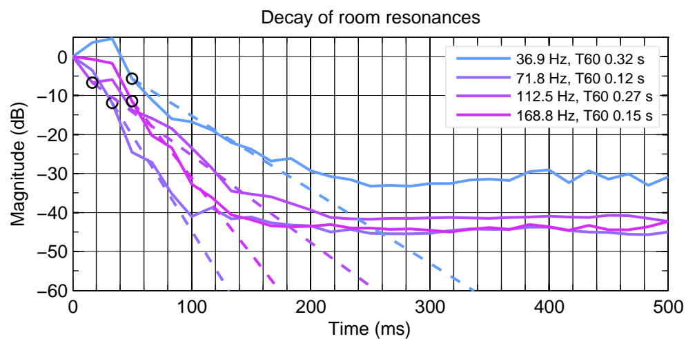
Figure 5.35: Left Side 8341A. Decay of detected resonances.
