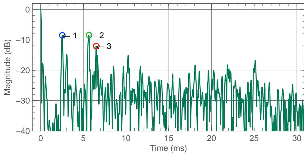
Figure 4.10: T R Rear early reflections.
