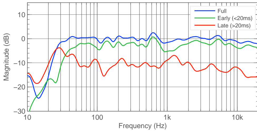
Figure 4.43: Right 8351B. Full, early and late frequency response.
