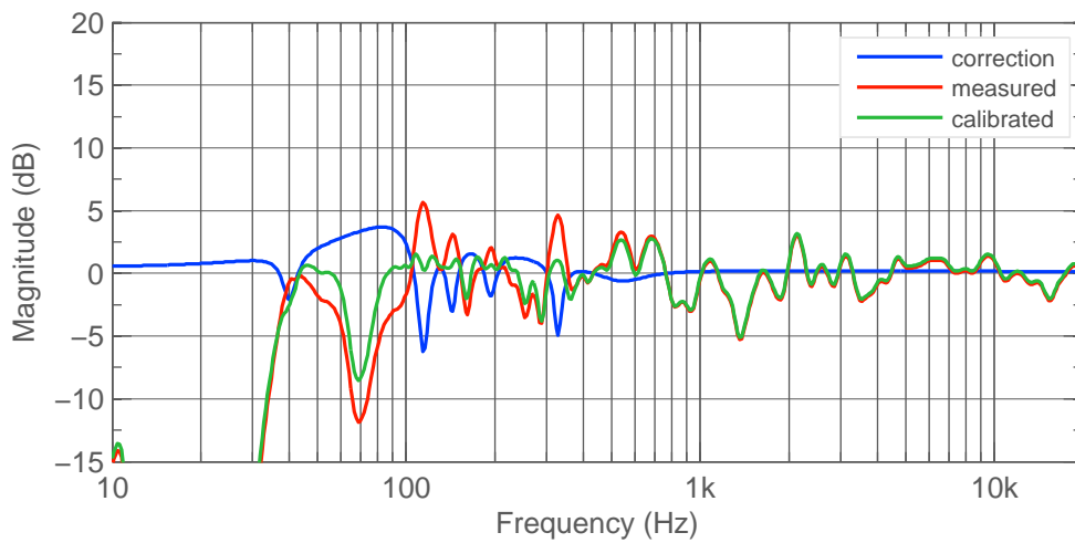
Figure 3.1: T L Front frequency response.
