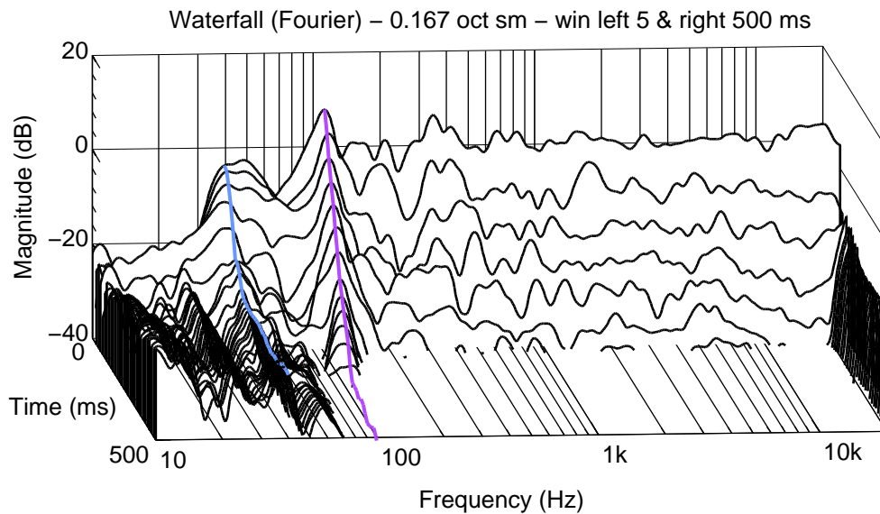
Figure 5.16: T L Mid. Waterfall.
