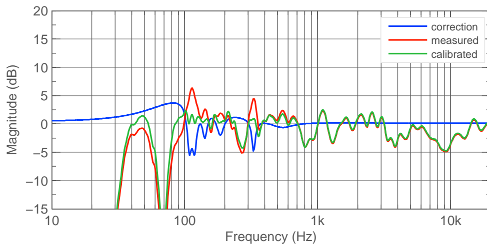
Figure 3.2: T R Front frequency response.
