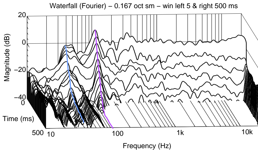
Figure 5.10: T R Mid. Waterfall.
