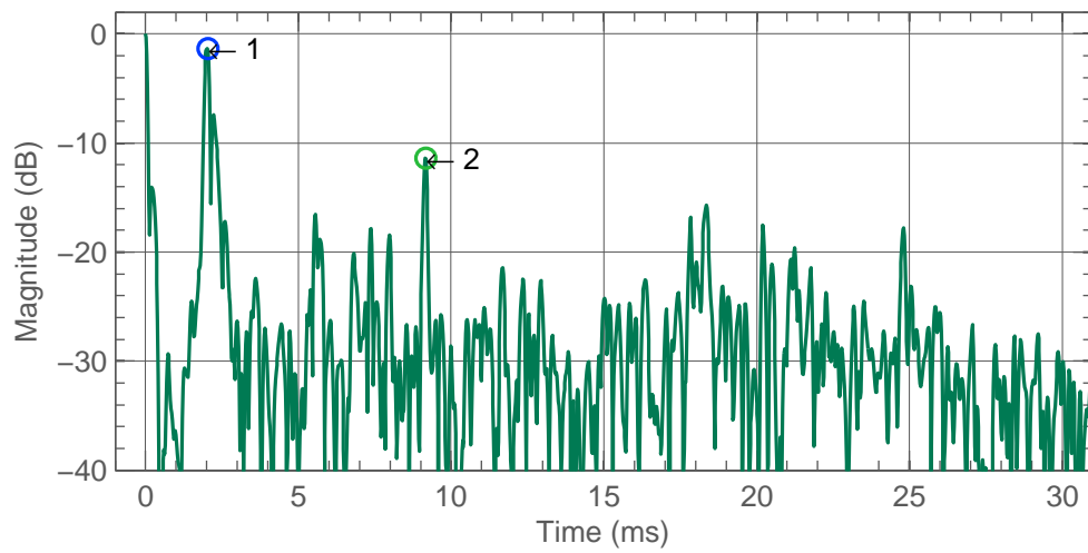
Figure 4.6: T R Front early reflections.
