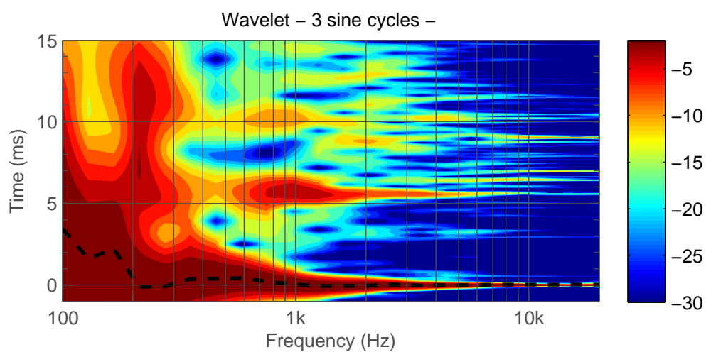
Figure 5.45: T L Rear. Wavelet.
