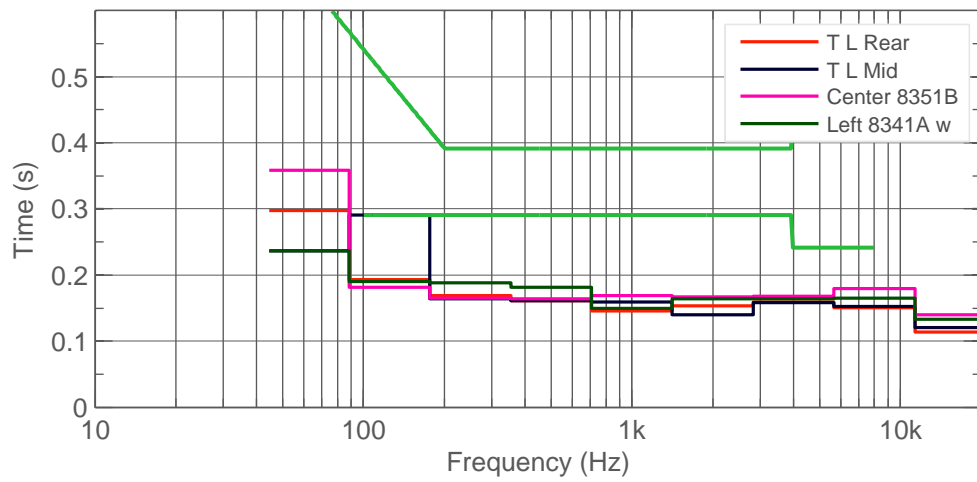
Figure 6.21: Decay time T60, after calibration. Target decay time T_m = 0.34 s (based on calculated room volume).
