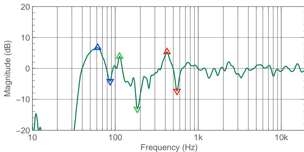
Figure 3.41: Left 8341A w peaks and notches (before calibration).
