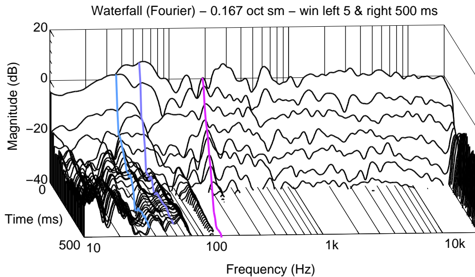
Figure 5.22: Left 8351B. Waterfall.
