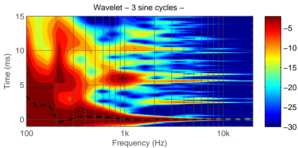
Figure 5.44: T R Rear. Wavelet.
