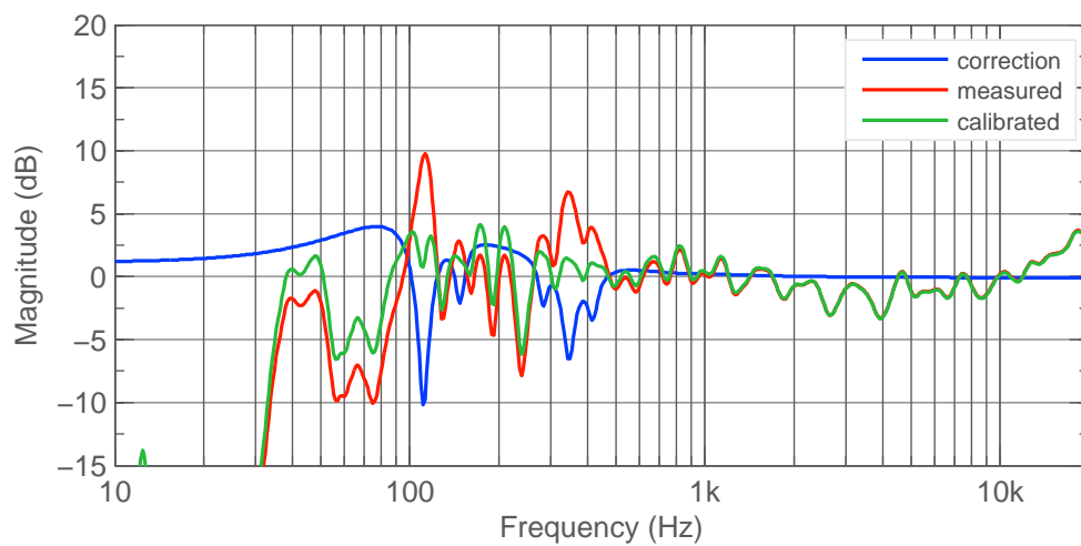
Figure 3.3: T R Mid frequency response.
