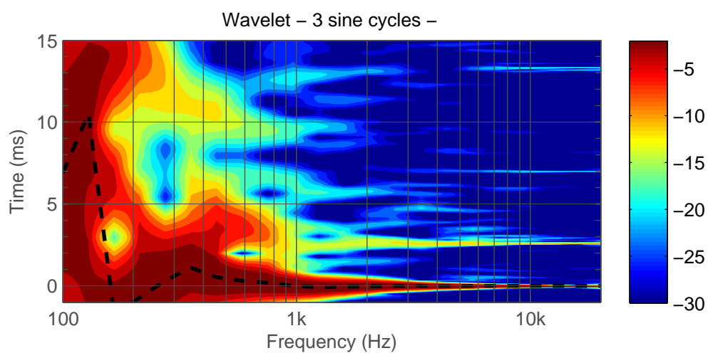
Figure 5.51: Right 8341A w. Wavelet.
