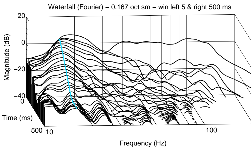
Figure 5.36: Right 7370A. Waterfall.
