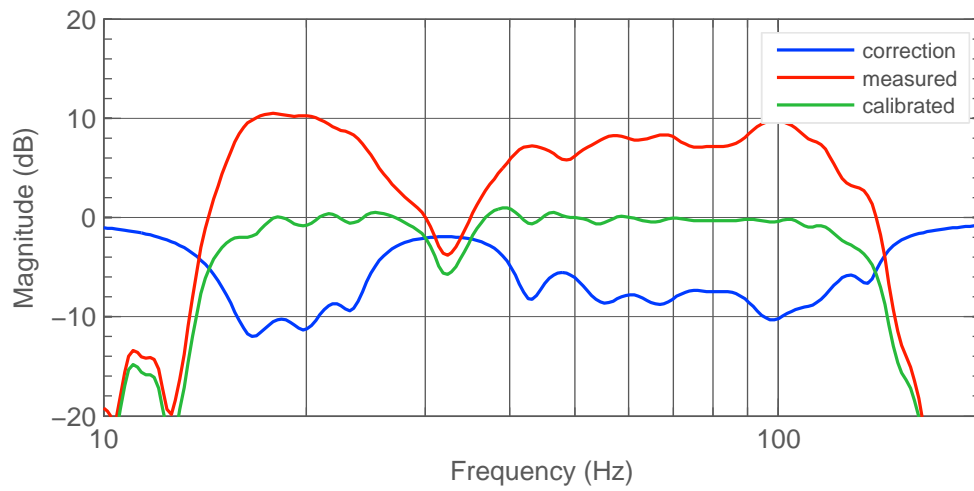
Figure 3.16: Right 7370A frequency response.
