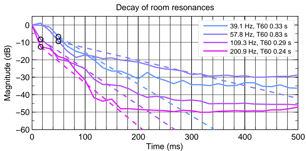
Figure 5.9: T R Front. Decay of detected resonances.
