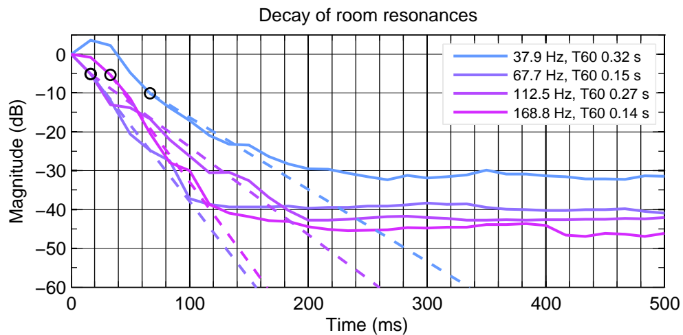
Figure 5.21: Left 8341A w. Decay of detected resonances.
