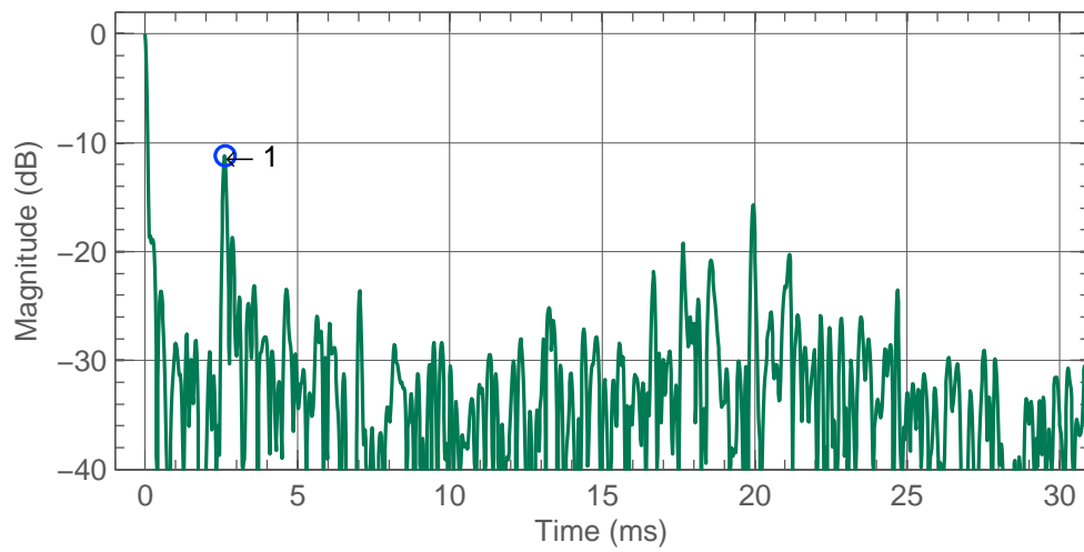
Figure 4.24: Right 8341A w early reflections.
