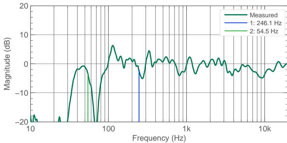
Figure 4.7: T R Front. Response and lowest cancellation frequency resulting from early reflection.
