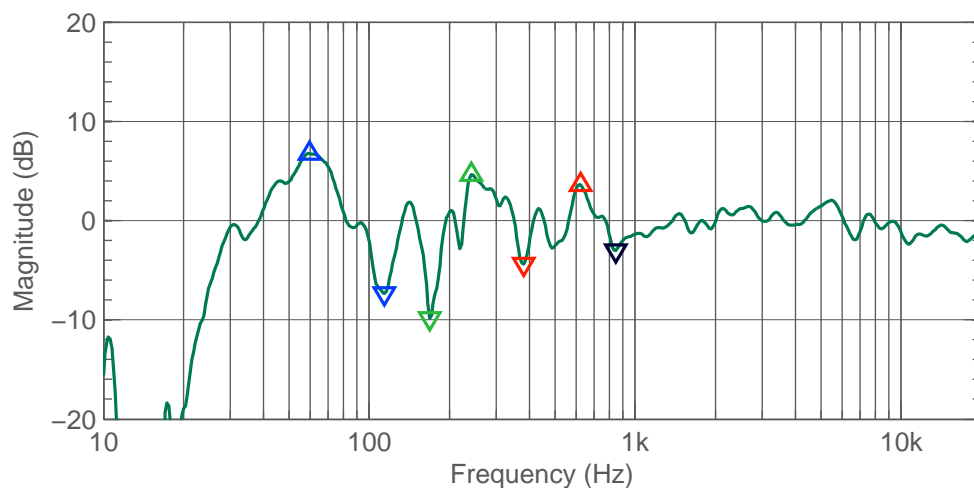
Figure 3.43: Right 8351B peaks and notches (before calibration).
