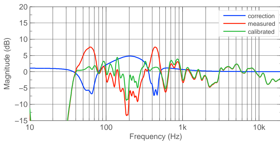
Figure 3.13: R Rear 8341A frequency response.
