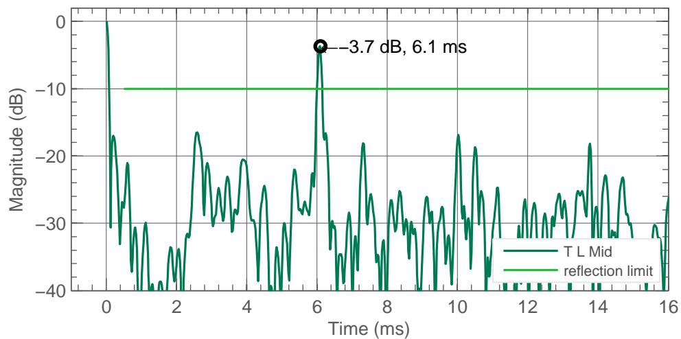
Figure 6.10: Early reflections. 1-8 kHz band. Level is relative to direct sound level.
