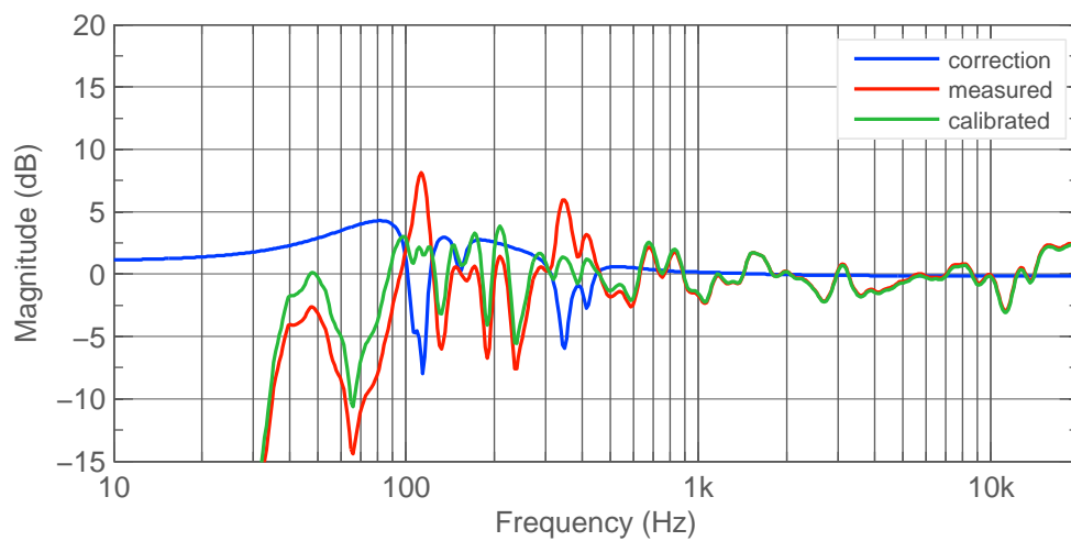
Figure 3.6: T L Mid frequency response.
