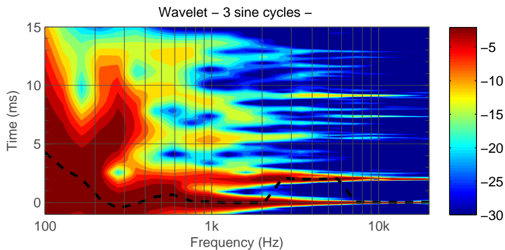
Figure 5.42: T R Front. Wavelet.
