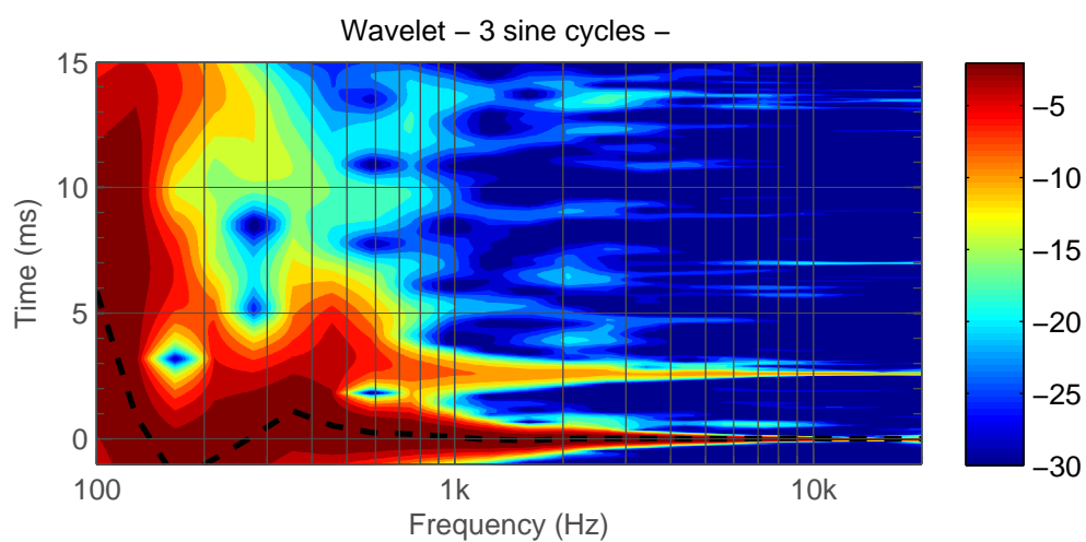
Figure 5.48: Left 8341A w. Wavelet.
