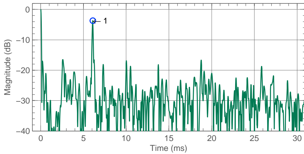
Figure 4.14: T L Mid early reflections.
