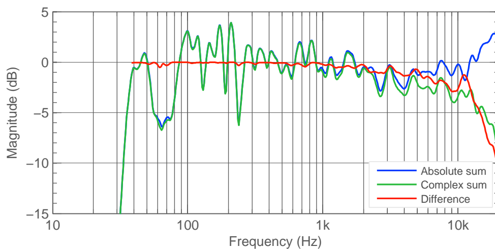
Figure 3.28: Difference between the sum of complex pressure and sum of absolute pressure. Calibration group ID 5.
