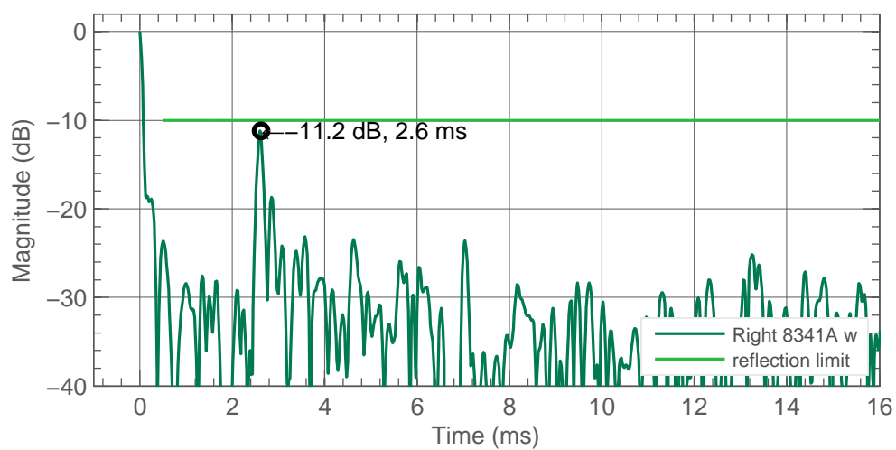
Figure 6.15: Early reflections. 1-8 kHz band. Level is relative to direct sound level.
