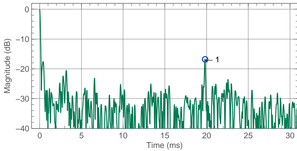
Figure 4.22: Right 8351B early reflections.
