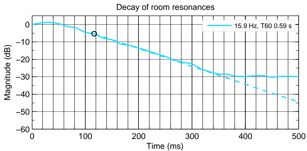
Figure 5.37: Right 7370A. Decay of detected resonances.
