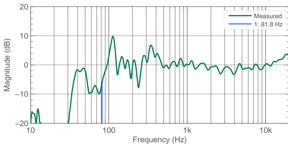
Figure 4.9: T R Mid. Response and lowest cancellation frequency resulting from early reflection.
