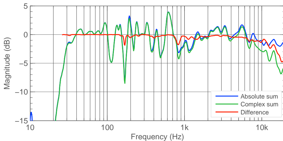
Figure 3.30: Difference between the sum of complex pressure and sum of absolute pressure. Calibration group ID 18.
