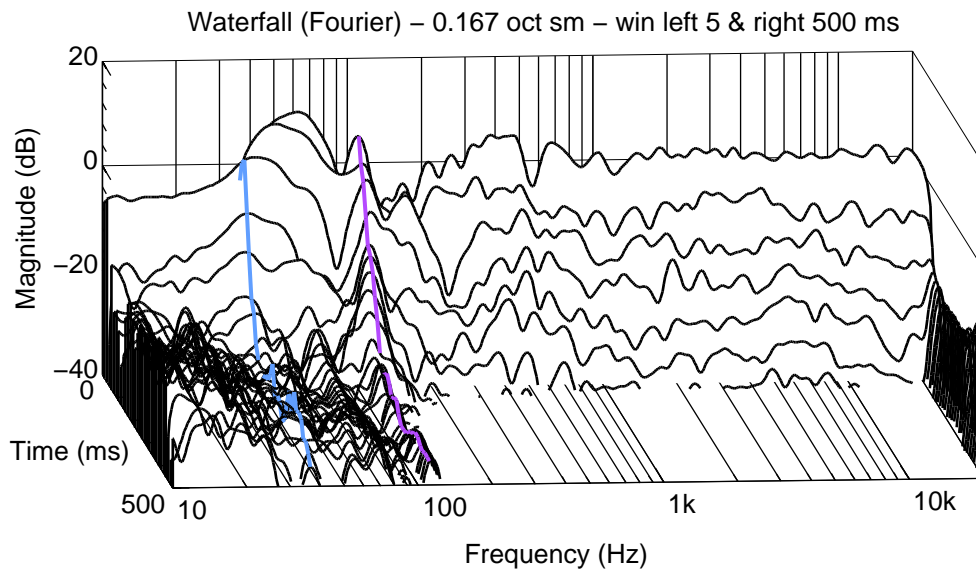
Figure 5.28: Right Side 8341A. Waterfall.
