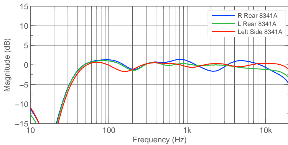
Figure 3.25: Frequency responses for monitors. One octave smoothing.
