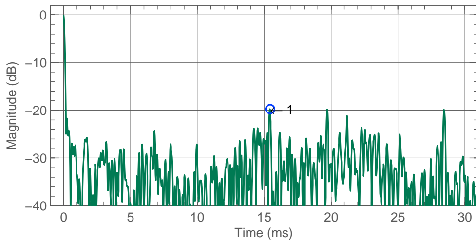
Figure 4.20: Left 8351B early reflections.
