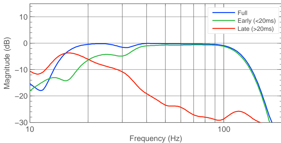
Figure 4.50: Left 7380A. Full, early and late frequency response.
