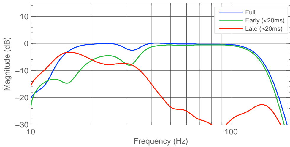
Figure 4.49: Right 7370A. Full, early and late frequency response.
