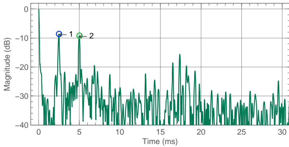
Figure 4.30: L Rear 8341A early reflections.
