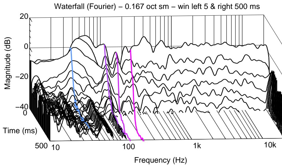
Figure 5.26: Right 8341A w. Waterfall.
