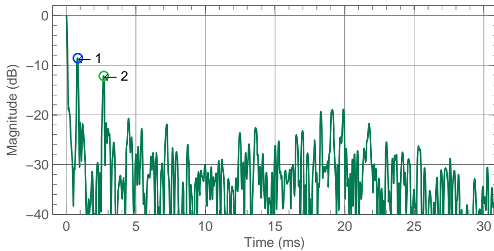
Figure 4.32: Left Side 8341A early reflections.
