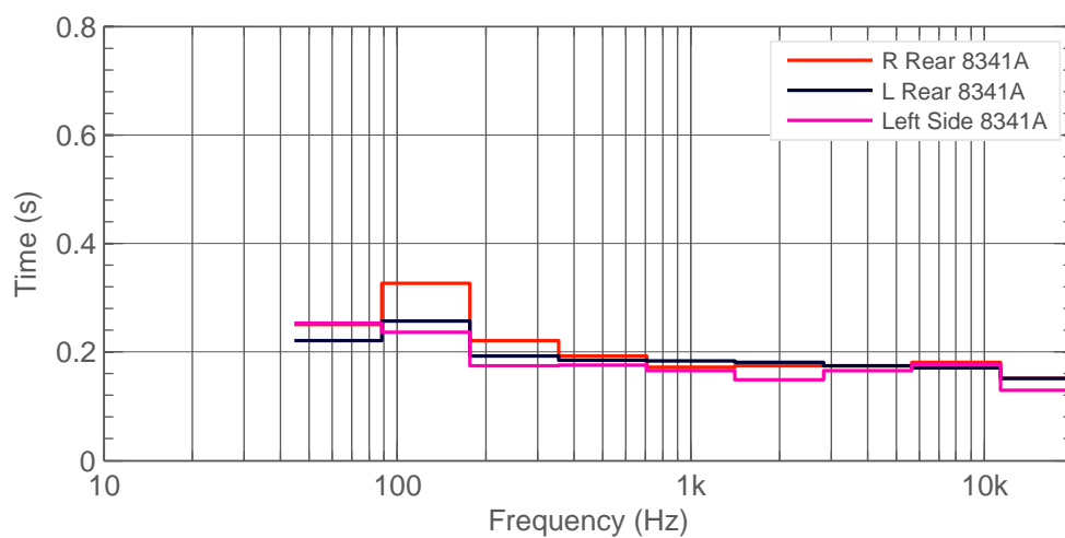
Figure 5.5: Decay time T60, after calibration.
