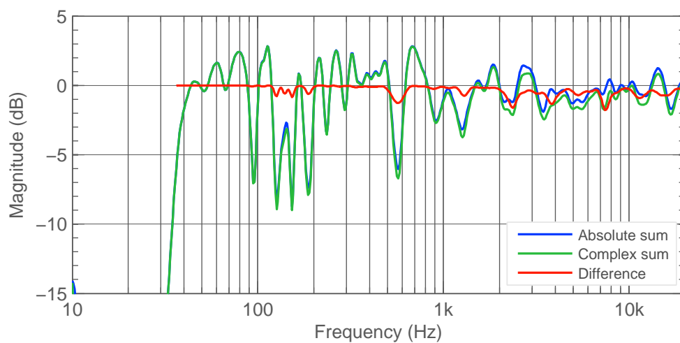
Figure 3.32: Difference between the sum of complex pressure and sum of absolute pressure. Calibration group ID 21.
