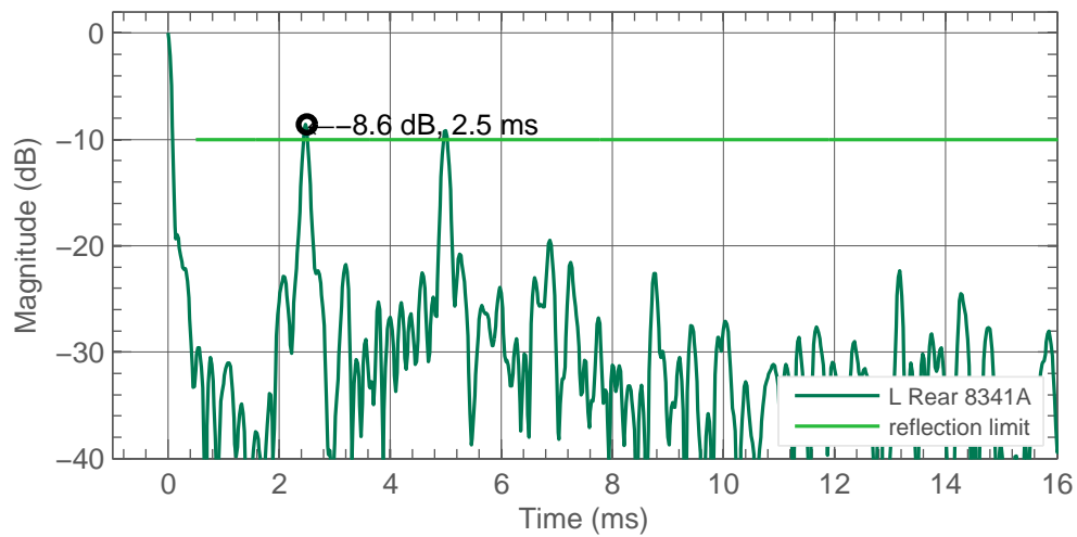
Figure 6.18: Early reflections. 1-8 kHz band. Level is relative to direct sound level.
