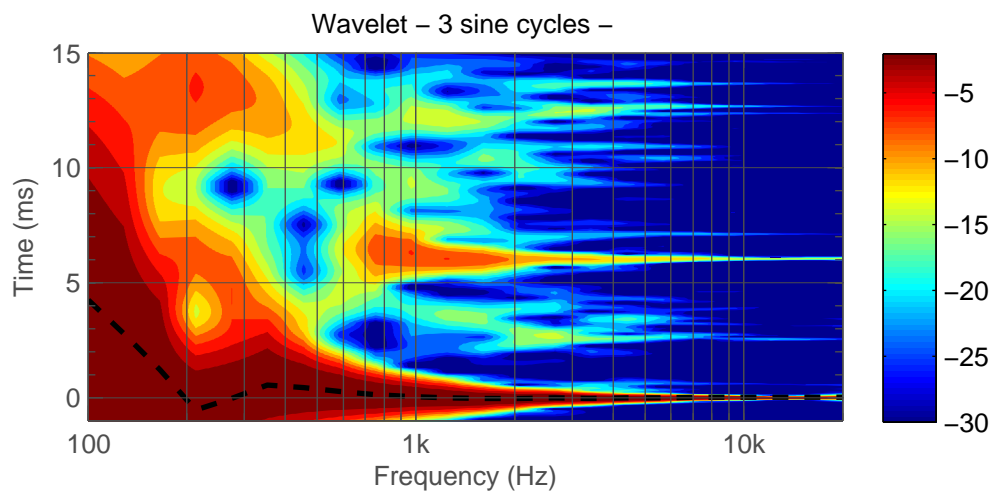
Figure 5.43: T R Mid. Wavelet.
