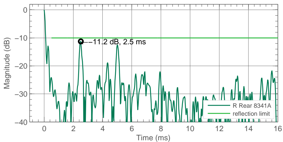
Figure 6.17: Early reflections. 1-8 kHz band. Level is relative to direct sound level.
