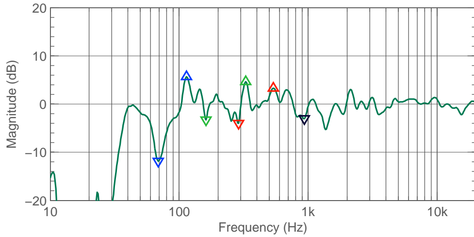
Figure 3.34: T L Front peaks and notches (before calibration).
