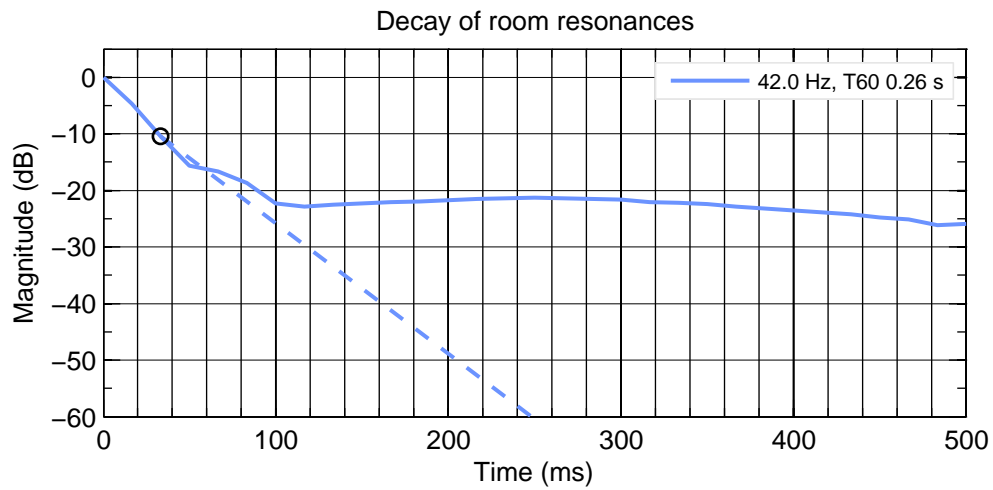
Figure 5.19: Center 8351B. Decay of detected resonances.
