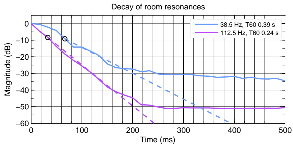
Figure 5.11: T R Mid. Decay of detected resonances.
