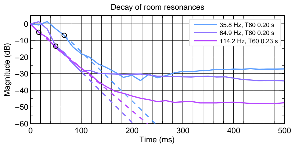
Figure 5.15: T L Rear. Decay of detected resonances.
