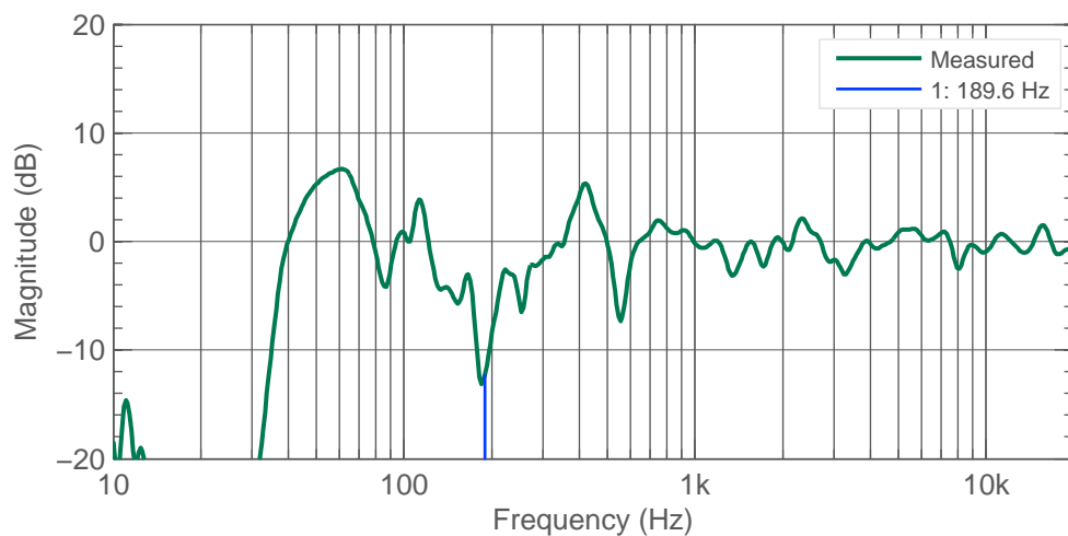
Figure 4.19: Left 8341A w. Response and lowest cancellation frequency resulting from early reflection.
