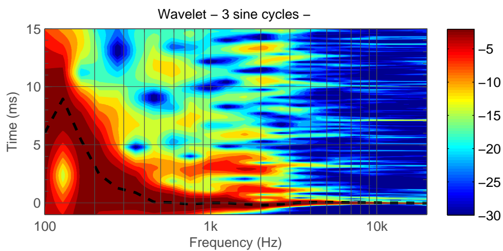
Figure 5.47: Center 8351B. Wavelet.
