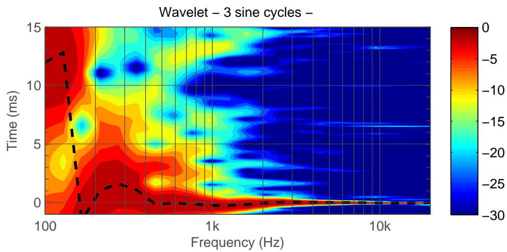
Figure 5.49: Left 8351B. Wavelet.
