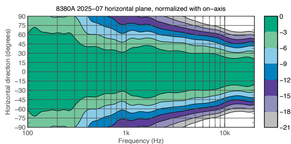
Figure 21. 8380A horizontal directivity plot.
