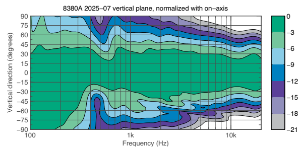
Figure 22. 8380A vertical directivity plot.
