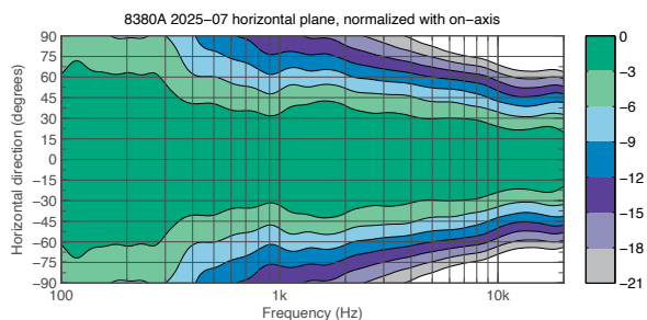
Figure 21. 8380A horizontal directivity plot.
