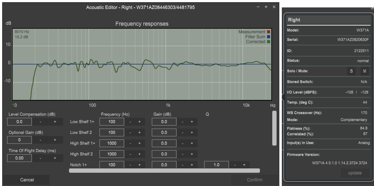
Figure 39. Acoustic editor for Woofer Systems and info on the Flatness and Correlation for Woofer Systems
