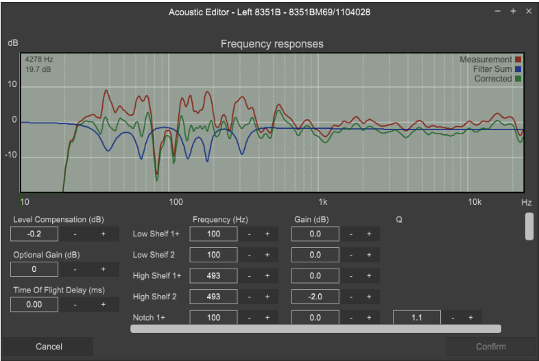
Figure 36. Example of the acoustical calibration editor window
