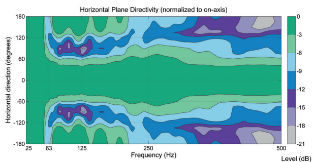
Figure 14. Horizontal directivity of W371A. Null Steering Mode - reduction side wall
