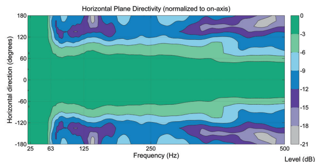
Figure 13. Horizontal directivity of W371A. Null Steering Mode - reduction back wall
