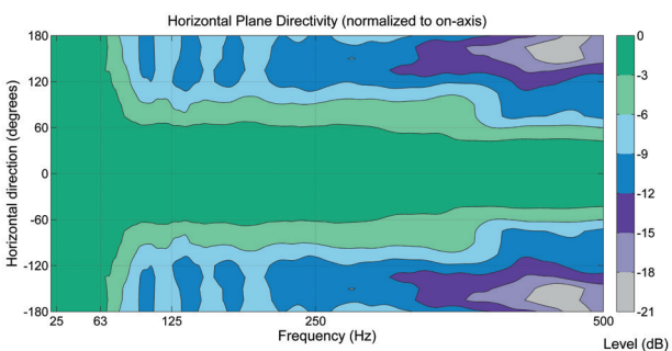
Figure 12. Horizontal directivity of W371A. Continued Directivity Mode
