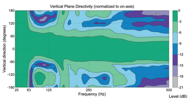
Figure 15. Vertical directivity of W371A. Null Steering Mode - reduction floor
