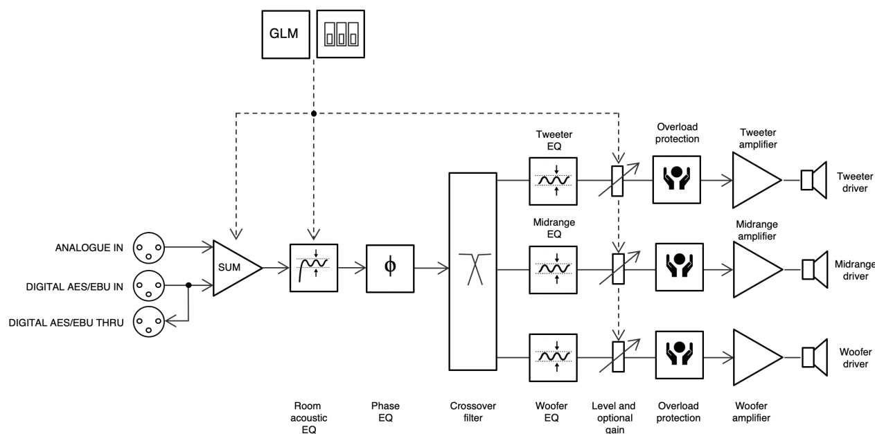
Figure 12. The signal path block diagram of the 8361A.
