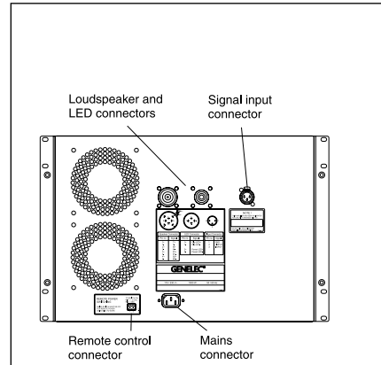
Fig 2. Amplifier unit connectors.
