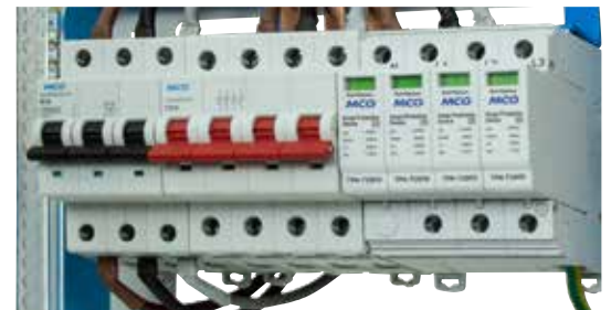
125A Incomer complete with pre-wired T2 SPD and protective MCB
