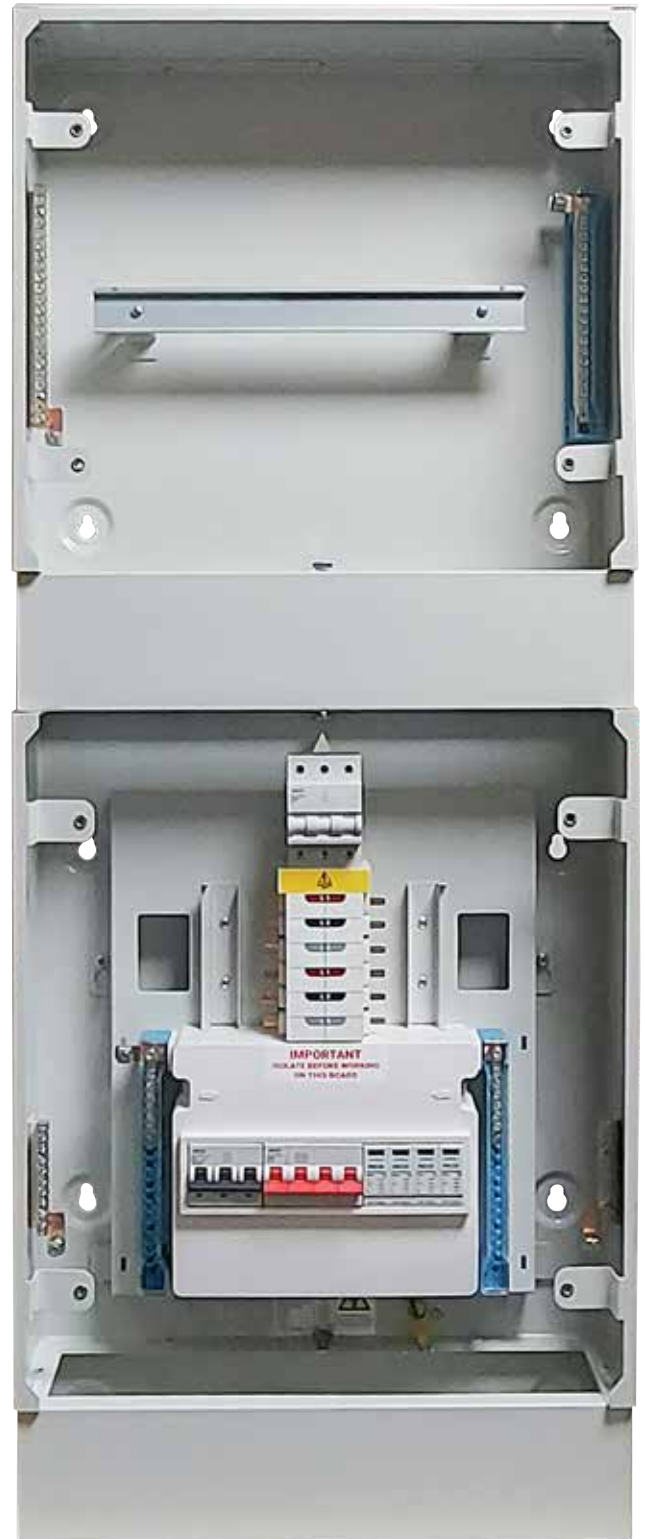
TPN4-125SPD illustration complete with Connector Block and 16-Way Extension Box
