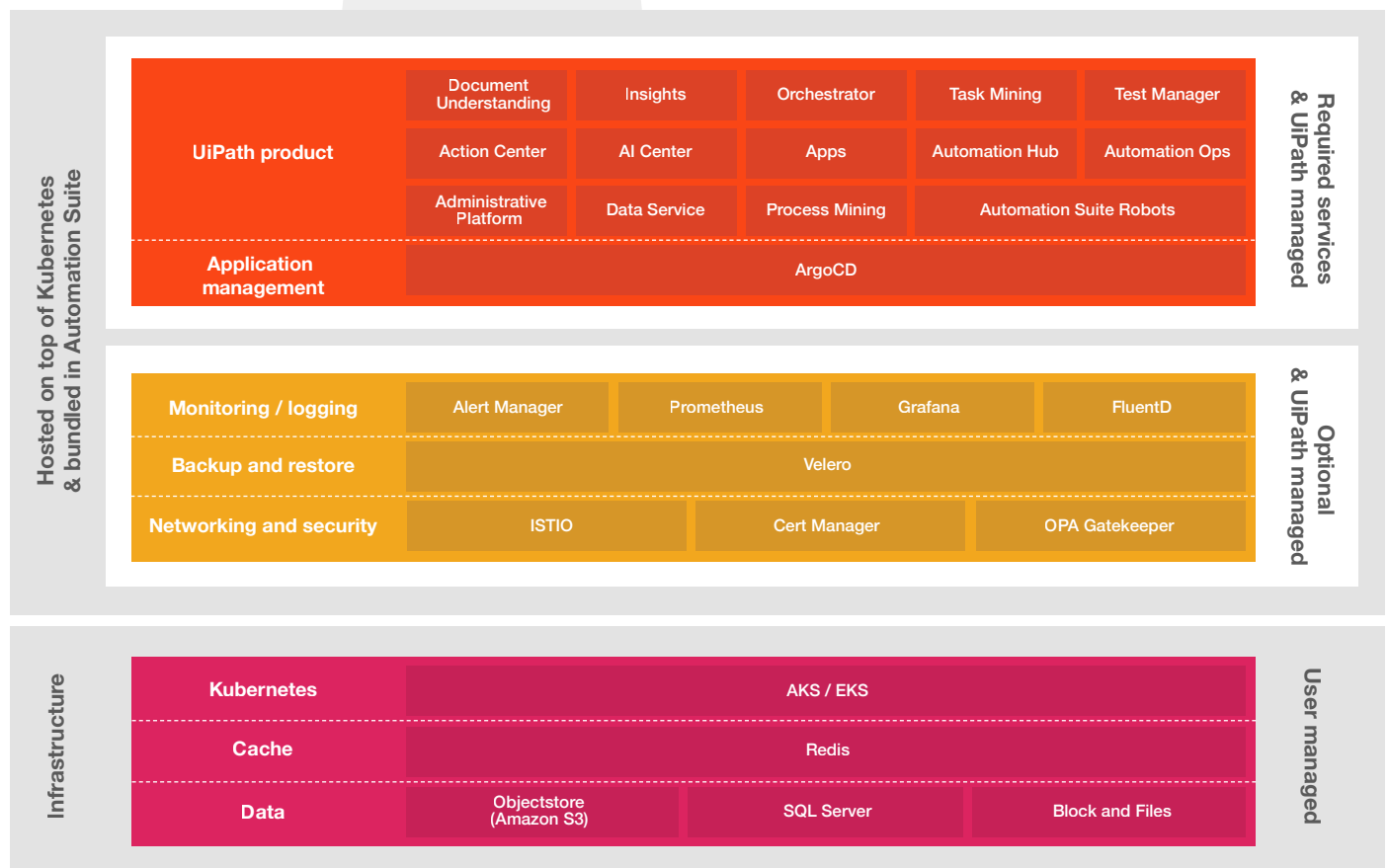
High-level architecture of Automation Suite on Amazon EKS
