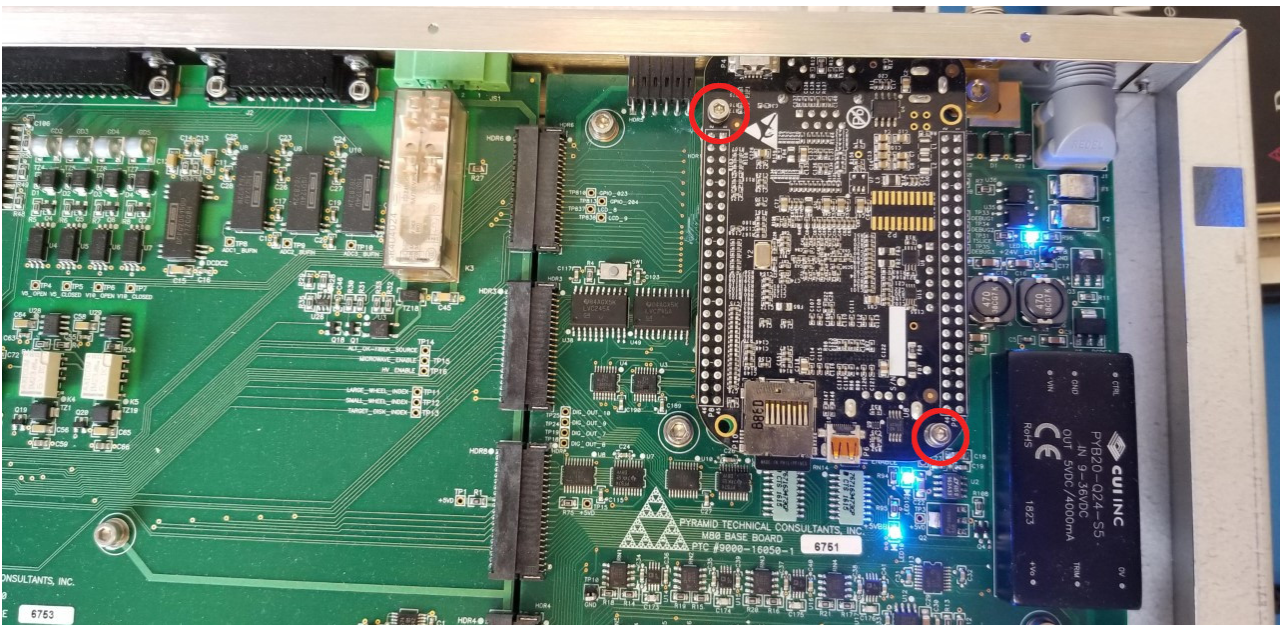
12 Mounting Screw Locations
