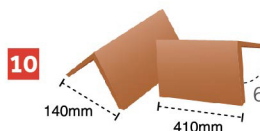
Mono-Ridge Tile (2.8pcs/metre) (Based on 50mm Lapping)
