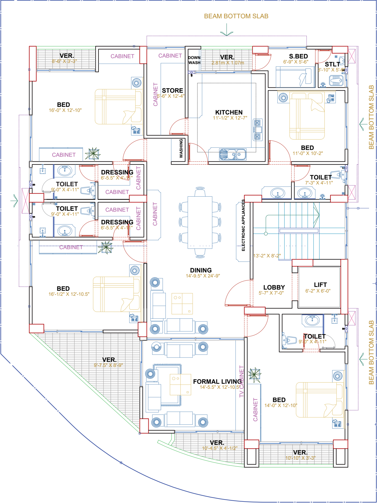
1ST,3RD,4TH & 7TH FLOOR PLAN NOT IN SCALE
