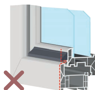
Windows with a weather profile
