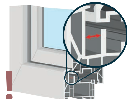
Window frames with an additional center seal
