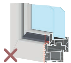
Windows with a weather profile
