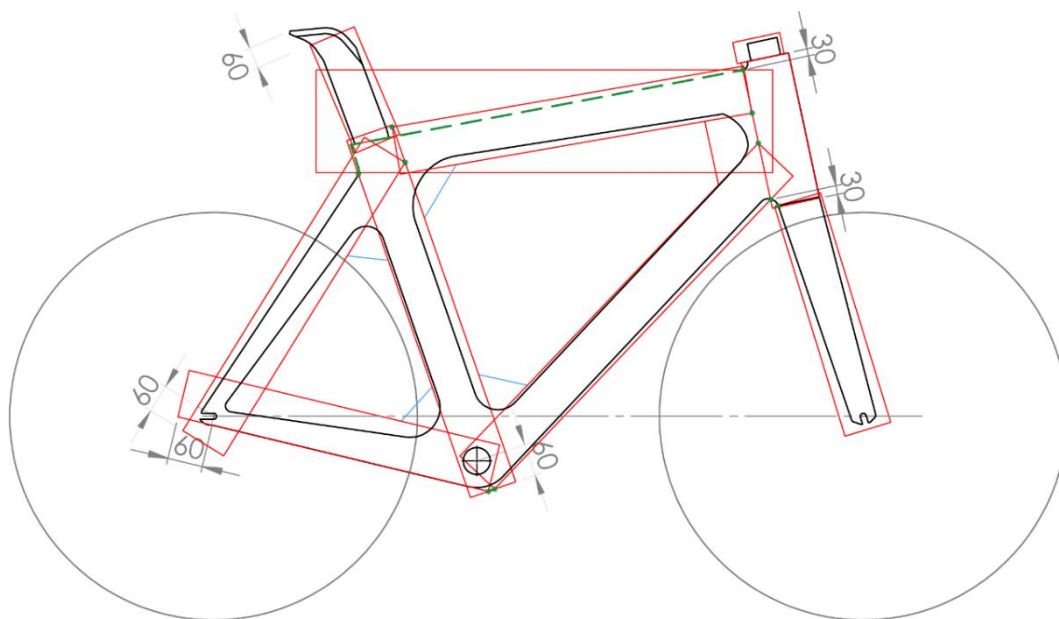
Figure 23: Illustration of the template showing the start and finish points of the 80 mm boxes for each element
