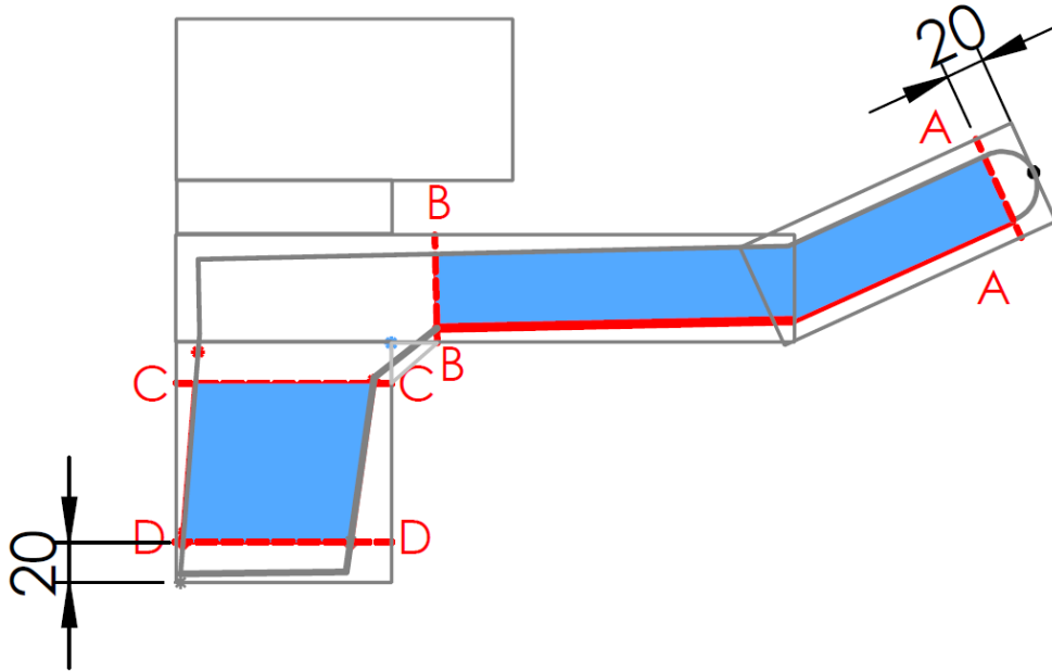
Figure 48 Illustration of minimum and maximum dimensions requirements
