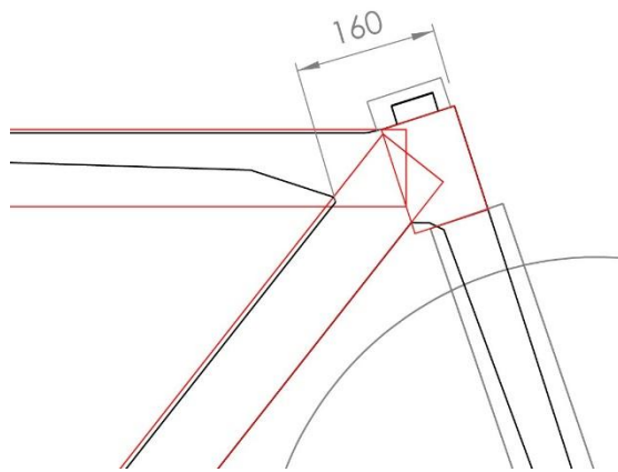
Figure 17: Illustration of the maximum distance of 160 mm for a small frame size (A)
