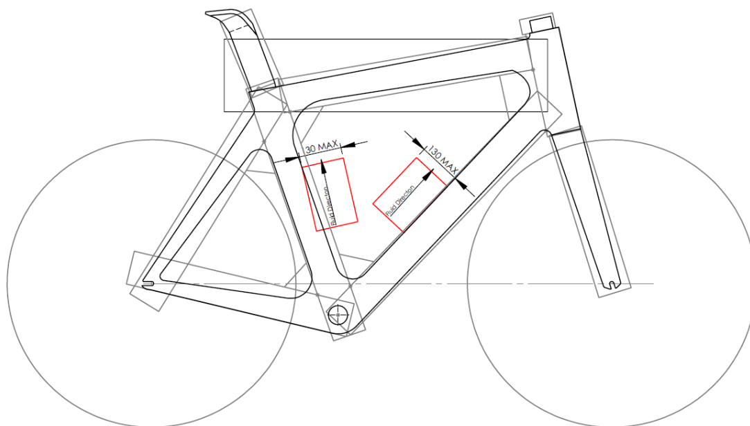
Figure 68: Illustration of the positioning of the bottle cage boxes
