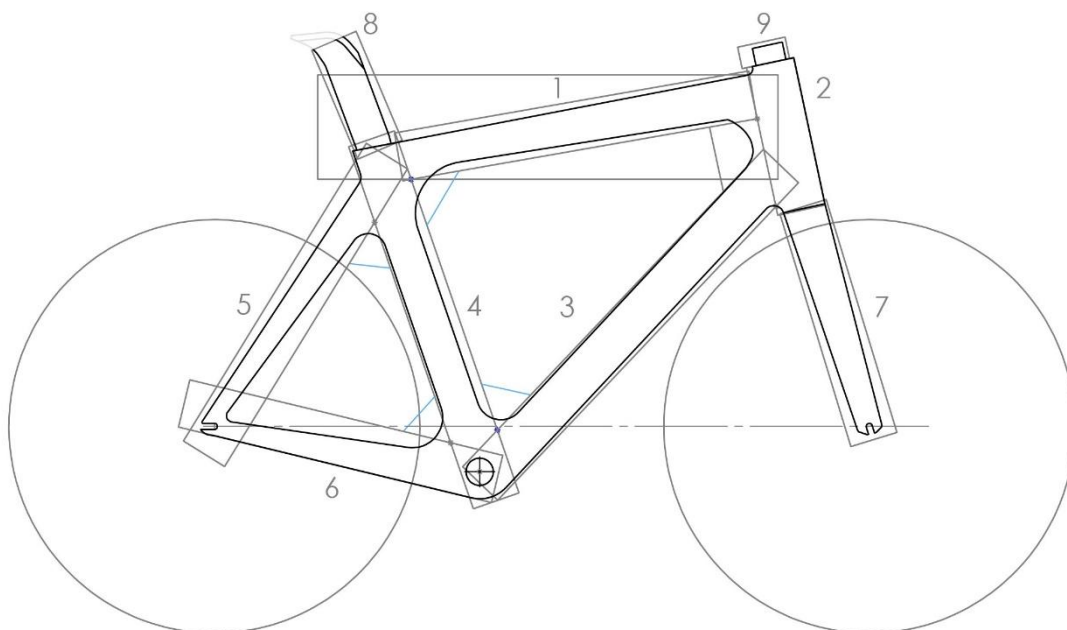
Figure 22: General illustration of the shape and positioning of the 80 mm boxes
