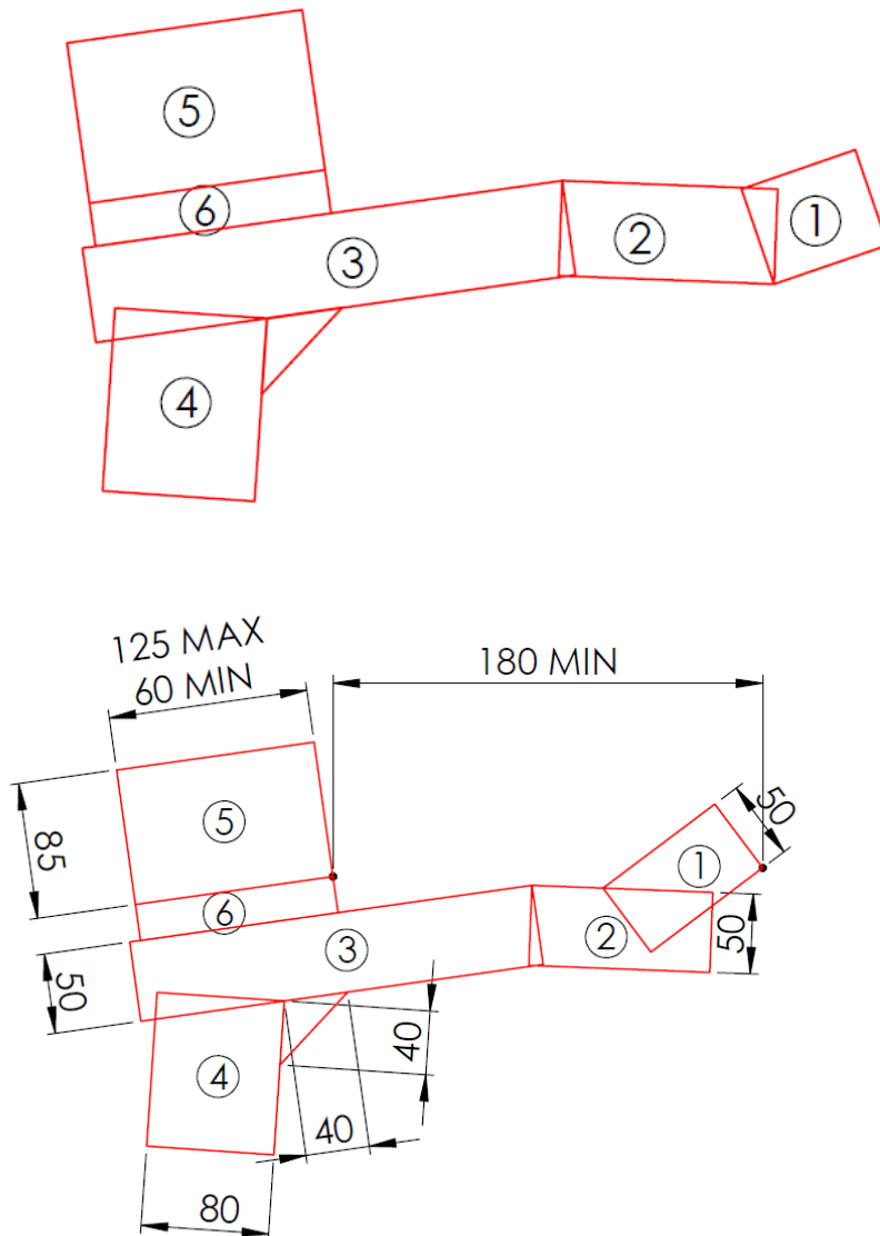
Figure 45 Illustrations (A), (B) of templates formed by red boxes for each element
