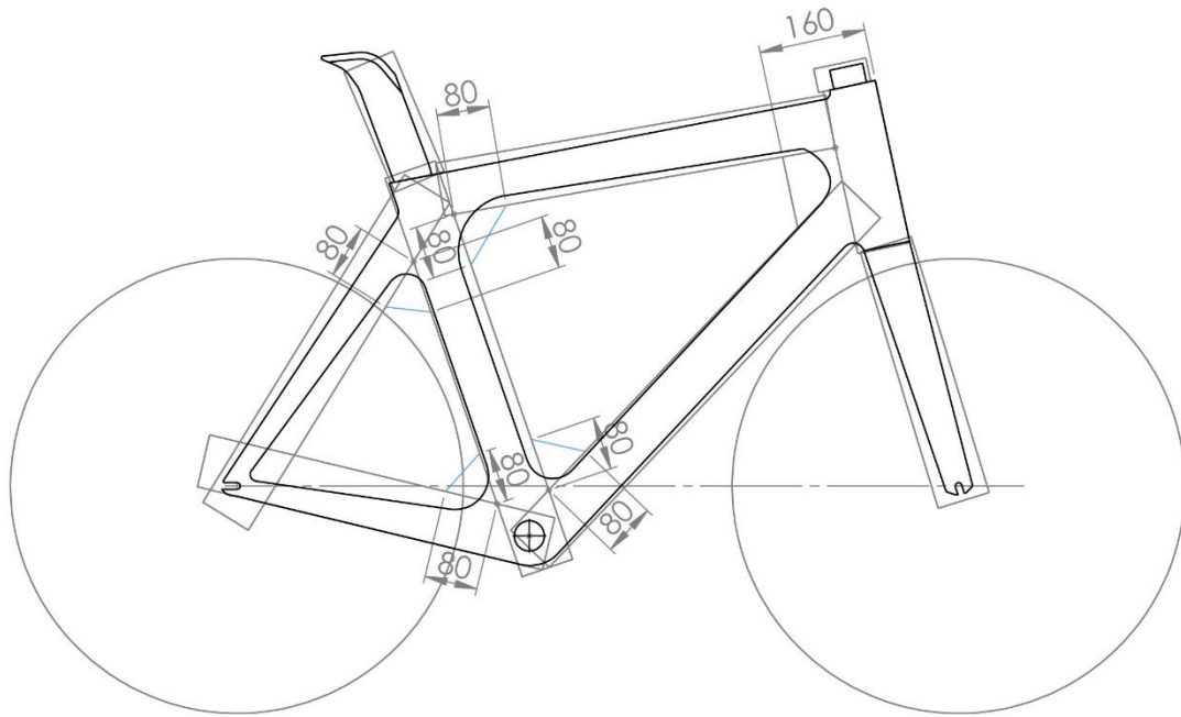
Figure 15: General illustration of compensation triangles and boxes
