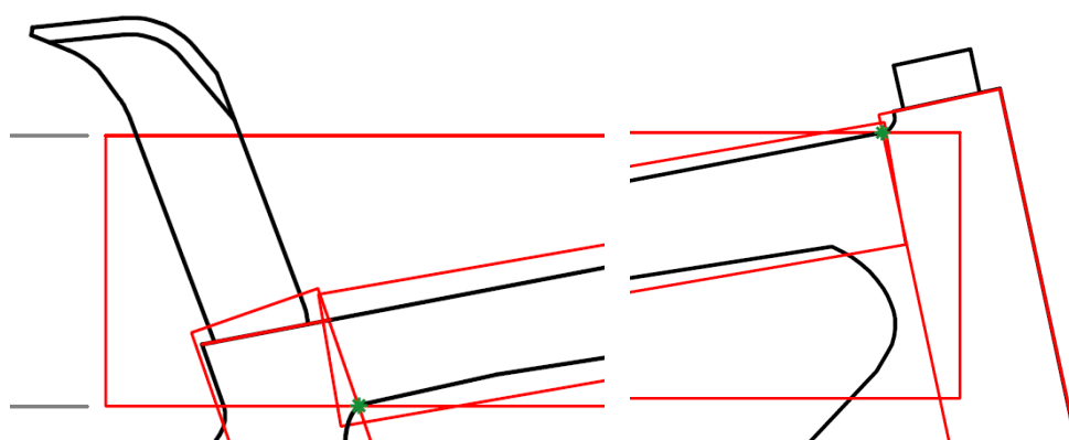
Figure 29: Highest point (circled in green) that must be contained within the 160 mm-high horizontal box
