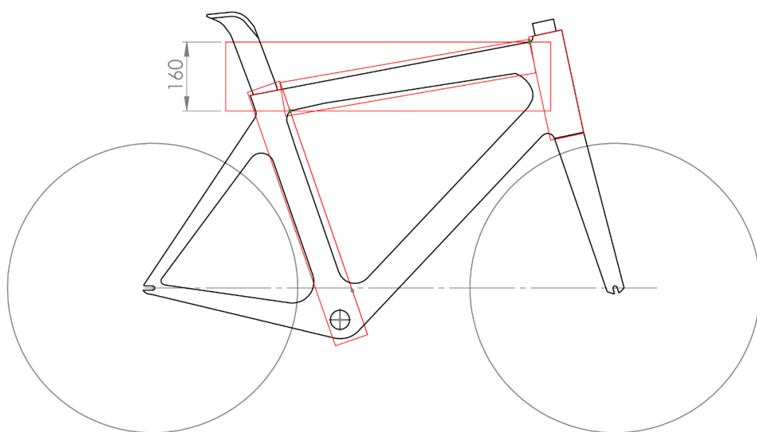
Figure 27: Illustration of maximum allowed sloping top tube
