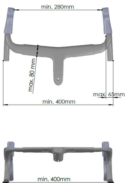
Figure 38 Road & Cyclo-cross, Illustration of the handlebar that must comply with the minimum overall width of 400 mm
