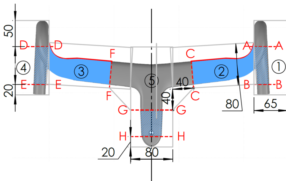
Figure 40 Road, Cyclo-cross, Illustration of minimum and maximum dimensions requirements
