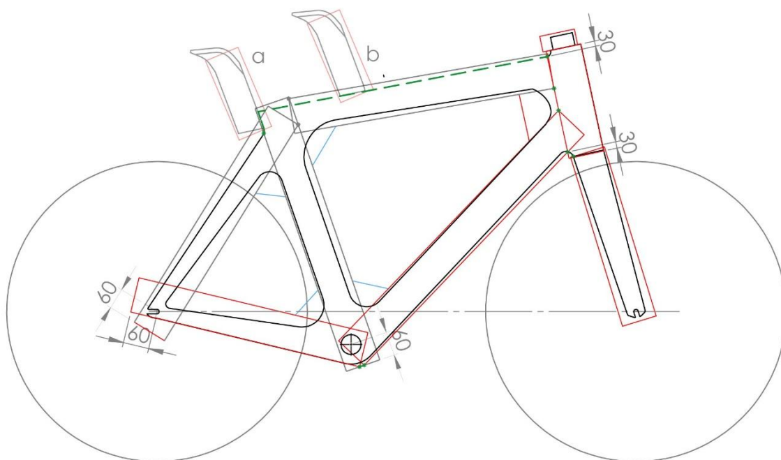
Figure 24: Illustration of the positioning of the seat post box
