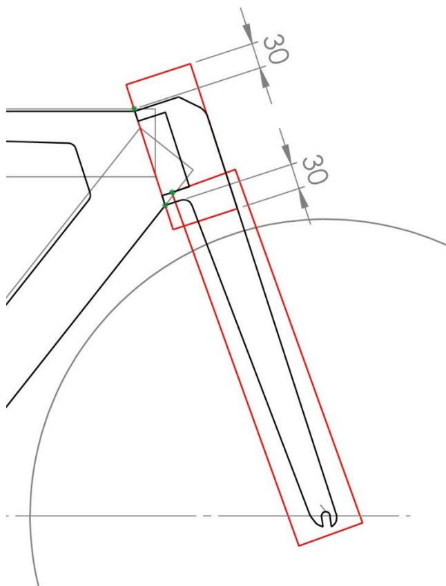
Figure 33: Illustration of the position of the boxes for offset fork
