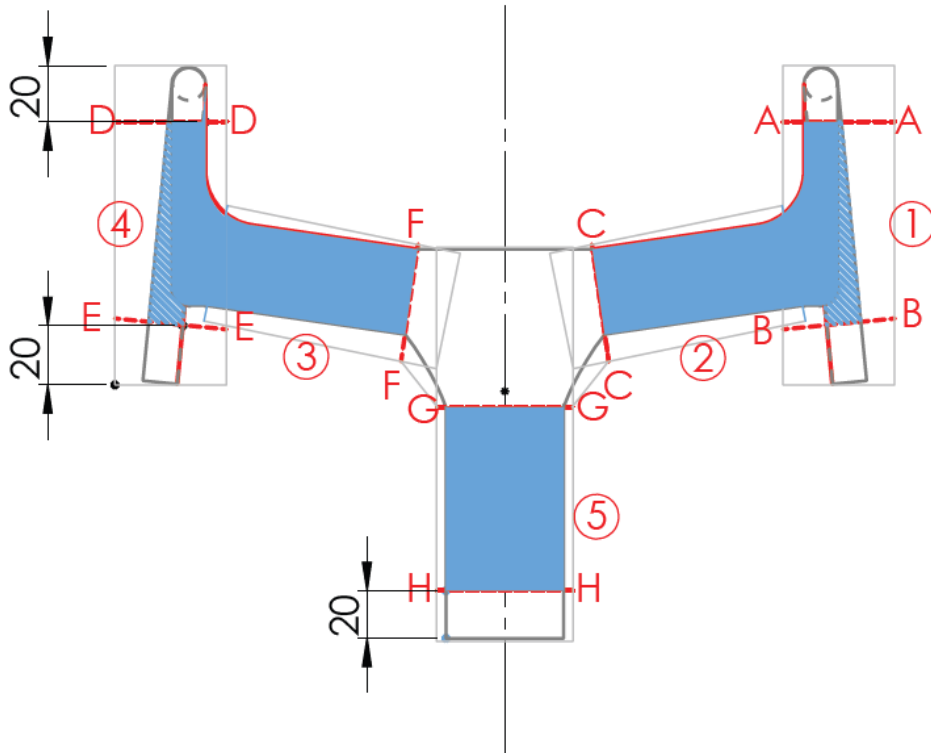
Figure 41 Track, Illustration of minimum and maximum dimensions requirements
