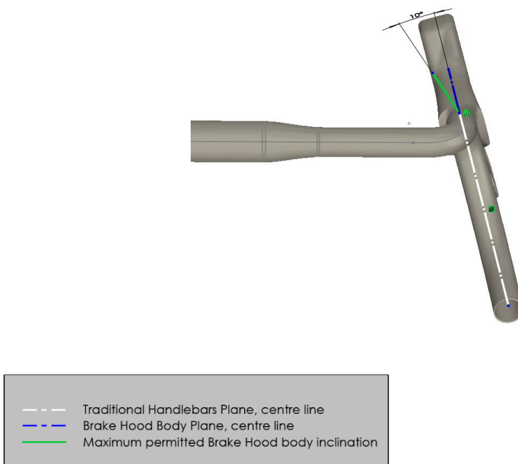
Figure 37 Illustration of the maximum permitted Brake Hood body inclination in combination with a flared traditional handlebars
