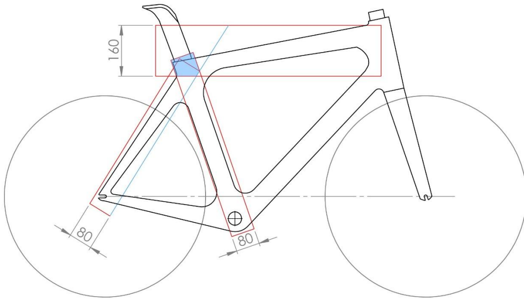
Figure 30: Illustration of the rule on the inclination of seat stays
