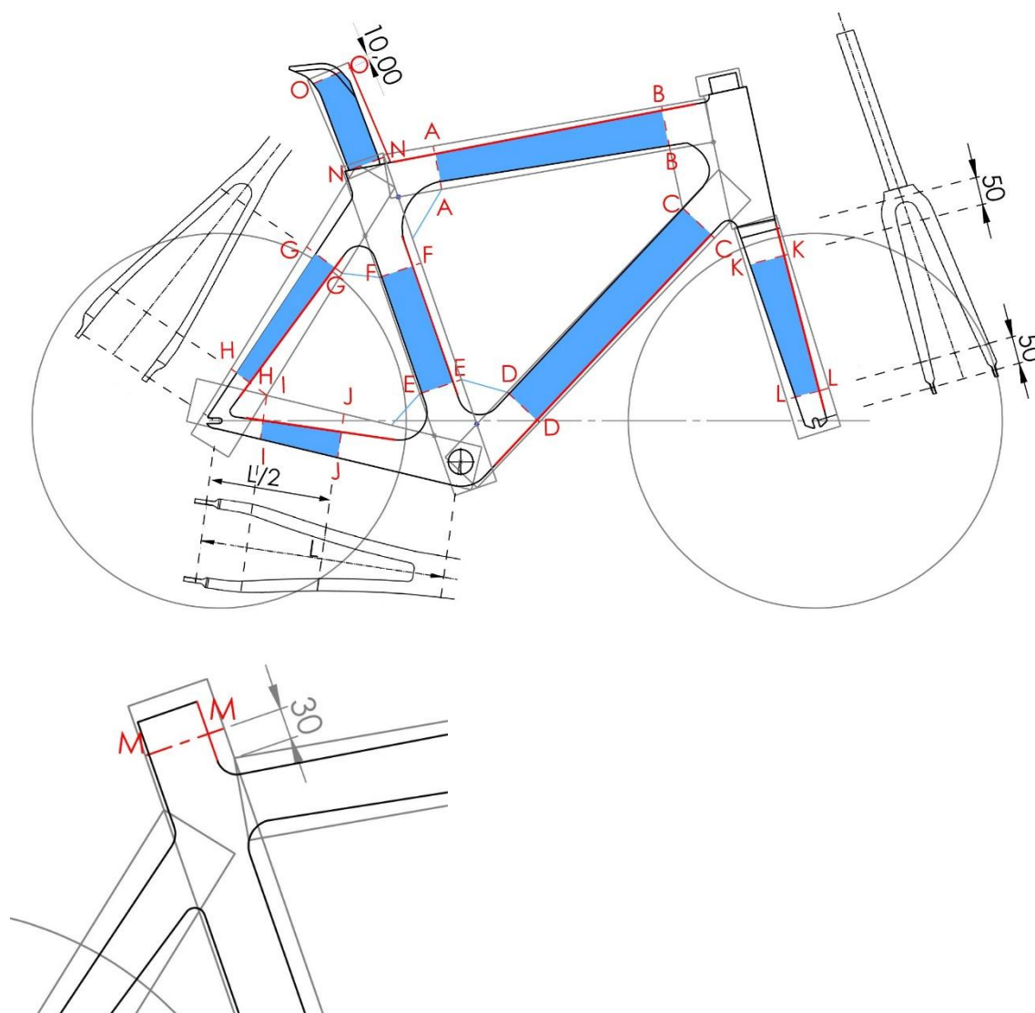
Figure 26: Illustrations of the areas of the frameset subject to the rule of minimum and maximum dimension
