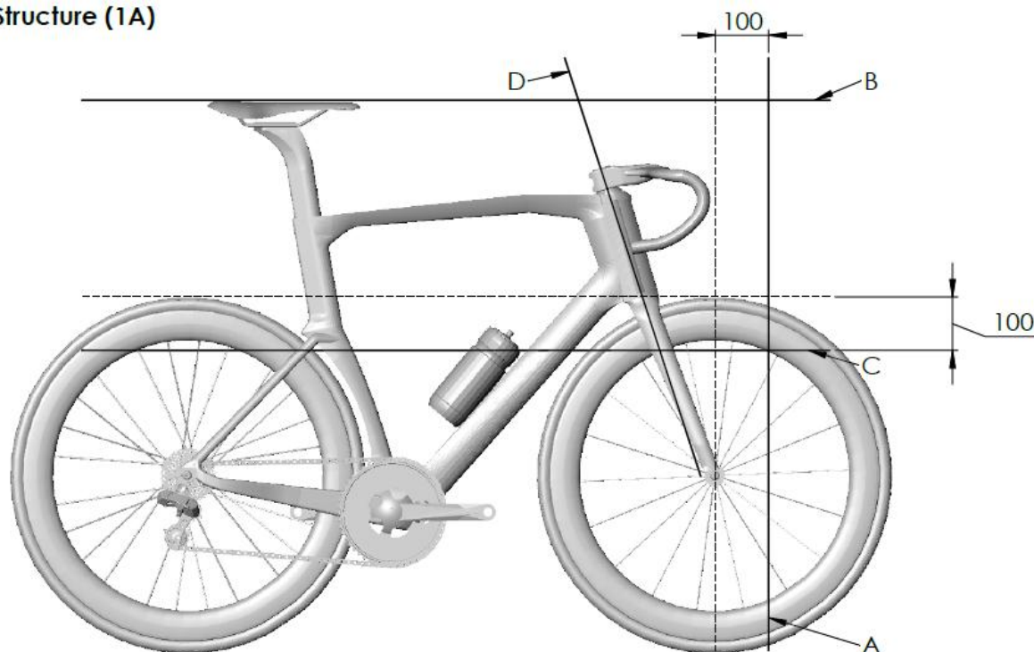
Figure 35: Illustration of the box, marked out by lines A, B, C and D, within which the handlebars must be fully contained.
