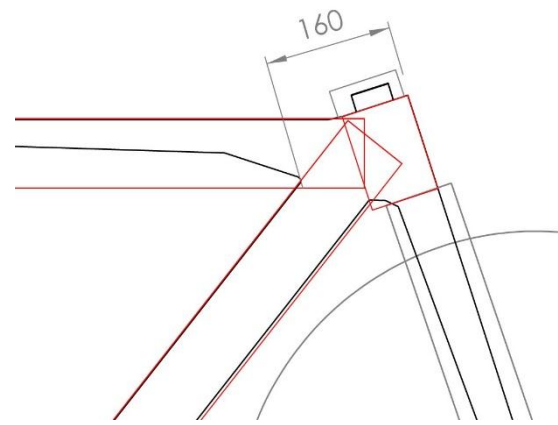
Figure 18: Illustration of the maximum distance of 160 mm for a small frame size (B)
