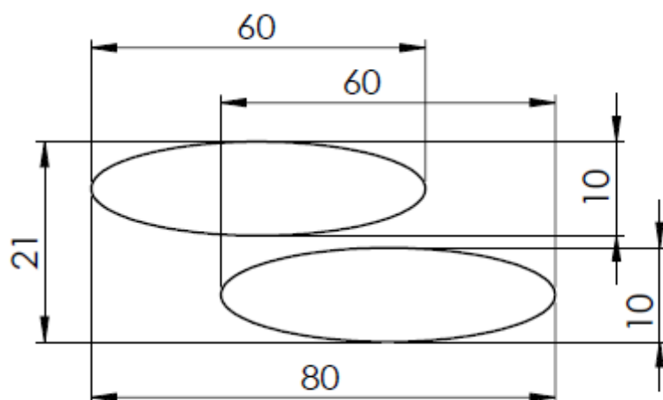
Figure 49: Example of a compliant section of an element formed by two tubes
