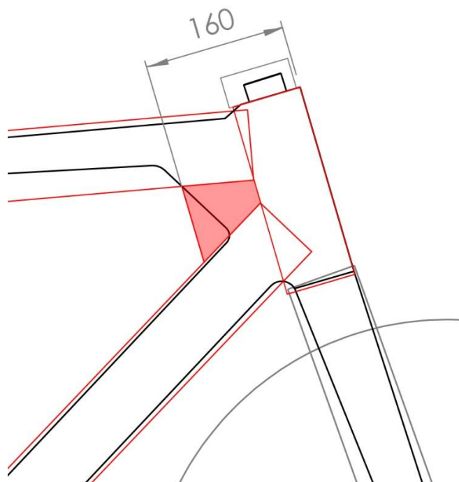
Figure 20: Illustration of the compensatory joint zone
