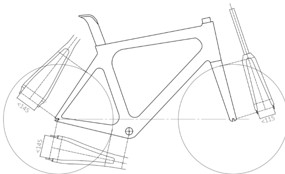
Figure 10: Road and Cyclo-cross - Illustration of the maximum distances between the internal extremities of the two legs of the front forks and the two sides of the rear triangle
