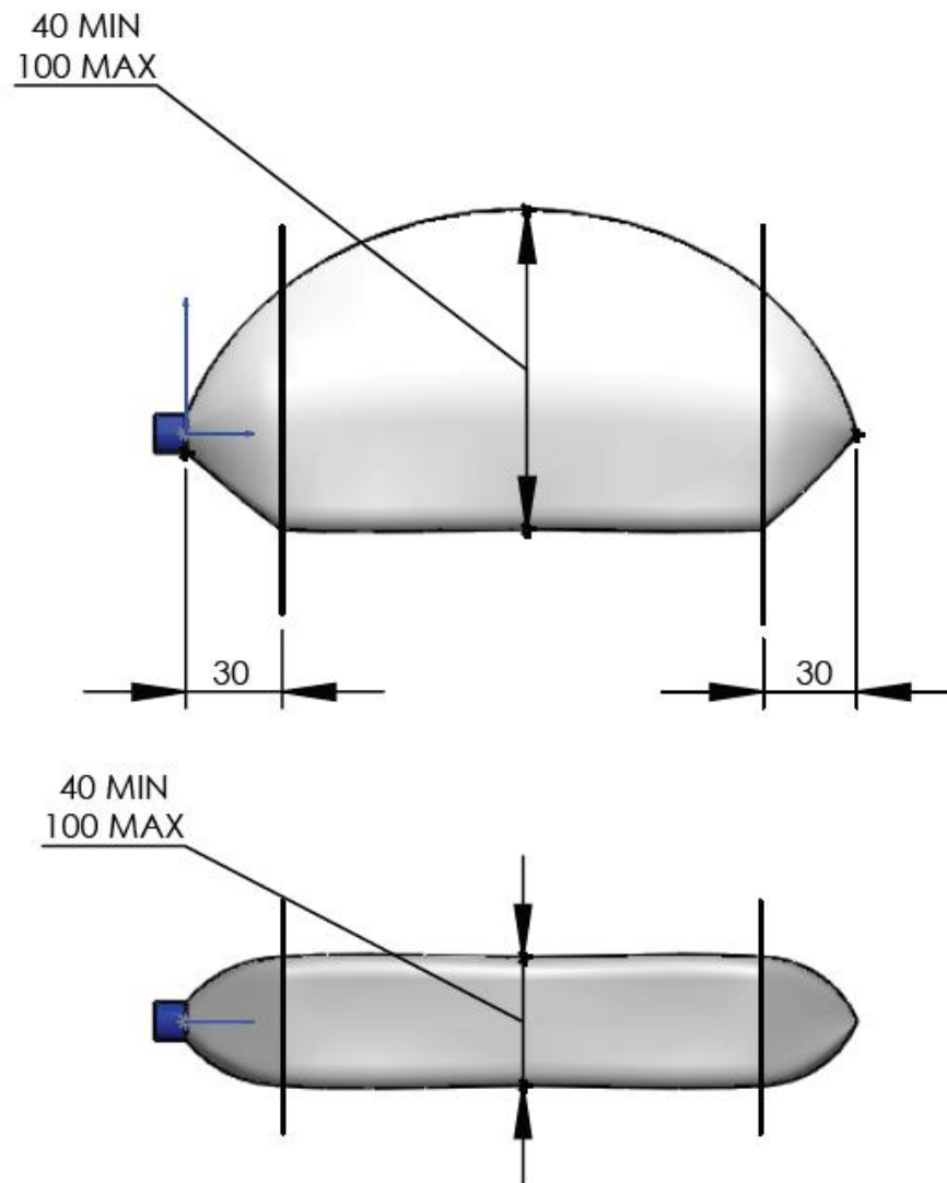
Figure 67: Illustration of the areas of a bottle where the dimensions are subject to regulations
