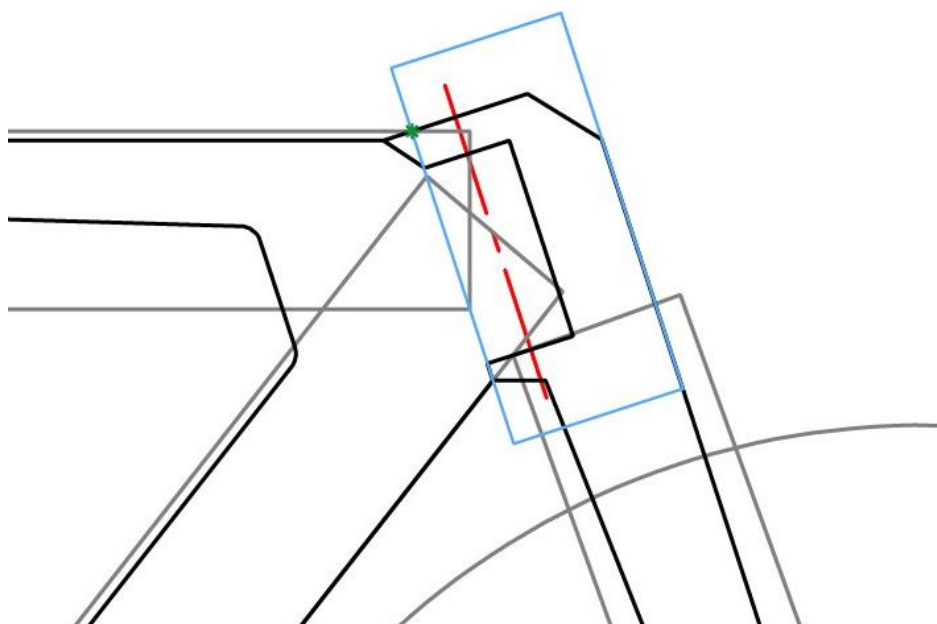
Figure 32: Illustration of the positioning of the axis of the head tube within the head tube box
