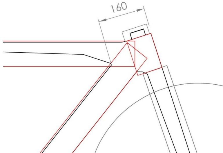
Figure 16: Illustration of the 160 mm rule
