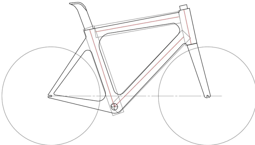
Figure 21: Illustration of the start and finish points of the straight lines required inside tubes
