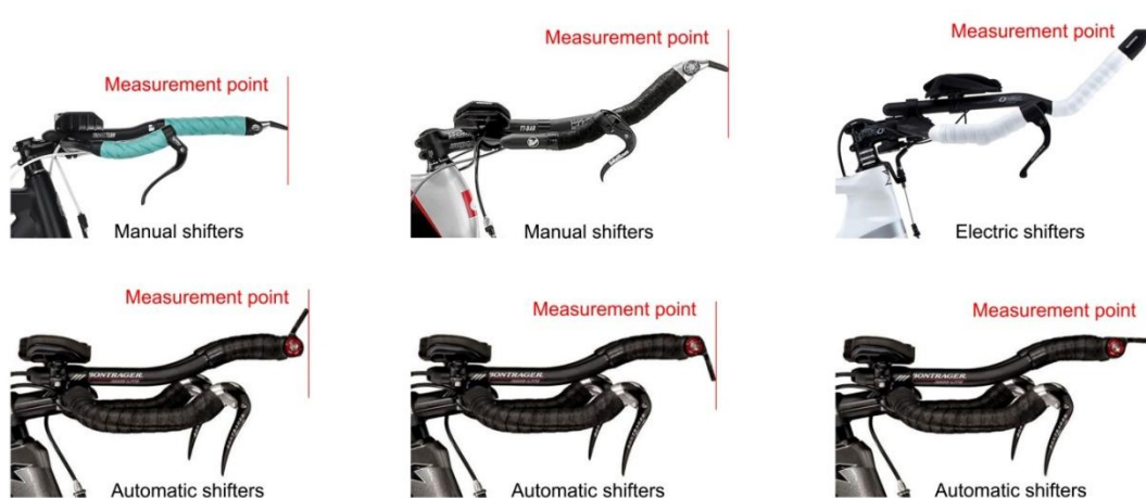
Figure 55 Points of measurement for the horizontal distance from the bottom bracket axle
