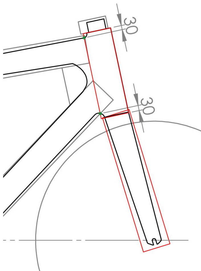
Figure 31: Illustration of the position of the boxes for a fork using a traditional internal steerer
