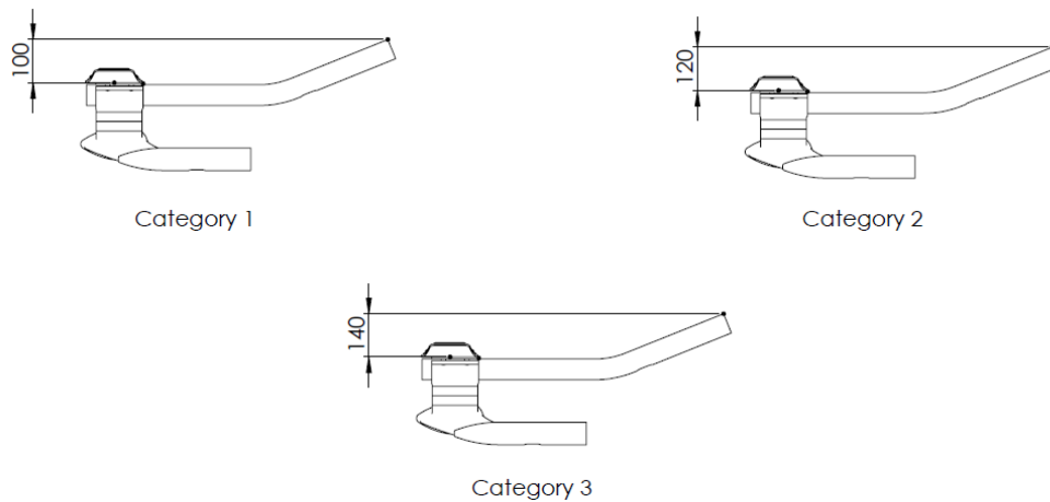
Figure 52 Examples of the vertical limits per each height category (as per provisions of article 1.3.023)
