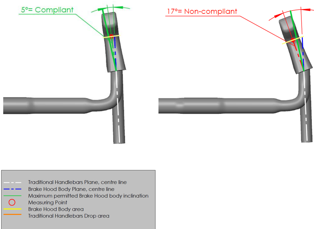
Figure 36: Illustration of the maximum permitted Brake Hood body inclination
