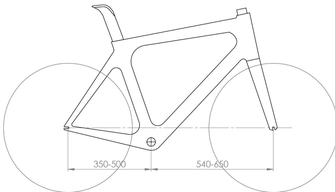
Figure 9: Illustration of the minimum and maximum distances between the bottom bracket and front and rear wheel axles
