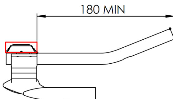
Figure 47 Illustration of the Forearm support box position
