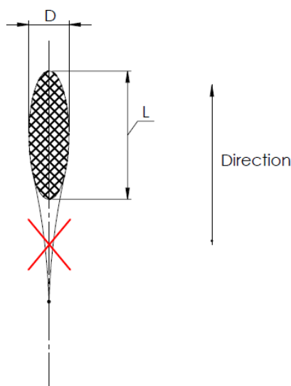
Figure 63: Illustration of the restriction around the fuselage form of elements
