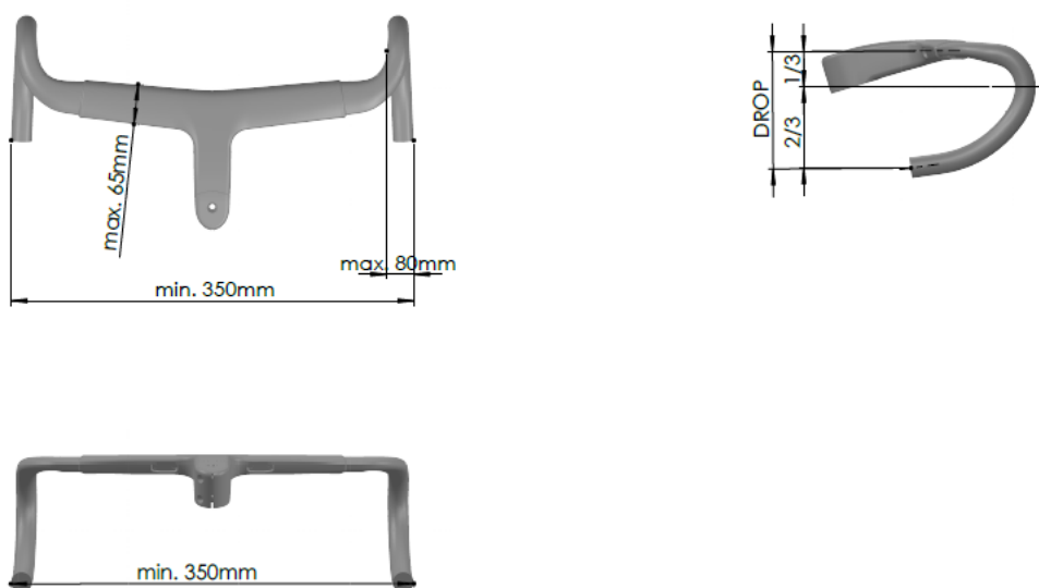
Figure 38 Illustration of the handle area that must comply with the minimum overall width of 350 mm
