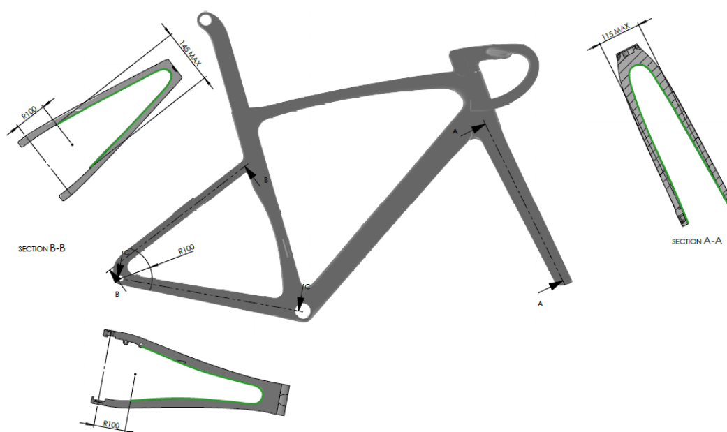
Figure 9: Road, Cyclo-cross - Illustration of the maximum distances between the internal extremities of the two legs of the front forks and the two sides of the rear triangle
