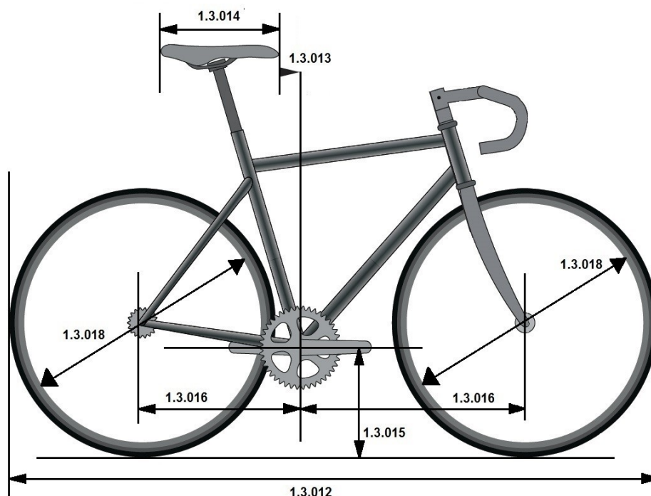
Figure 6: Illustration of the parts of the bicycle covered by Articles 1.3.011 to 1.3.025
