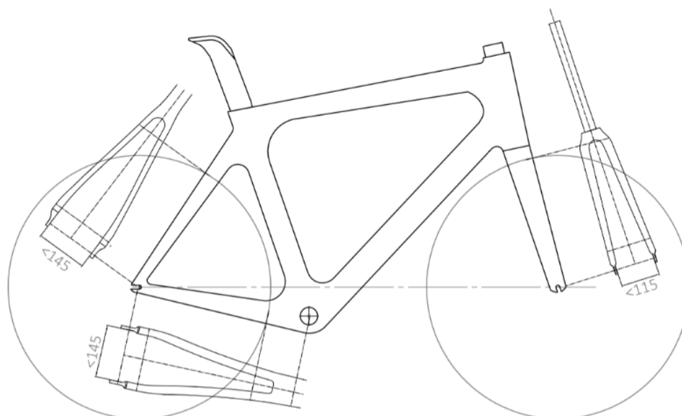
Figure 10: Track - Illustration of the maximum distances between the fork drop-outs and rear drop-outs
