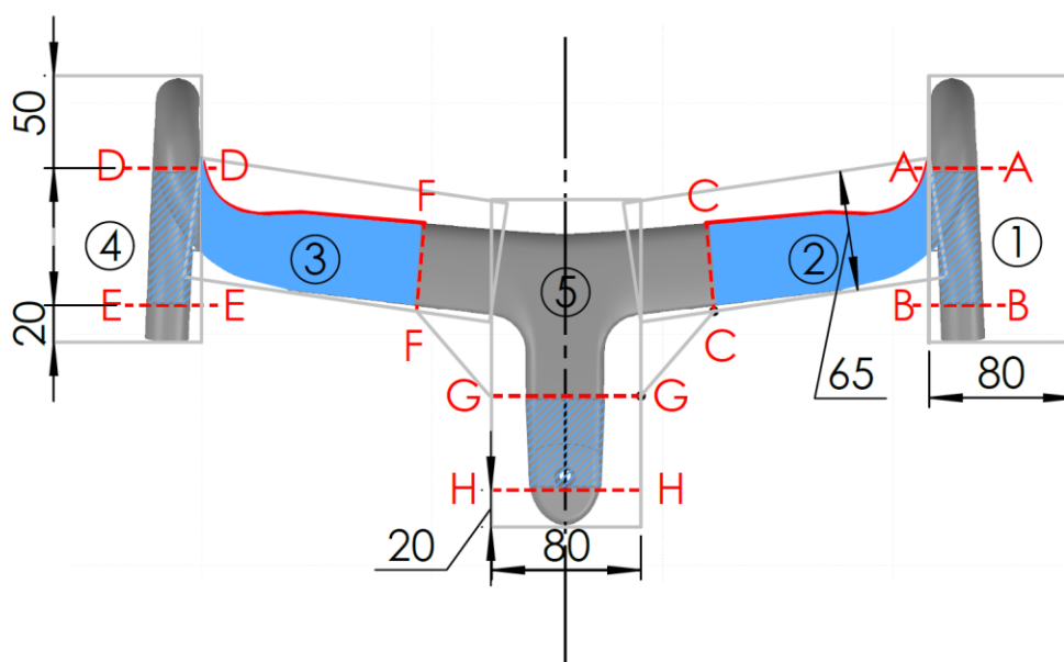
Figure 41 Track, Illustration of minimum and maximum dimensions requirements
