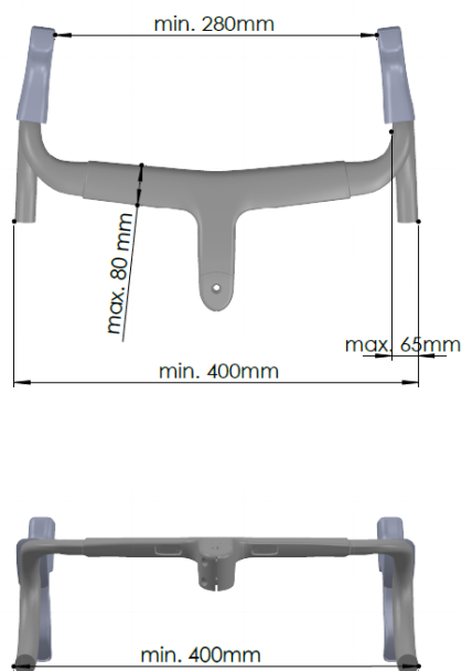
Figure 37 Illustration of the handlebar that must comply with the minimum overall width of 400 mm
