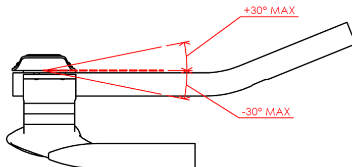
Figure 54 Illustration of the maximum inclination of each elbow rest
