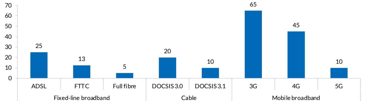
Typical telecoms access technology latency (ms)
