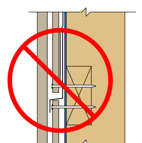
Do Not Span Batten over Horizontal Panel Seam
