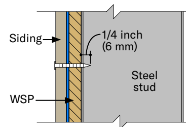
Siding nailed to WSP Sheathing
