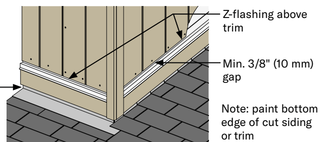
Siding with Trim
