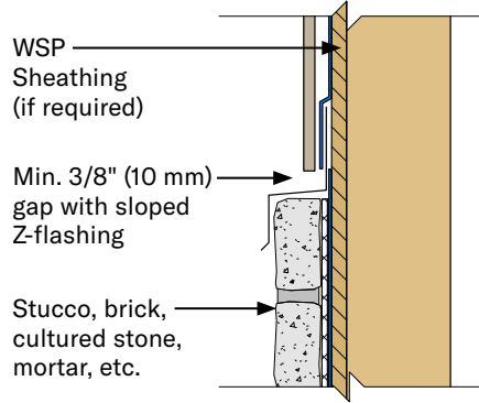
Section View
