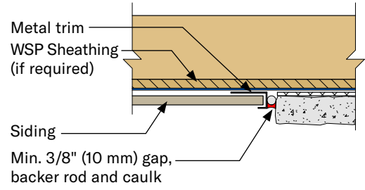
Plan View - Metal Trim
