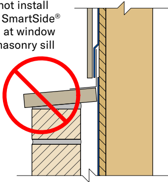
Section View
