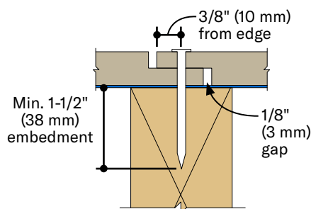
Single nailing option Figure 4e
