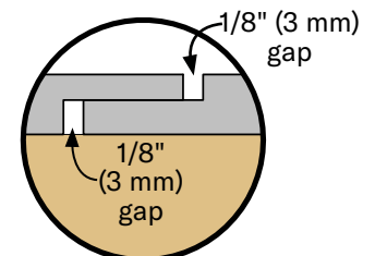
Shiplap Edge without Alignment Bead Figure 2b
