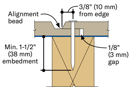
Single nailing option Figure 4d
