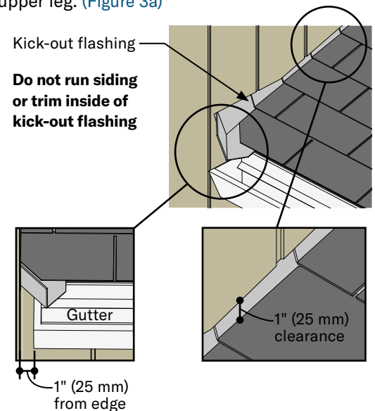
Kick-out Flashing Figure 3c
