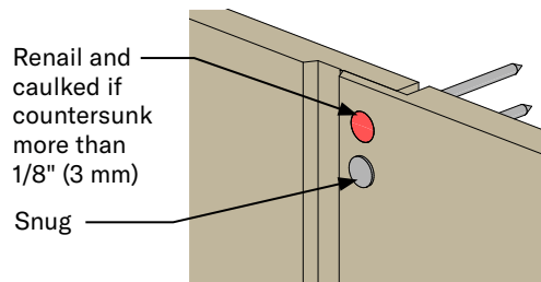
Figure 5b FACE NAILED CONDITION
