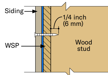
Siding nailed to WSP Sheathing
