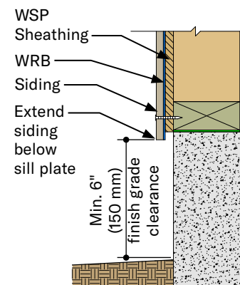
WSP Sheathing Attachment
