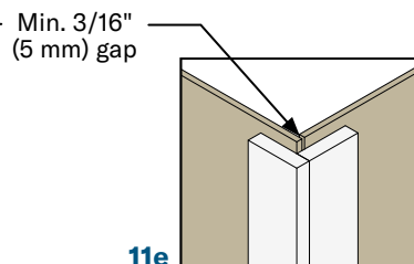
OUTSIDE CORNER PREFERRED
