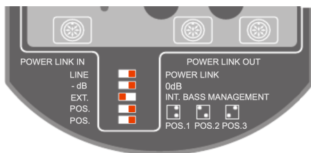
Figure 10.2: The recommended settings of the Beolab 11 when used with the Beosound Theatre are shown in red.
