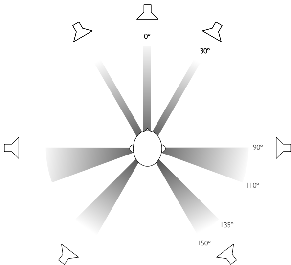
Figure 12.3: Recommended loudspeaker configuration for most 7.x channel audio signals. The actual angles of the loudspeakers shows the reference placement used at Bang & Olufsen for testing and tuning.
