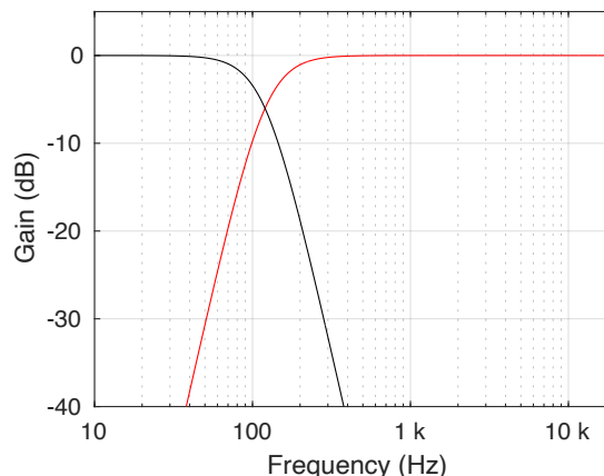
Figure 4.1: Gain response of the crossover used in the Bass Management system, showing an example with the factory-default crossover frequency of 120 Hz.
