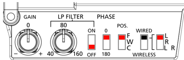
Figure 10.4: The recommended settings of the Beolab 19 when used with the Beosound Theatre are shown in red. This diagram assumes that the subwoofer is connected using a Wired Power Link and that you are using the Left channel of that connection; this may not be the case in your setup.
