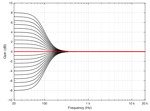
Figure 6.2: Frequency response measurements of all settings of the Bass control. Note that this response is applied to all input channels.
