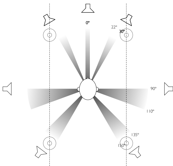
Figure 12.4: Loudspeaker positions associated with the speaker roles available in the Theatre, showing a full 7.x.4 configuration.
