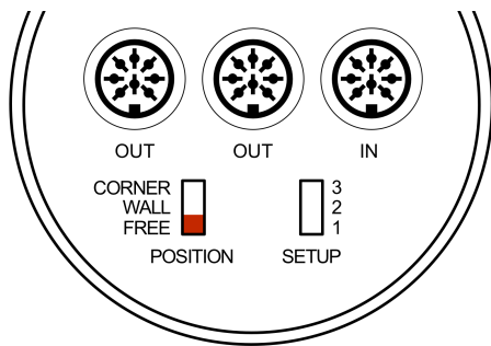
Figure 10.1: The recommended settings of the Beolab 2 when used with the Beosound Theatre are shown in red. Additional Beolab loudspeakers should be connected directly to the Beosound Theatre instead of to the Beolab 2’s outputs.
